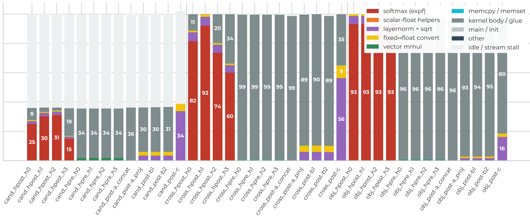
AIE per-tile time breakdown — head_post tiles saturated by scalar softmax
