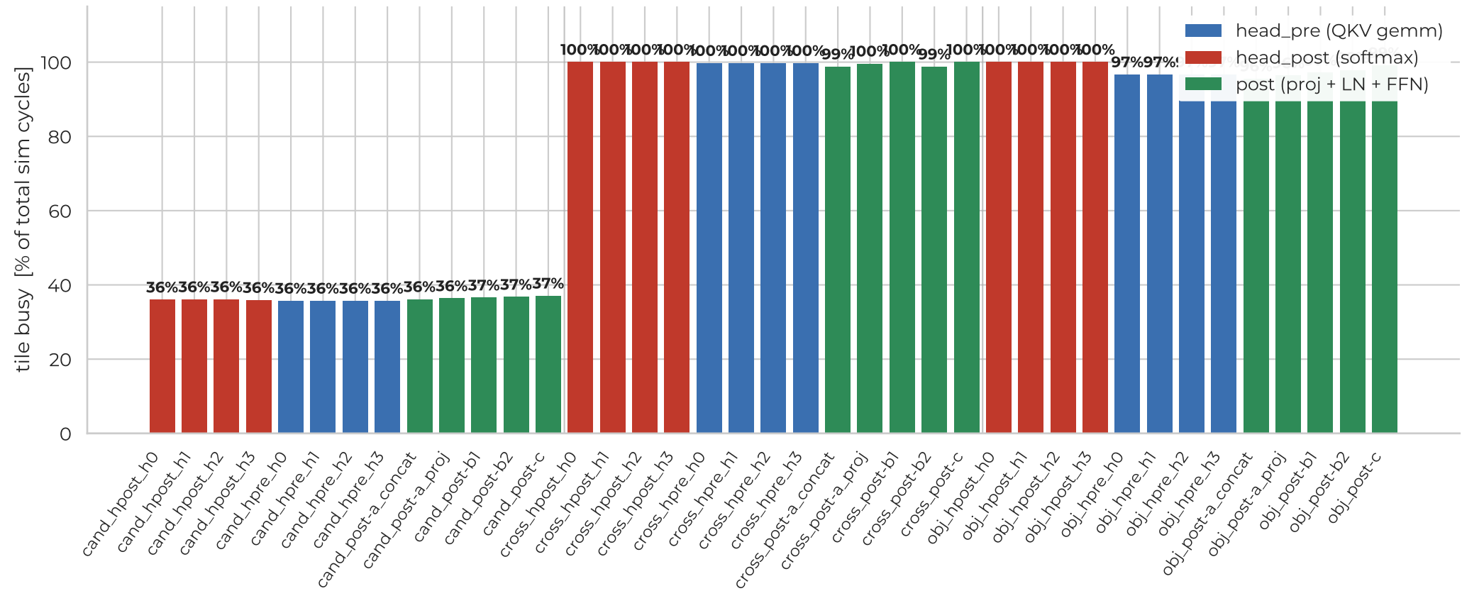
AIE per-tile utilization — obj head_post tiles are pipeline-saturating
