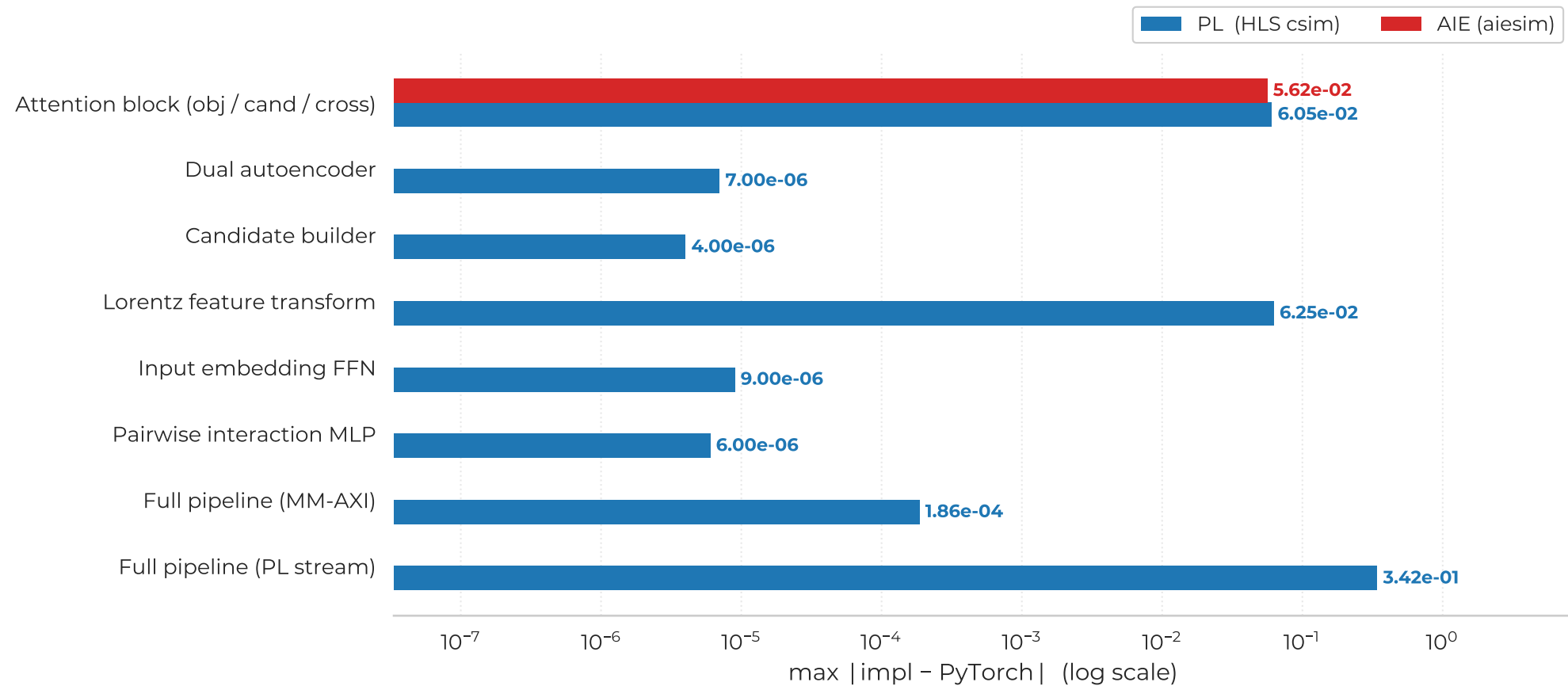
Numerical accuracy per algorithm component — HLS csim & AIE aiesim
