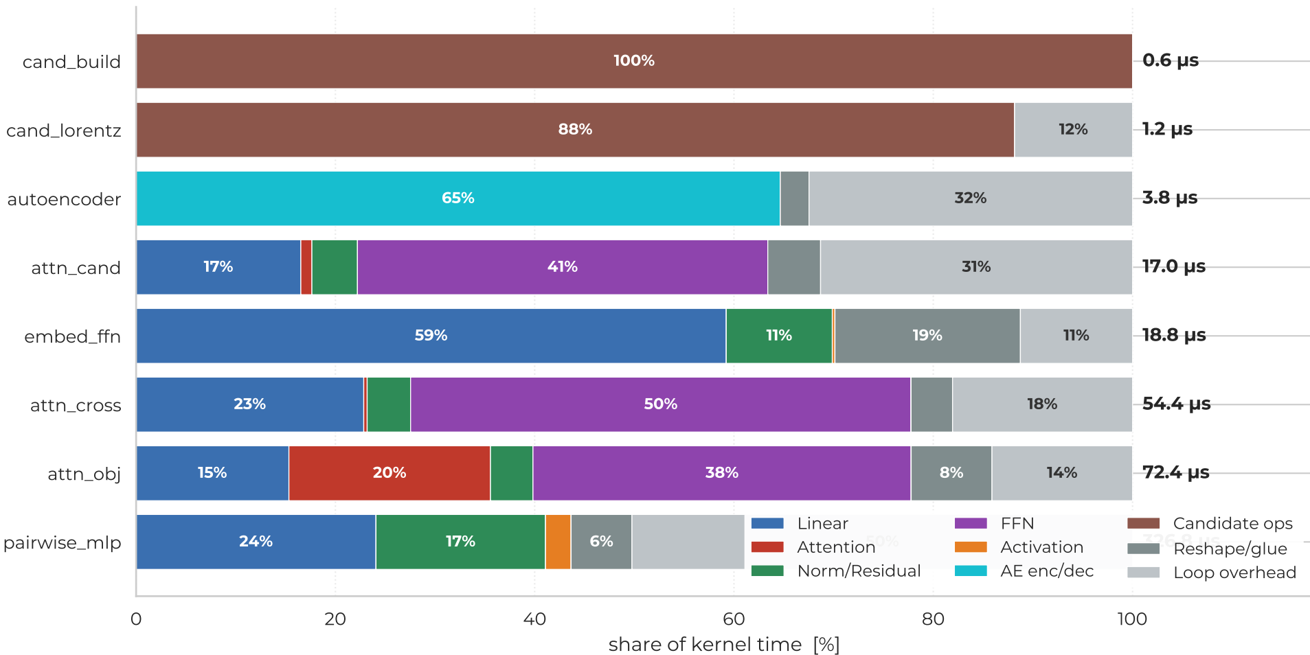
PL kernel per-stage breakdown — normalized (csynth estimates)
