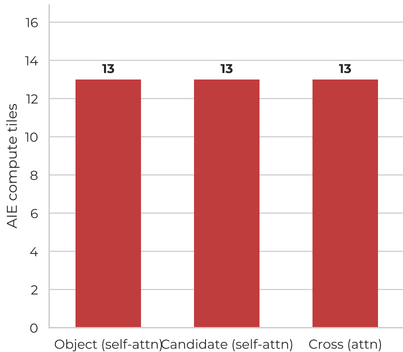
AIE tile usage (39/400 = 9.8% of array)
