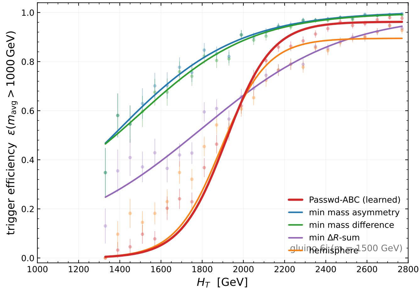
(a) SIGNAL — mass trigger turns on
