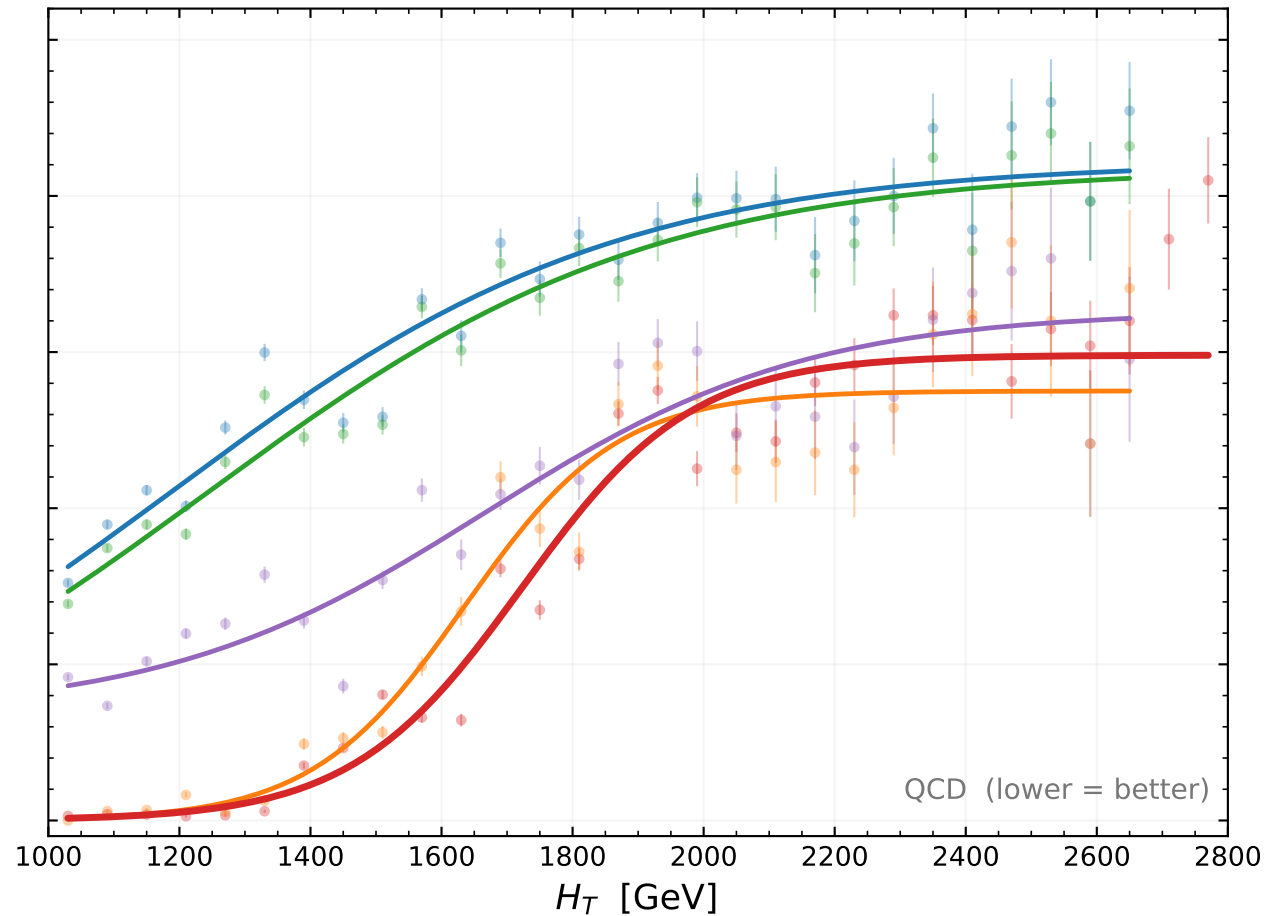
(b) BACKGROUND — a good assignment keeps it OFF
