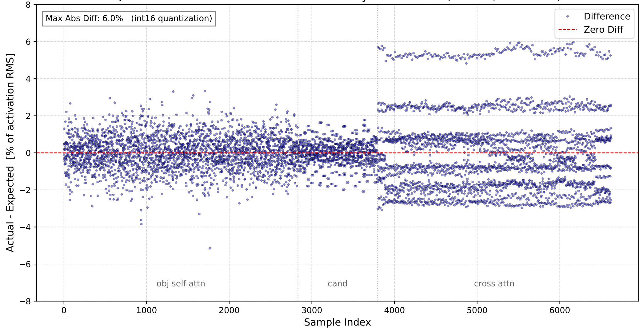
Quantization Error: AIE int16 Attention vs PyTorch float32 (x86sim, 20 events)
