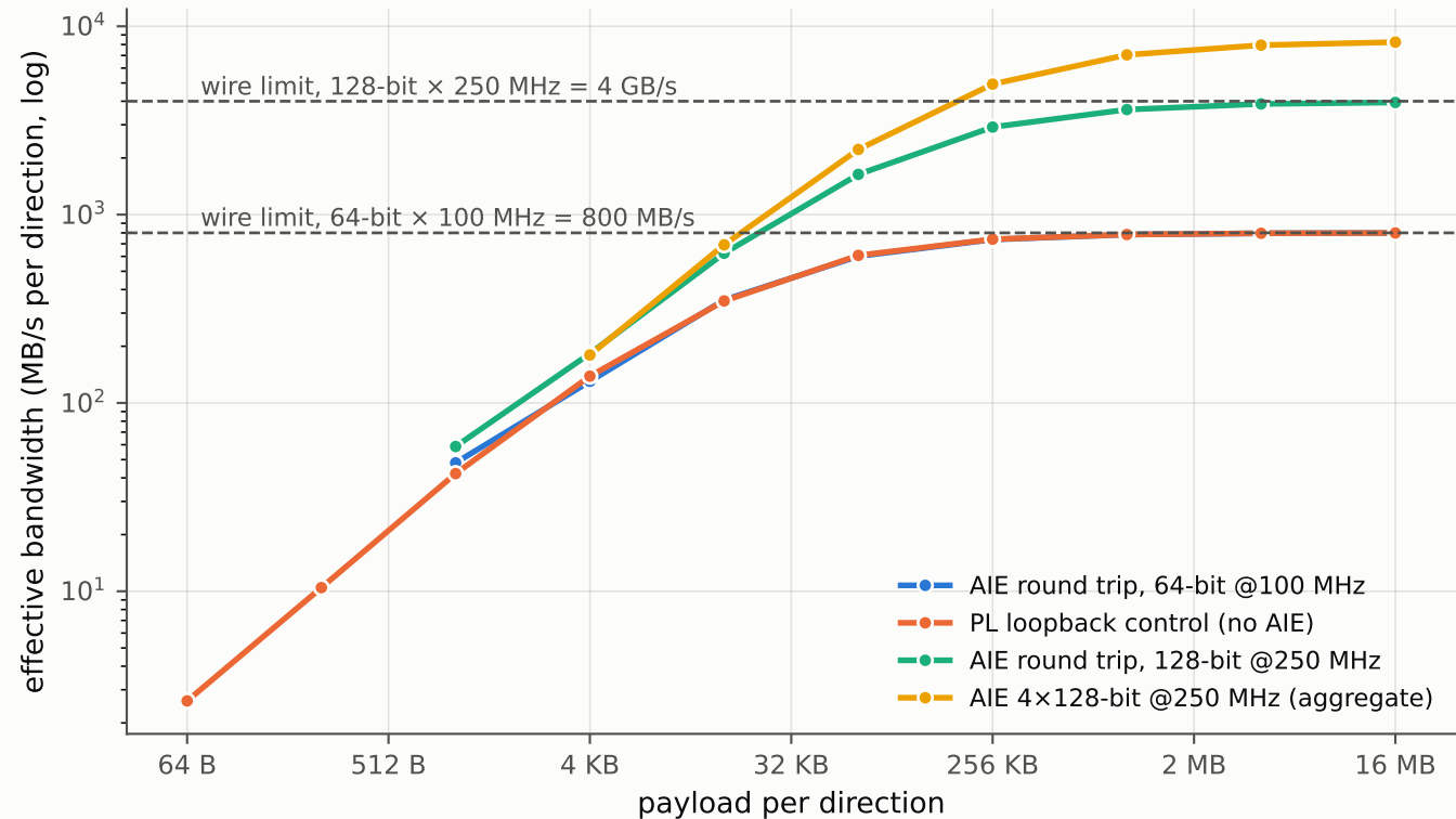
AIE↔PL effective bandwidth vs payload (VCK190, measured)
