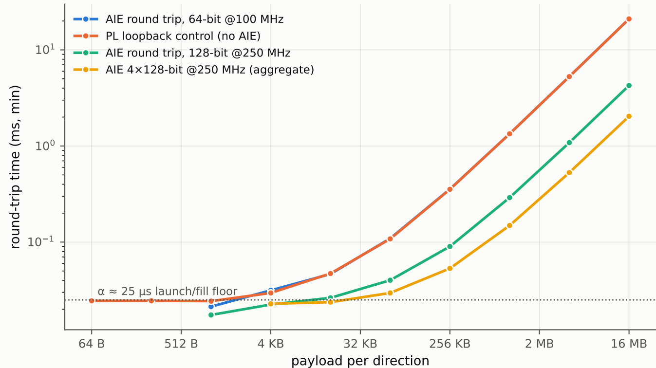
AIE↔PL round-trip time vs payload (VCK190, measured)
