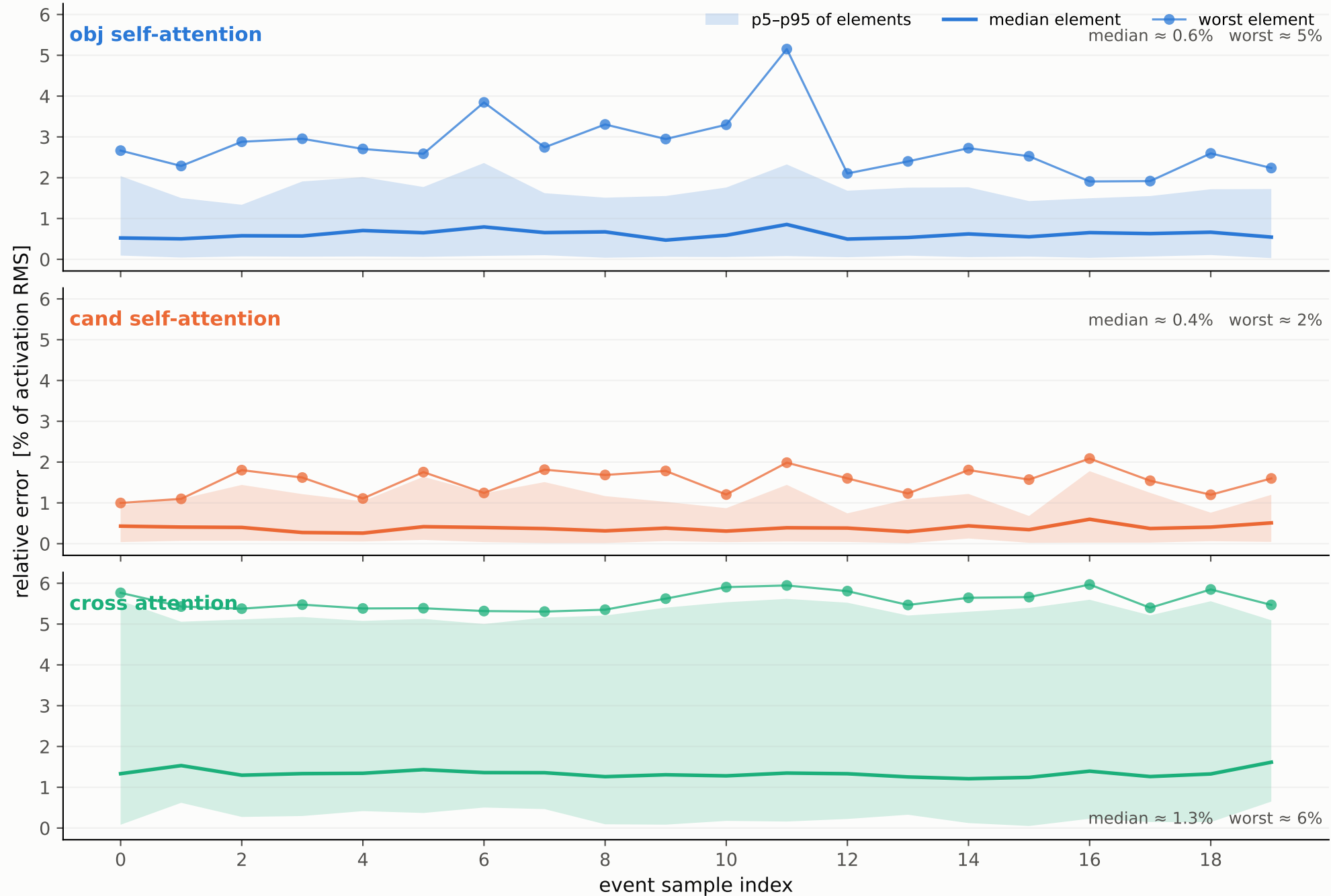
Quantization error of the AIE attention blocks, per event error as % of the event's golden activation RMS · x86sim (bit-exact model of the tiles) vs PyTorch float32, 20 events
