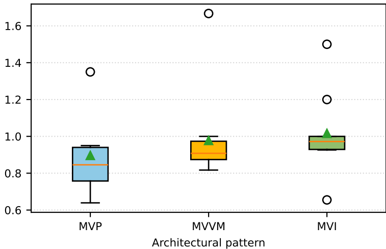
Lack of Cohesion (LCOM-HS)
