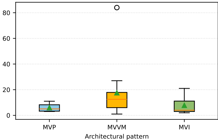
Weighted Methods per Class (WMC)
