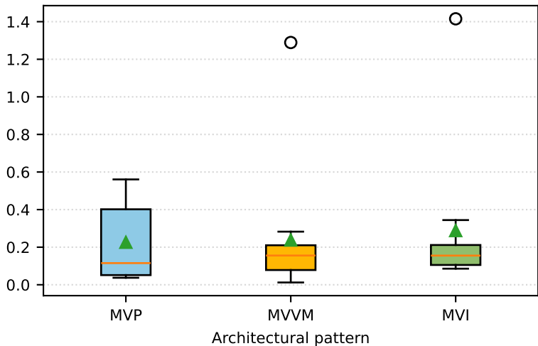
Change frequency (commits/month)
