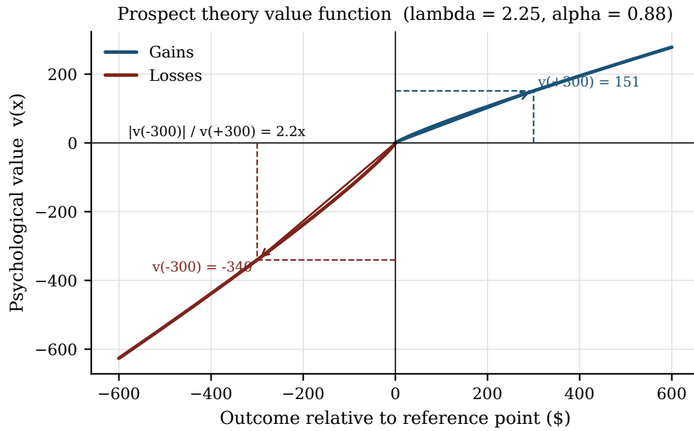
Figure 2.2.: The prospect theory value function (eq. (2.3), \lambda = 2.25 ). Concave in gains (risk-averse); steeply convex in losses (risk-seeking to avoid certain loss). The asymmetry at zero means a loss of any given size looms larger than an equal gain.
