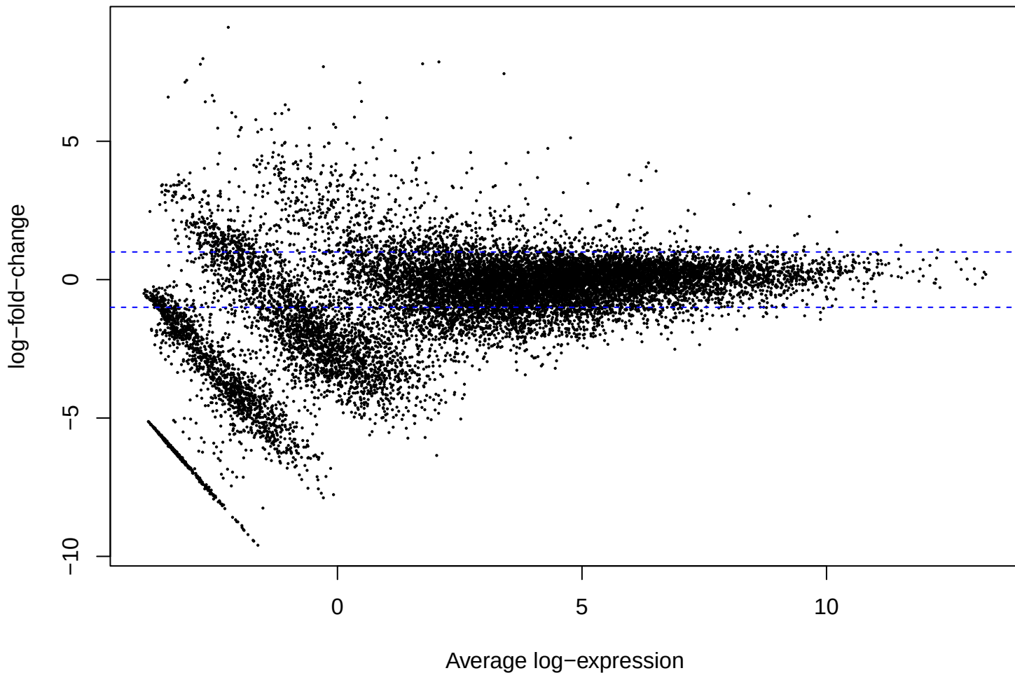
MA Plot: COVID-19 vs Influenza
