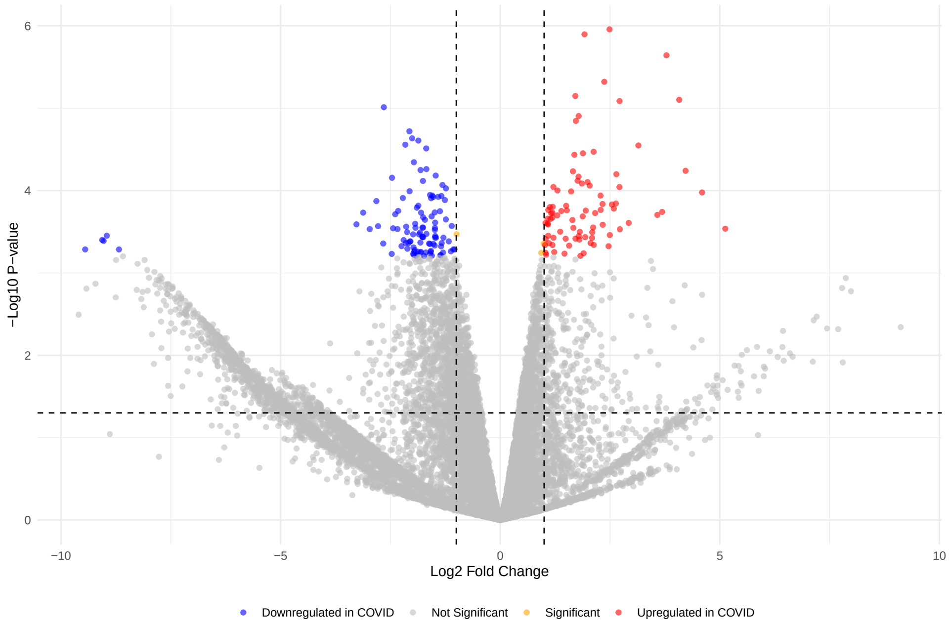
Volcano Plot: COVID-19 vs Influenza
