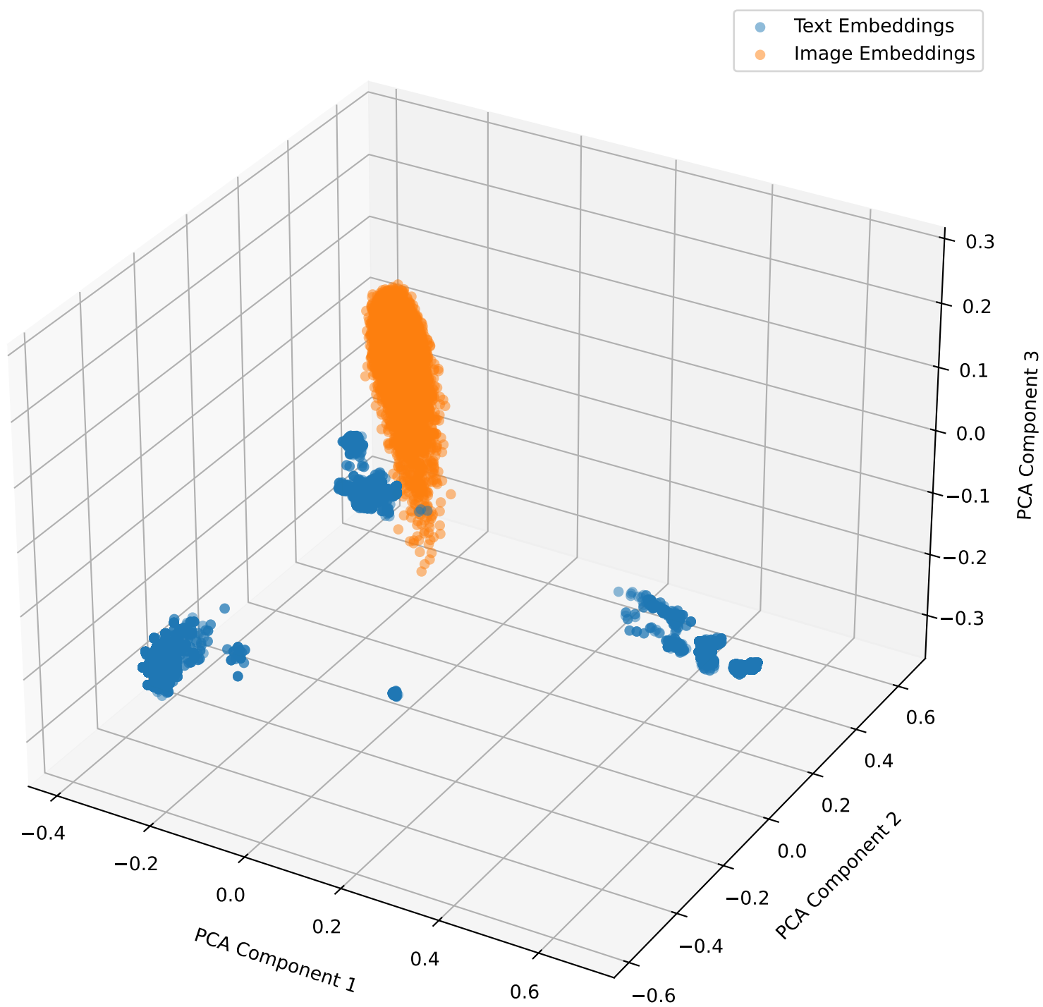
Embeddings with Lambda Shift 0.8 for ham10000 in 3D
