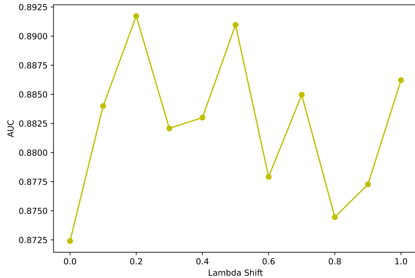
Late Fusion AUC - mbrset
