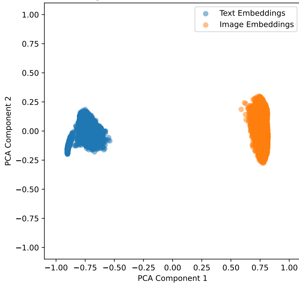
Embeddings with Lambda Shift -1.0 for fakeddit in 2D
