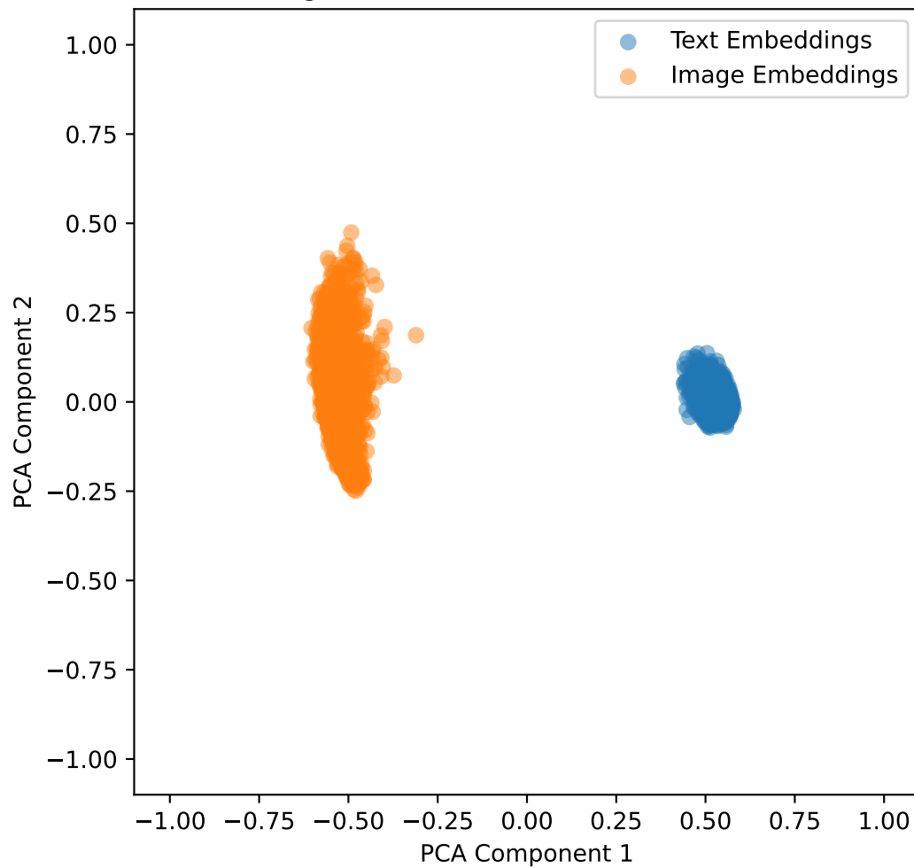
Embeddings with Lambda Shift 0.1 for mbrset in 2D
