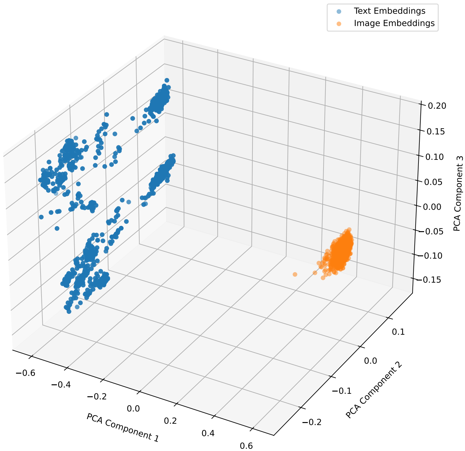
Embeddings with Lambda Shift 0.2 for mbrset in 3D
