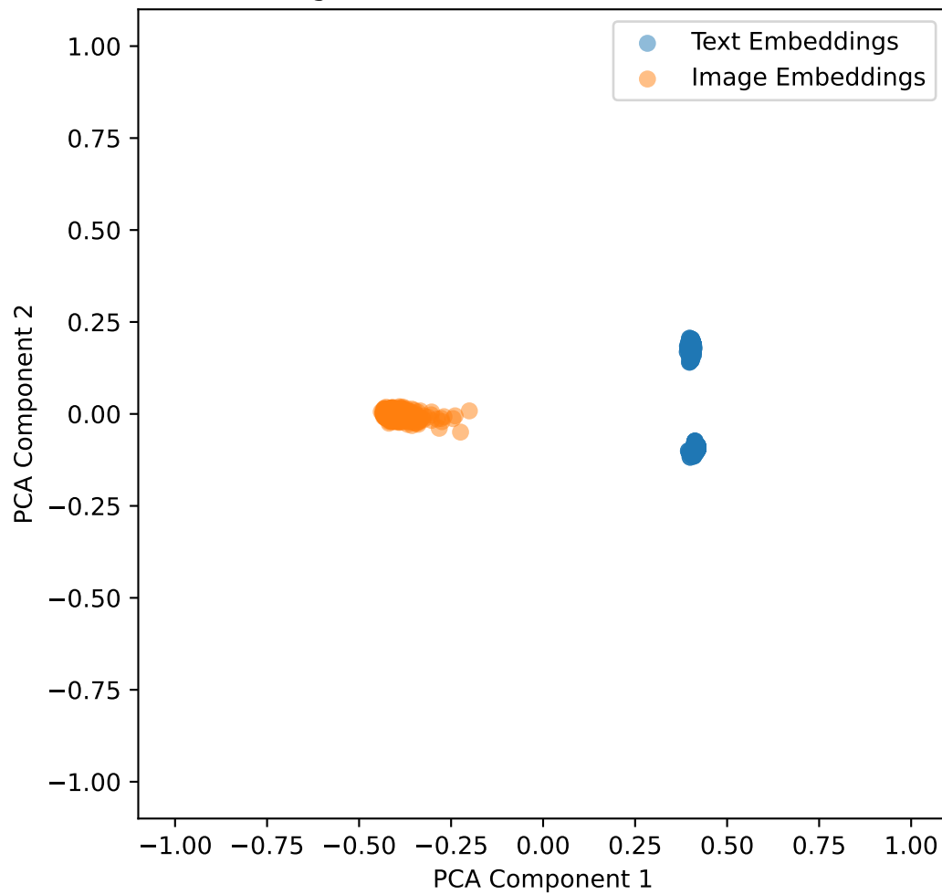
Embeddings with Lambda Shift 0.4 for mbrset in 2D
