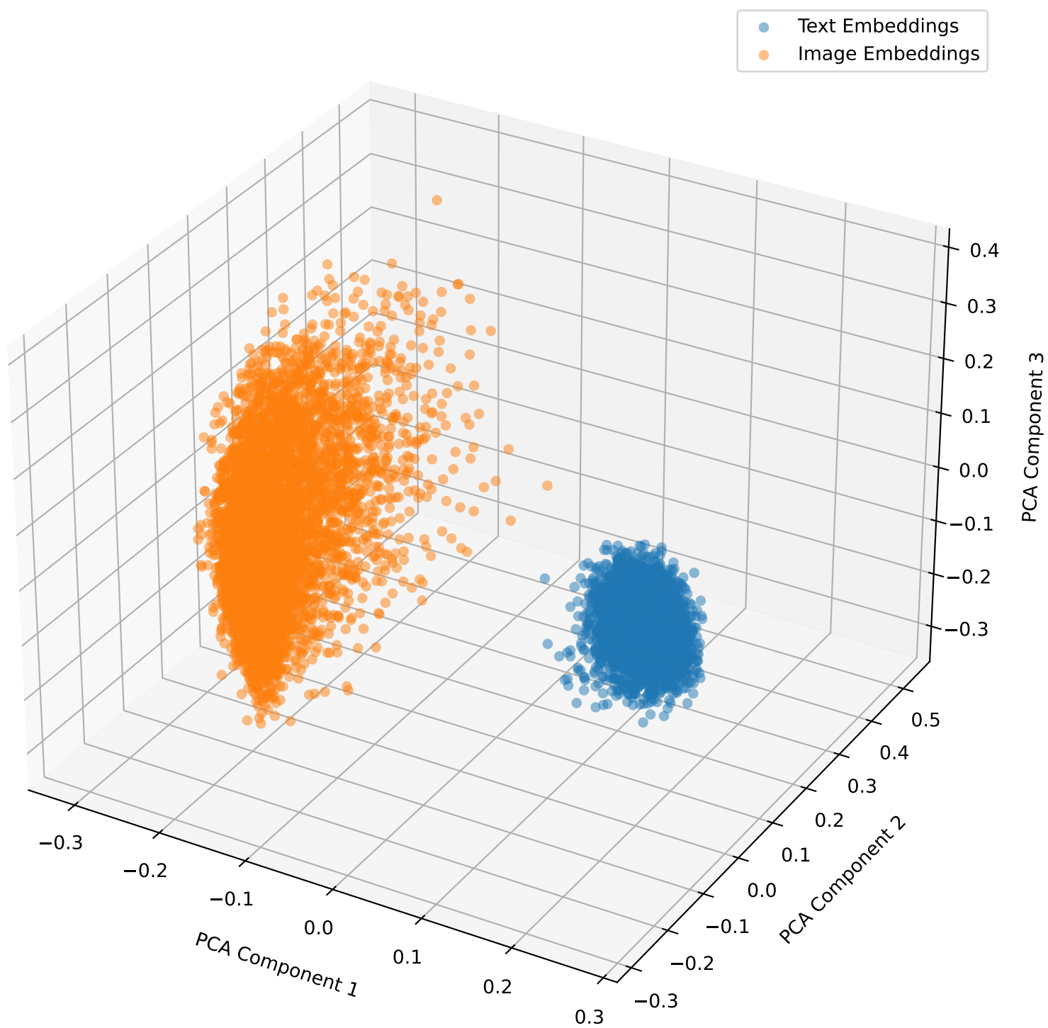
Embeddings with Lambda Shift 0.7 for mbrset in 3D
