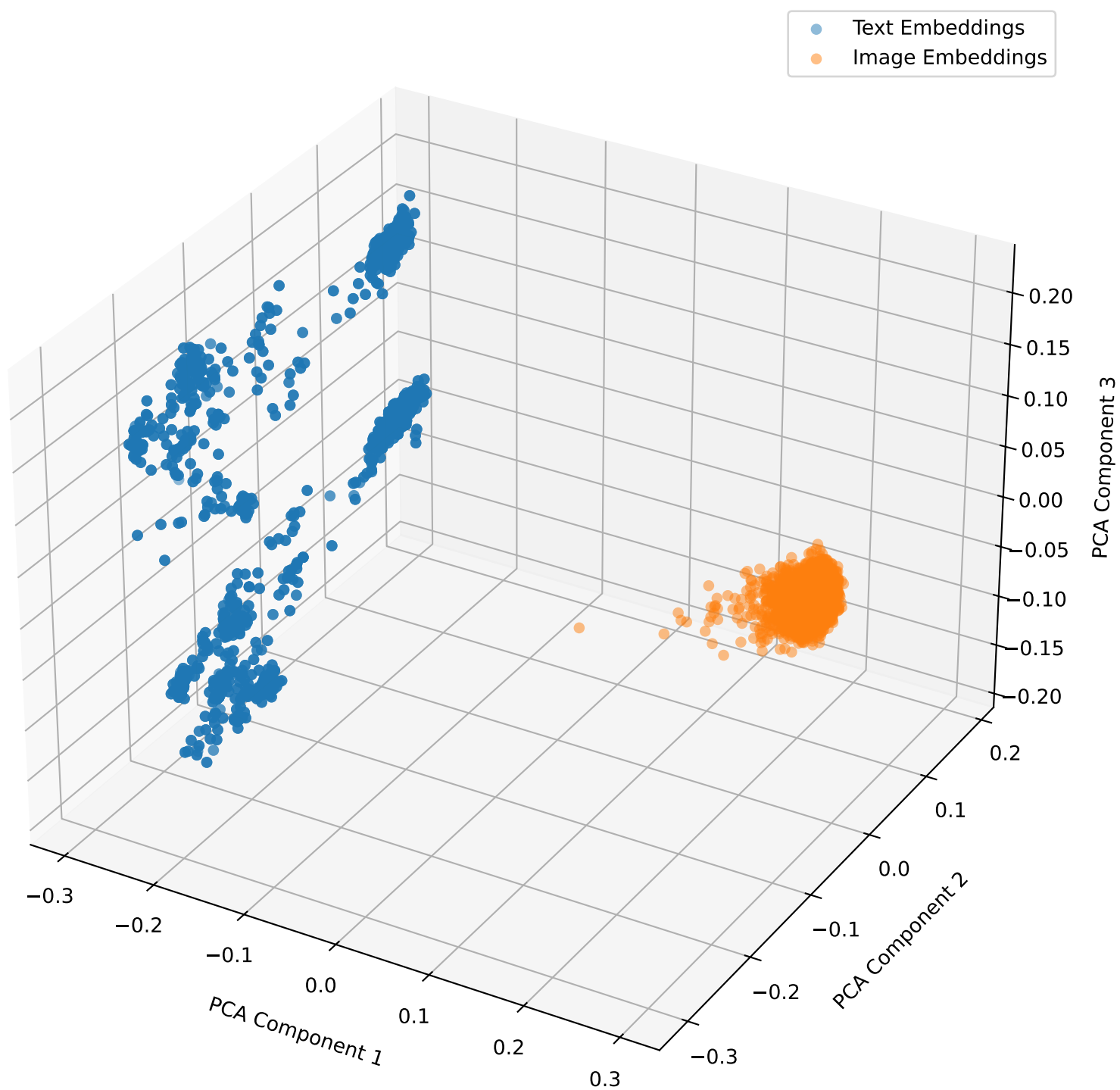
Embeddings with Lambda Shift 0.7 for mbrset in 3D
