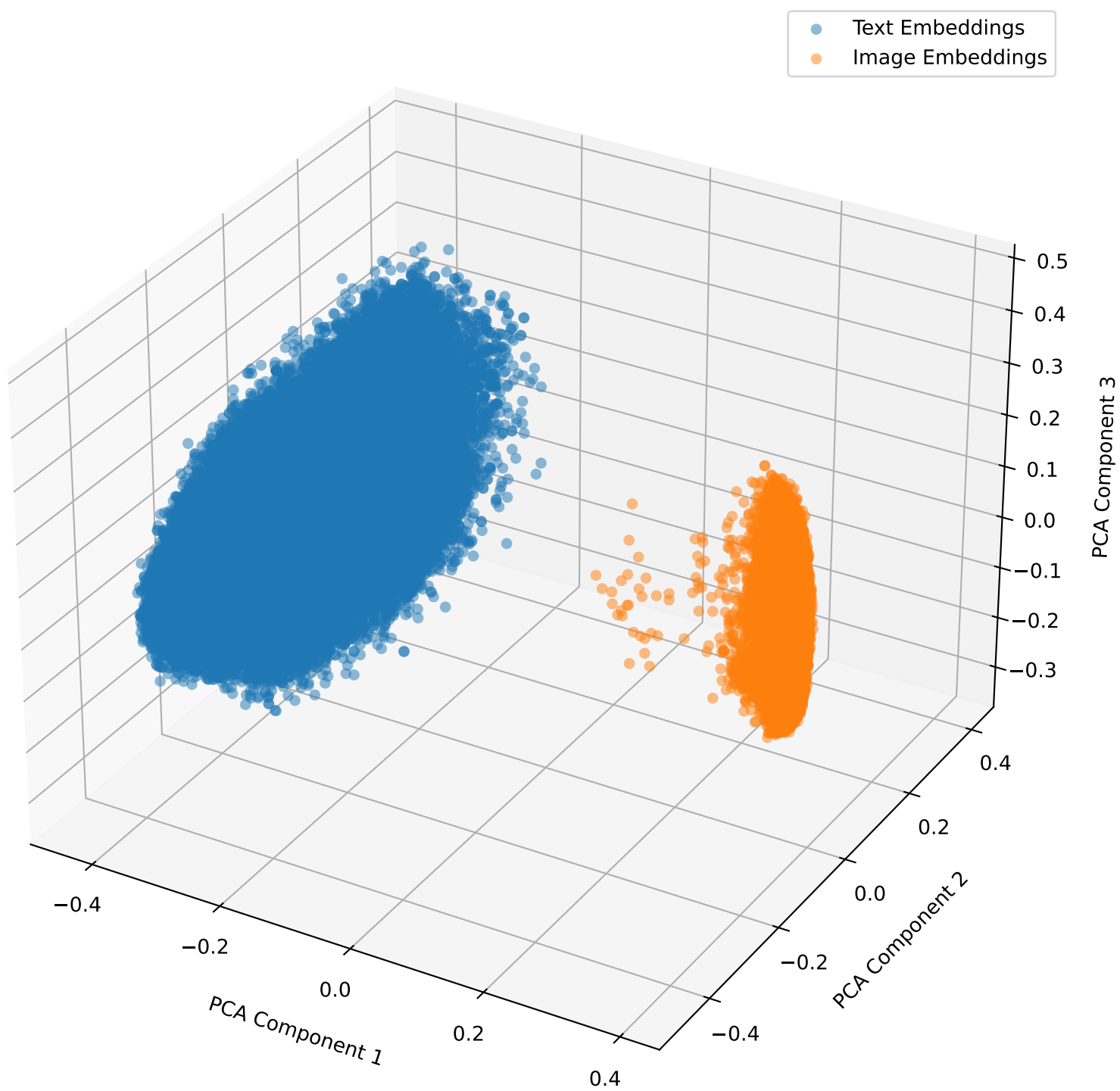
Embeddings with Lambda Shift 0.5 for mimic in 3D
