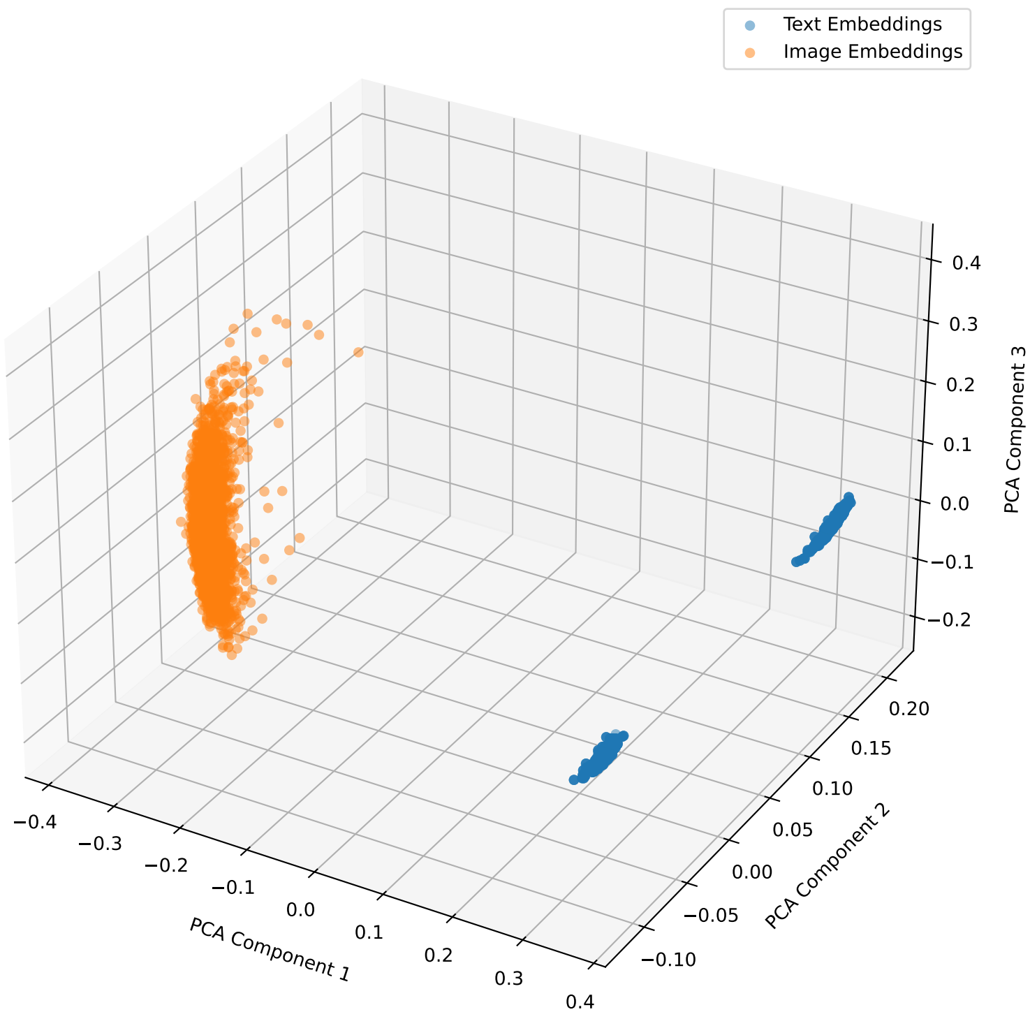
Embeddings with Lambda Shift 0.5 for mbrset in 3D
