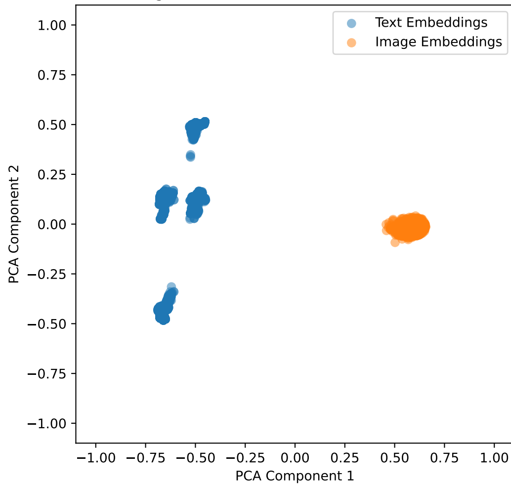
Embeddings with Lambda Shift 0.1 for ham10000 in 2D
