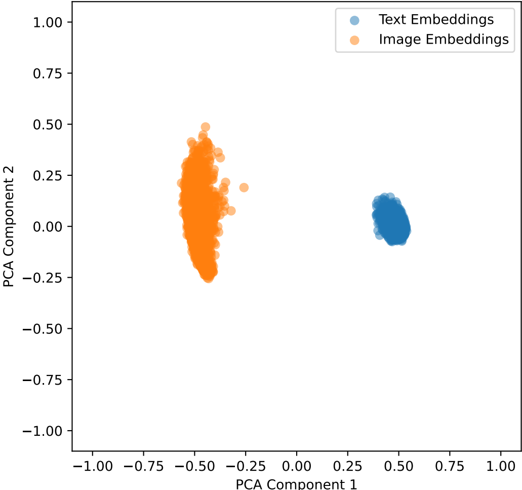
Embeddings with Lambda Shift 0.2 for mbrset in 2D
