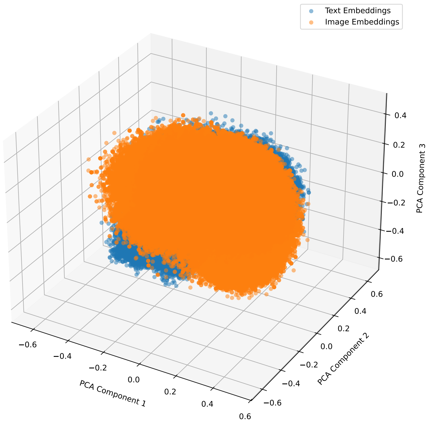
Embeddings with Lambda Shift 1.0 for coco-qa in 3D
