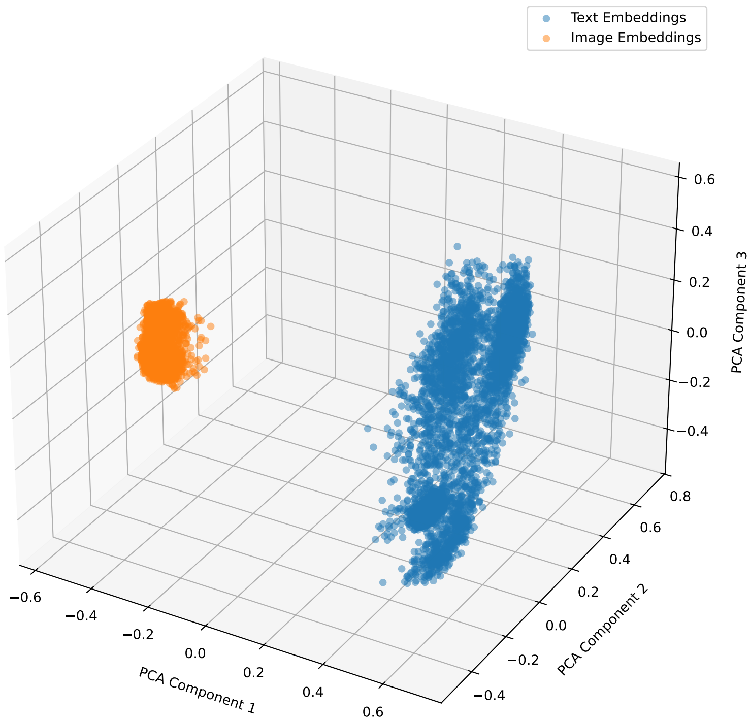
Embeddings with Lambda Shift 0.0 for Recipes5k in 3D
