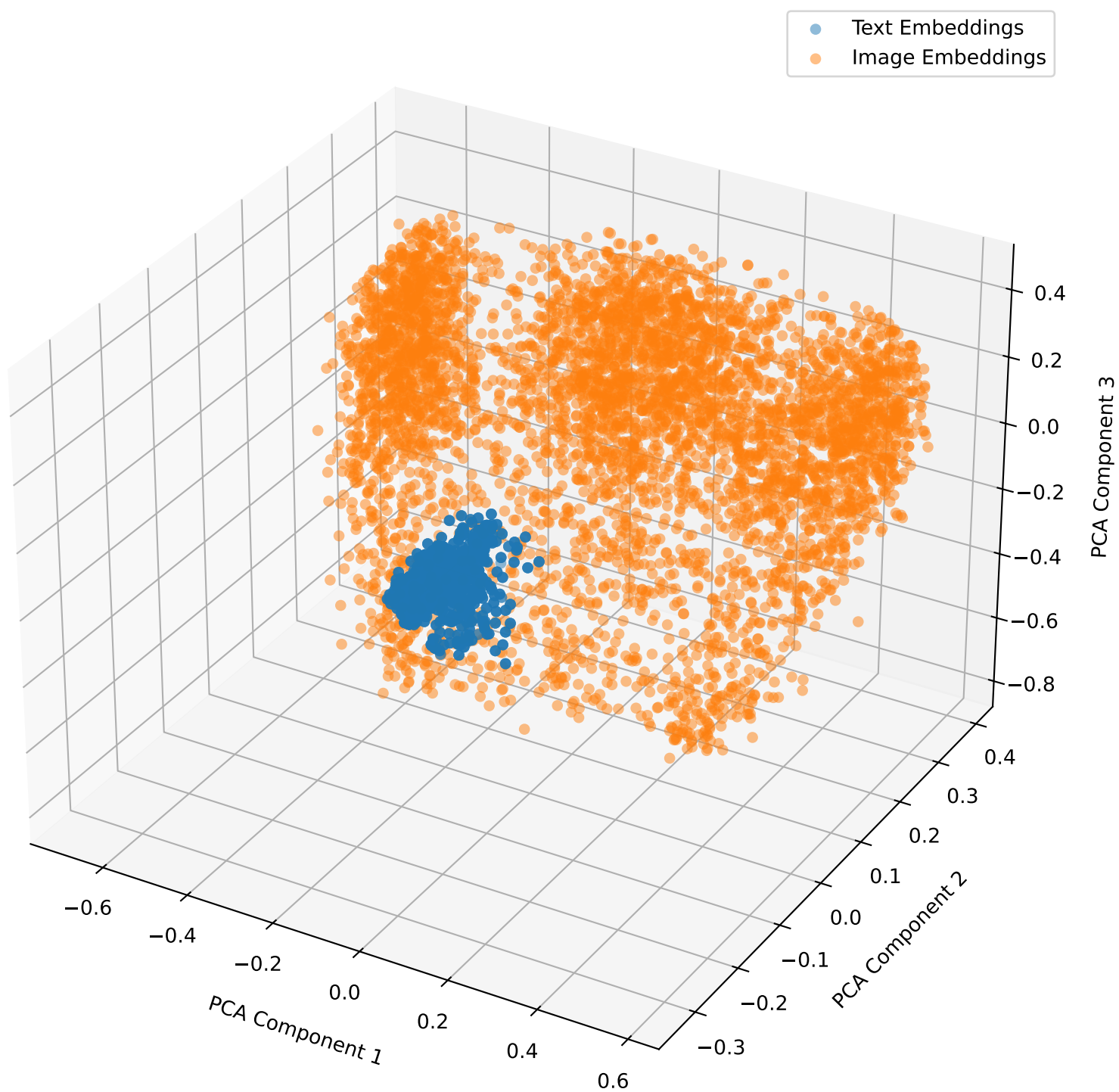
Embeddings with Lambda Shift 0.8 for mbrset in 3D
