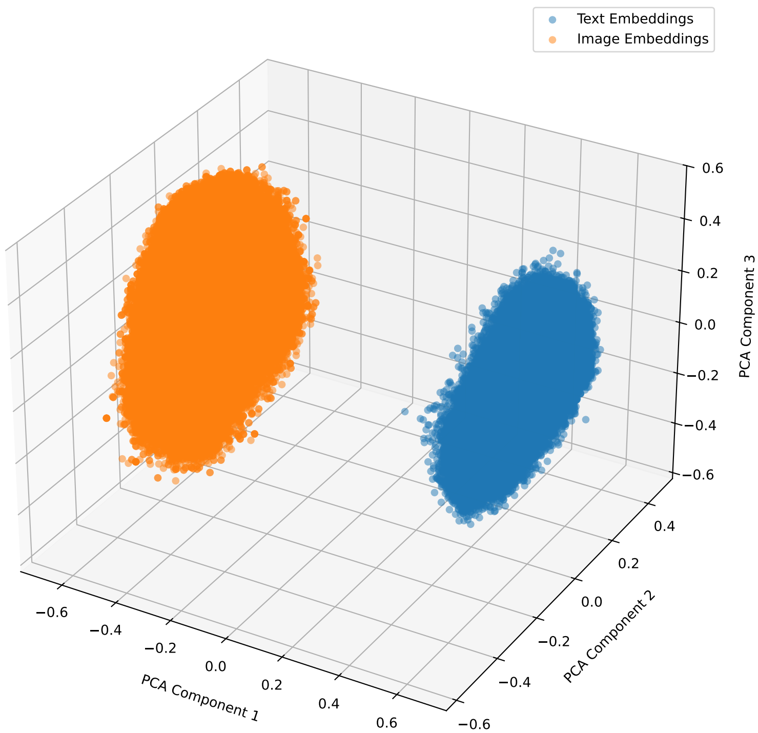
Embeddings with Lambda Shift -0.5 for coco-qa in 3D
