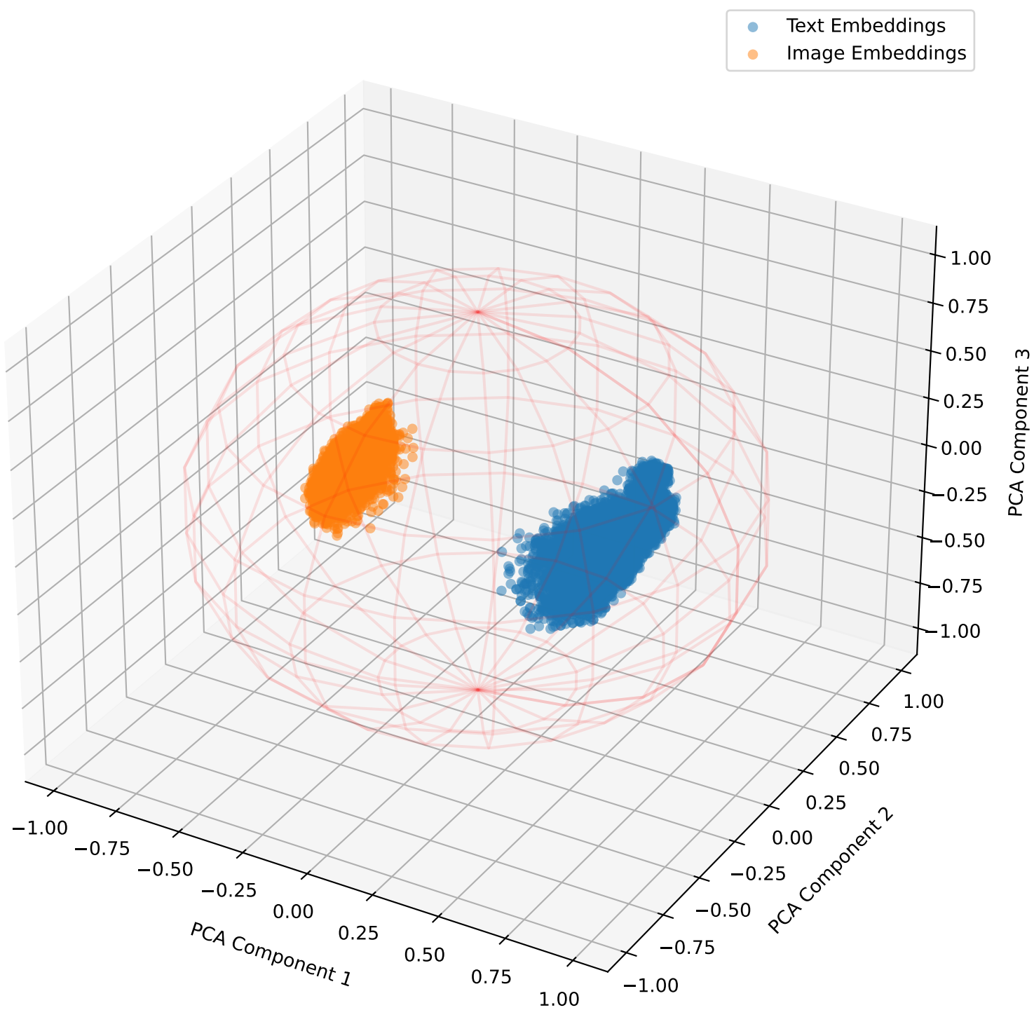
Embeddings with Lambda Shift -0.1 for Recipes5k in 3D
