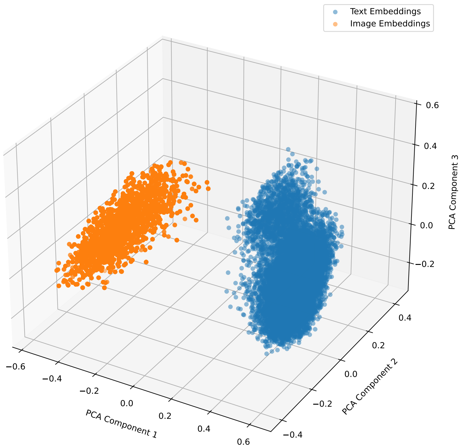
Embeddings with Lambda Shift 0.0 for daquar in 3D
