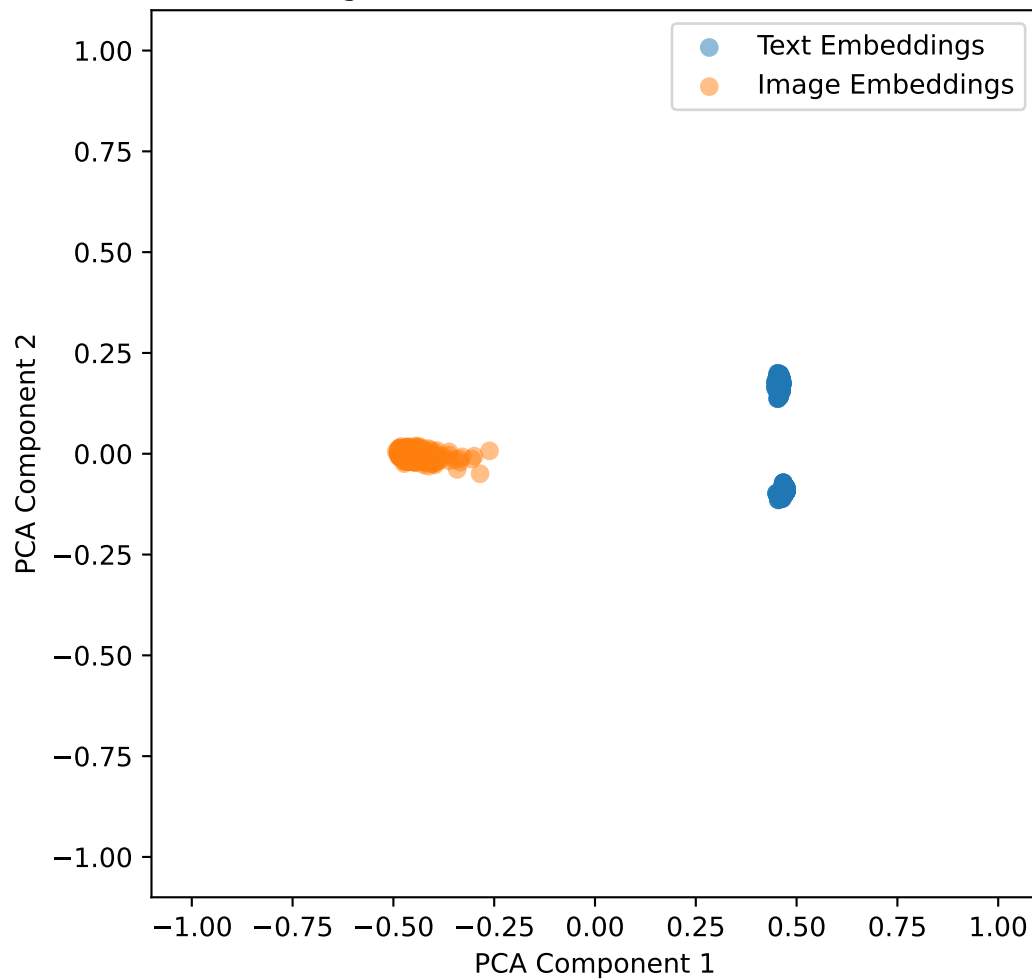
Embeddings with Lambda Shift 0.3 for mbrset in 2D
