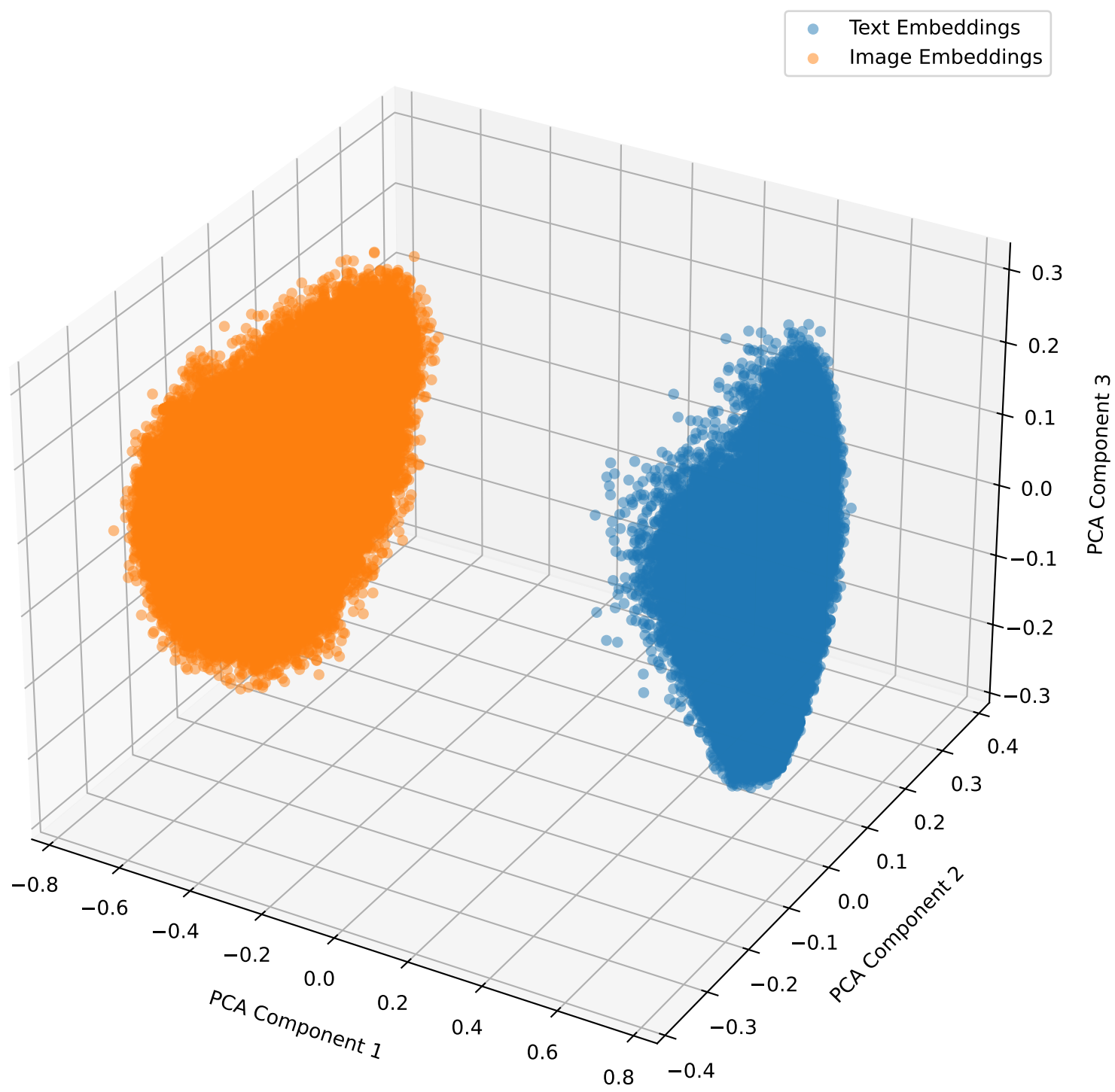
Embeddings with Lambda Shift -1.0 for fakeddit in 3D
