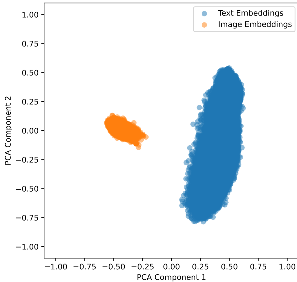
Embeddings with Lambda Shift 0.0 for fakeddit in 2D
