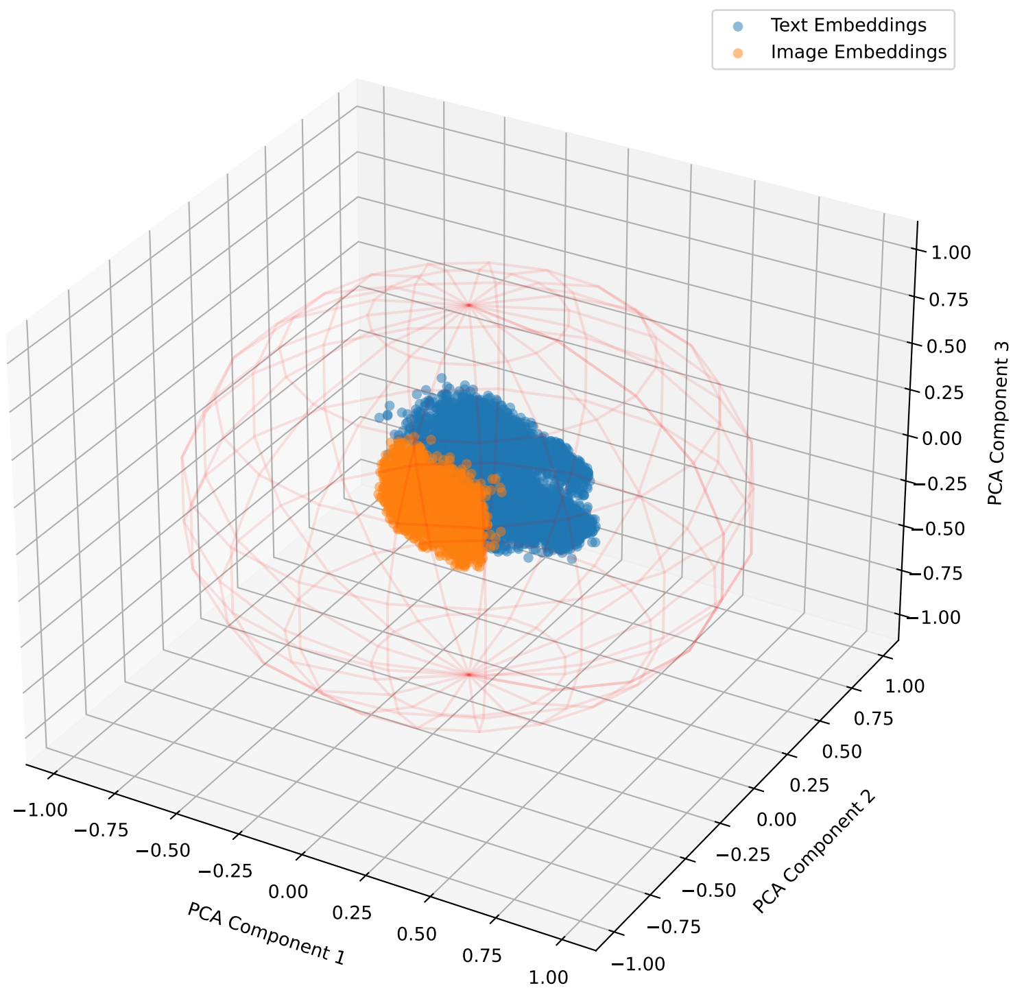
Embeddings with Lambda Shift 0.7 for Recipes5k in 3D
