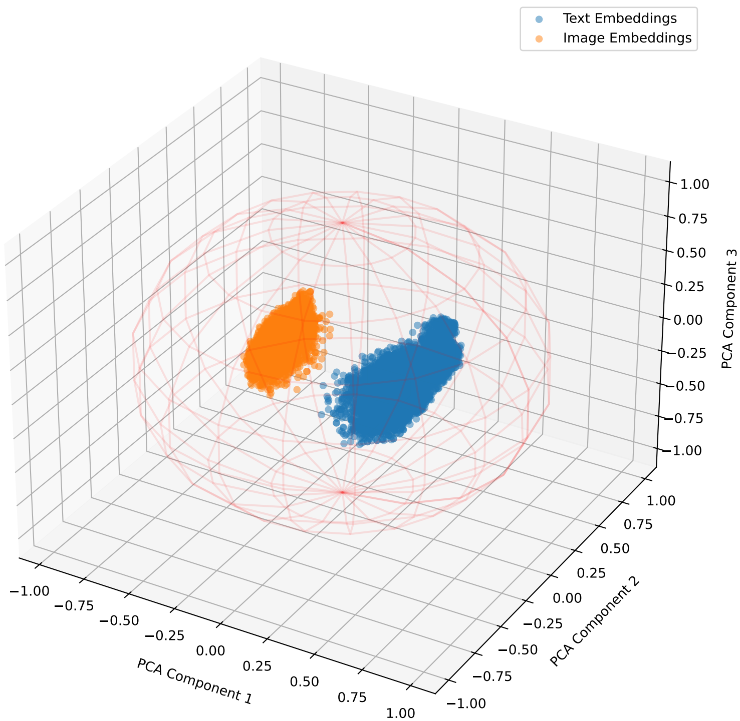
Embeddings with Lambda Shift 0.3 for Recipes5k in 3D
