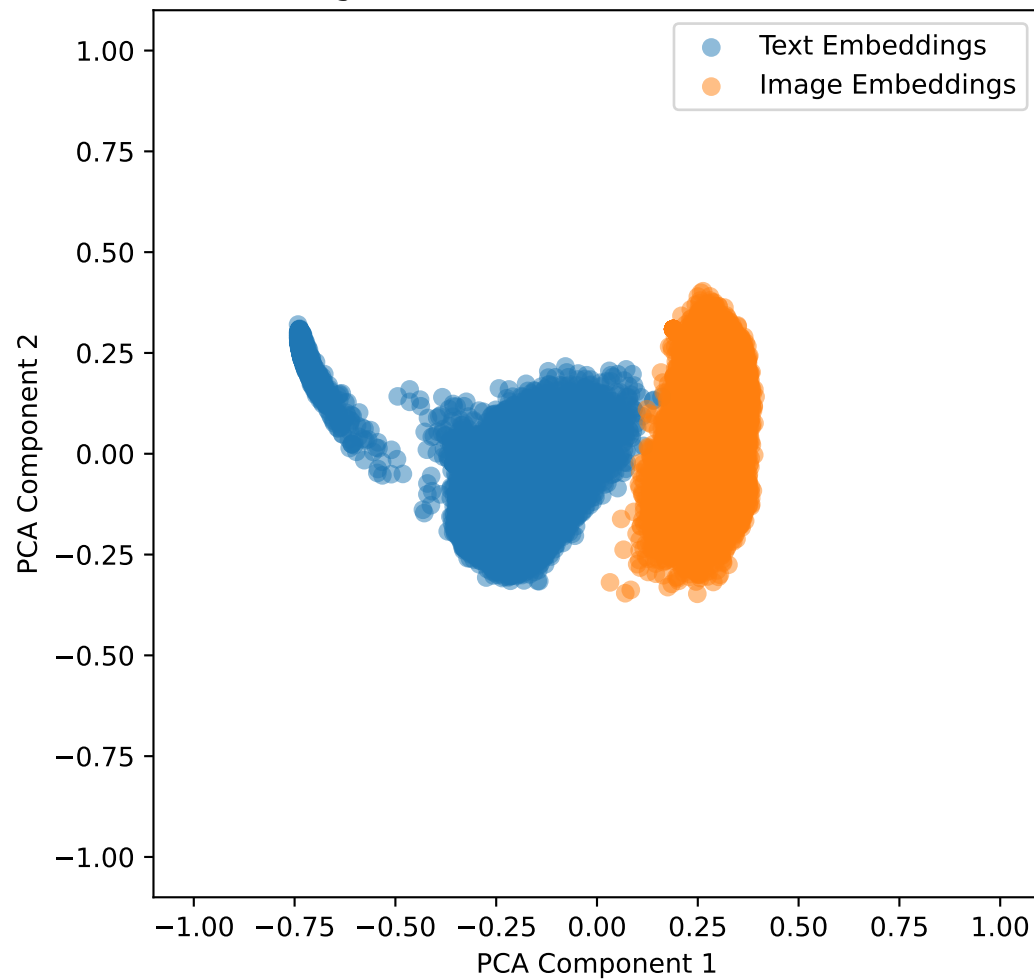
Embeddings with Lambda Shift 0.5 for fakeddit in 2D
