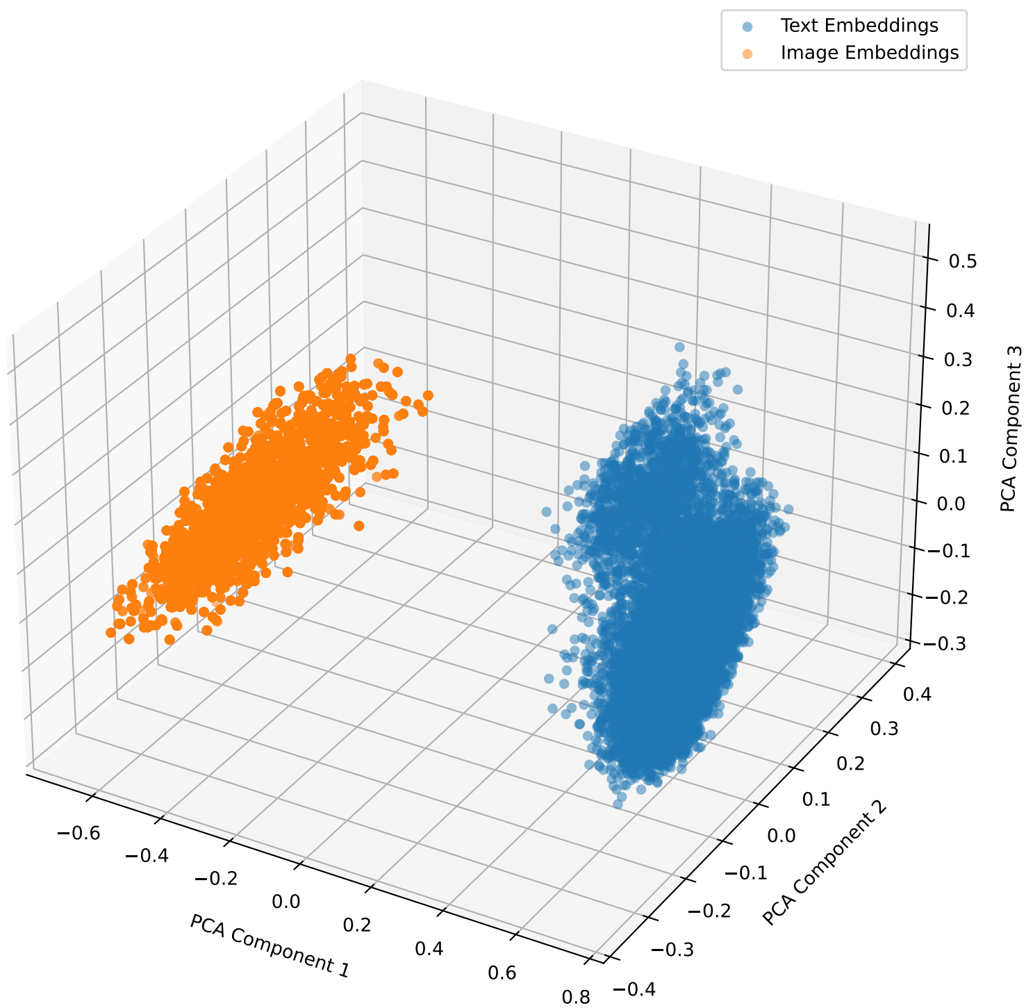
Embeddings with Lambda Shift -0.5 for daquar in 3D
