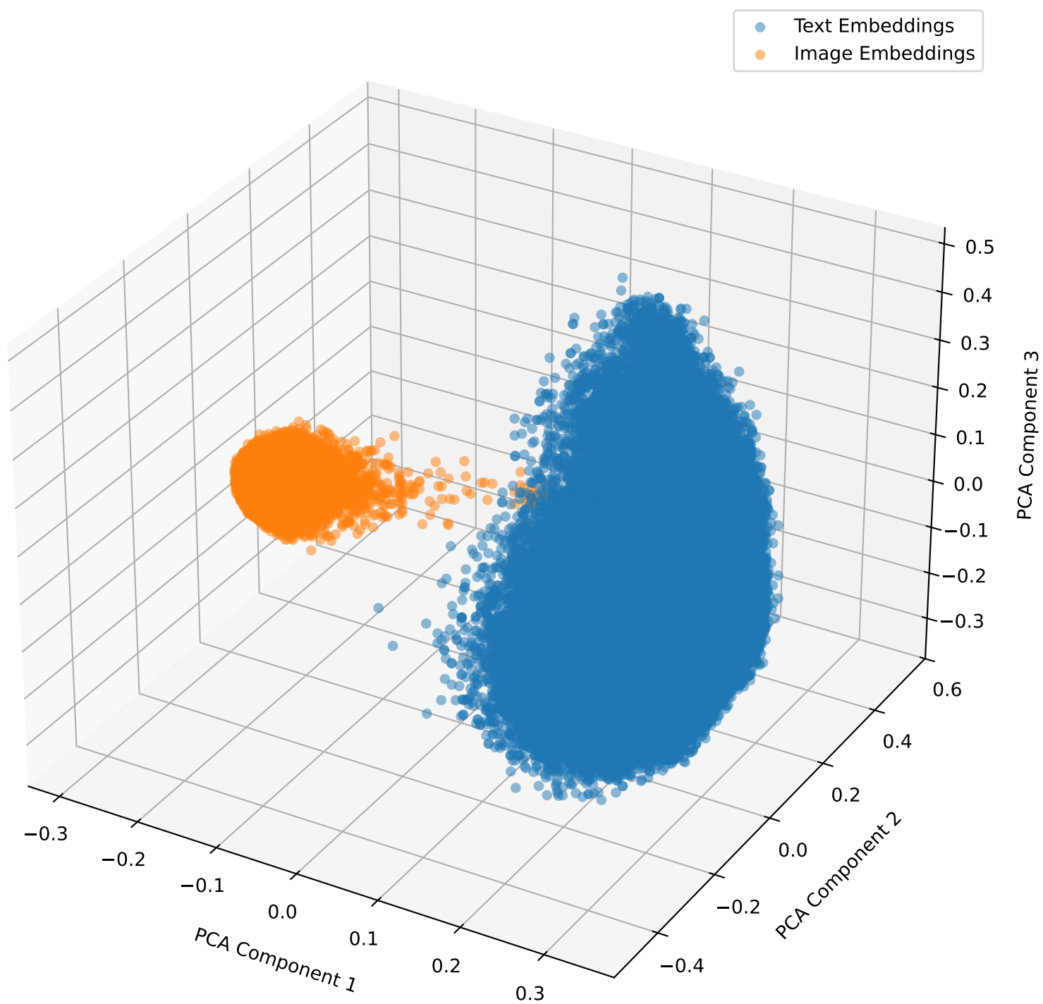
Embeddings with Lambda Shift 0.6 for mimic in 3D
