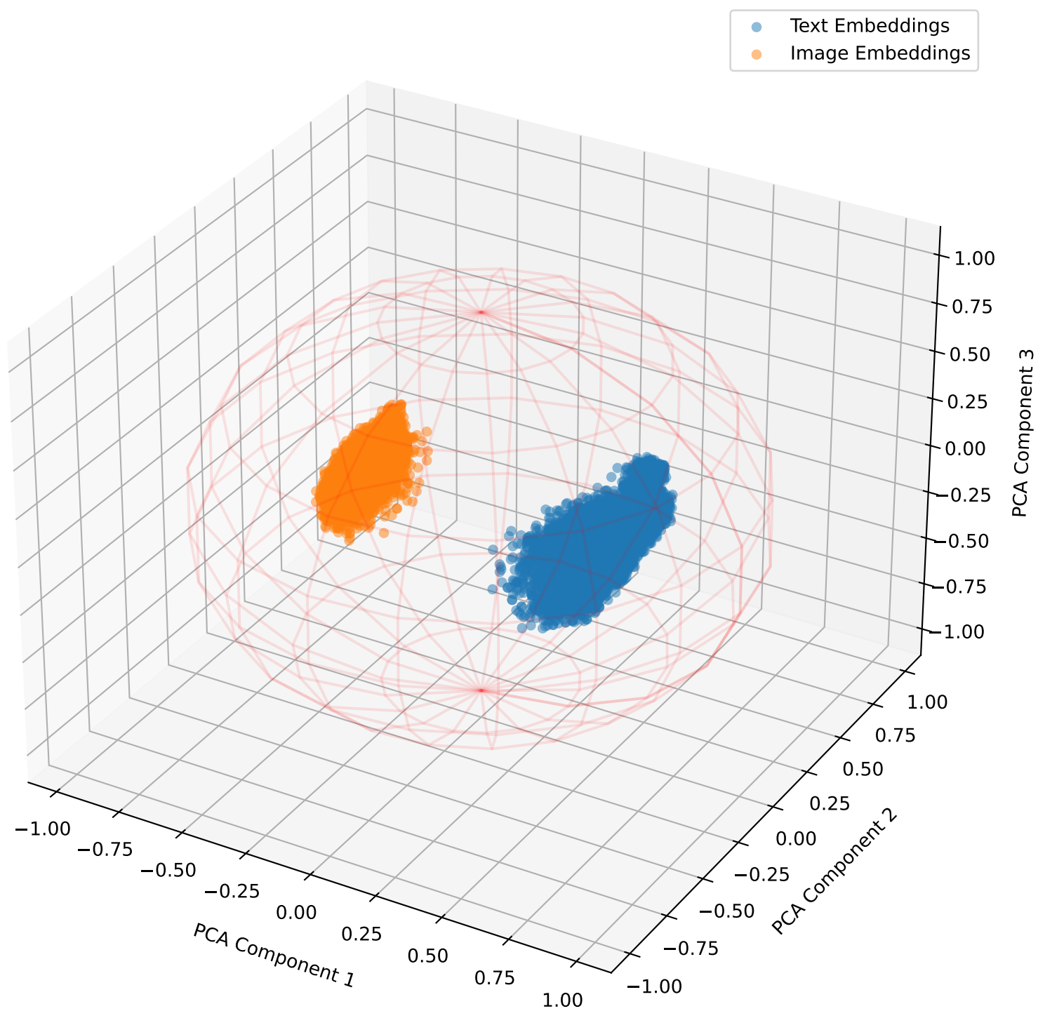
Embeddings with Lambda Shift 0 for Recipes5k in 3D
