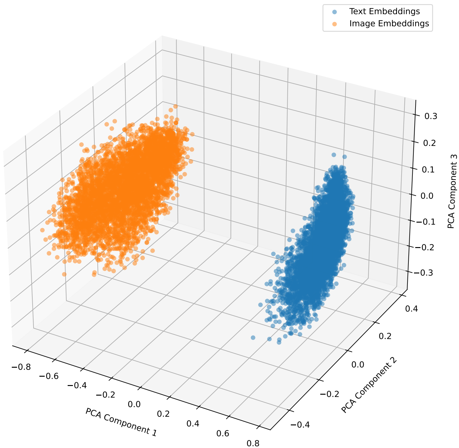
Embeddings with Lambda Shift -1.0 for Recipes5k in 3D
