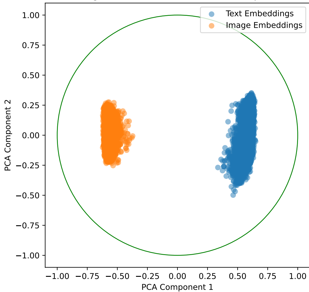
Embeddings with Lambda Shift -0.3 for Recipes5k in 2D
