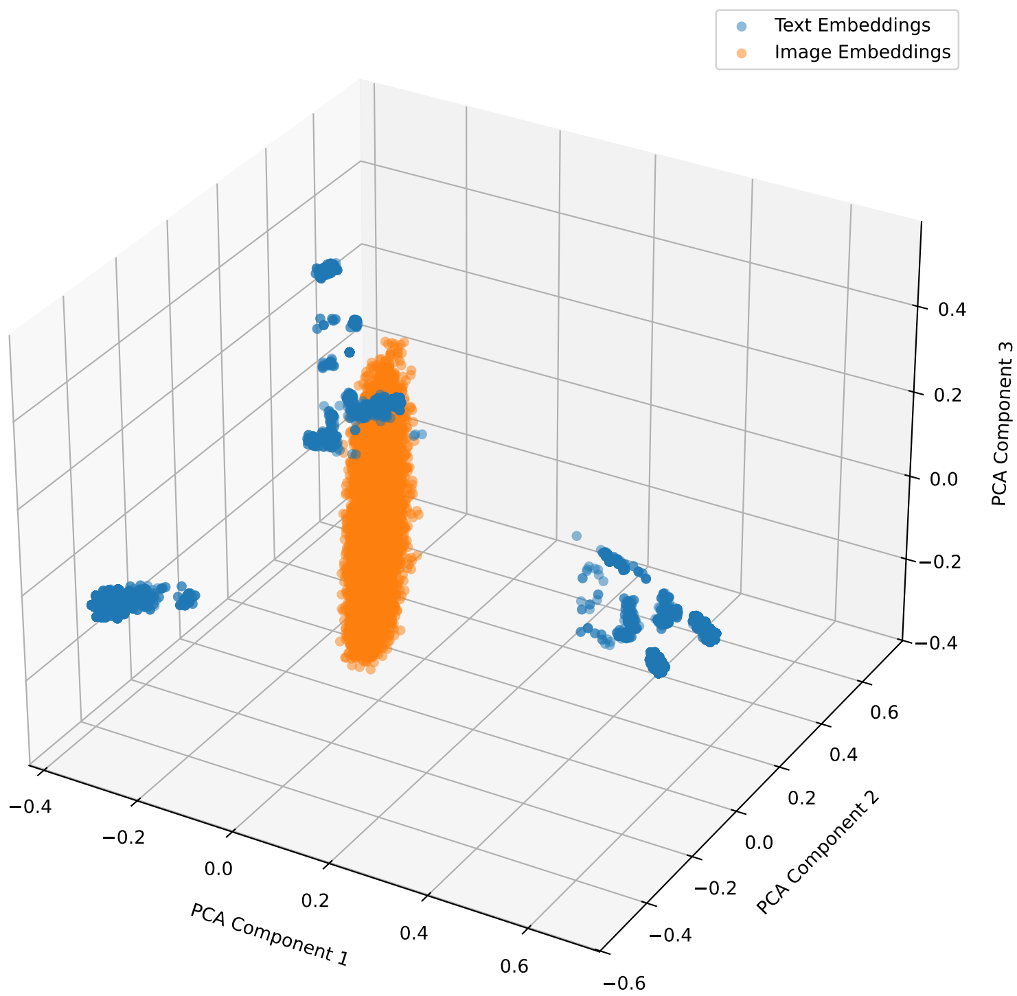
Embeddings with Lambda Shift 0.9 for ham10000 in 3D
