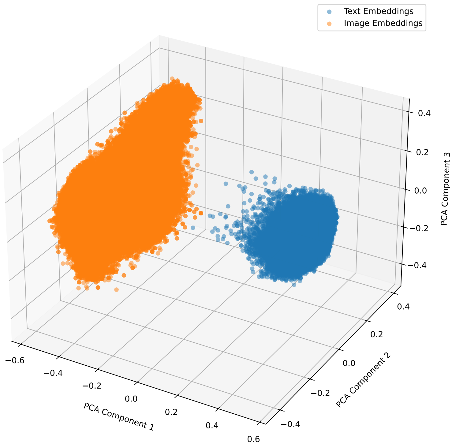
Embeddings with Lambda Shift 0.0 for coco-qa in 3D
