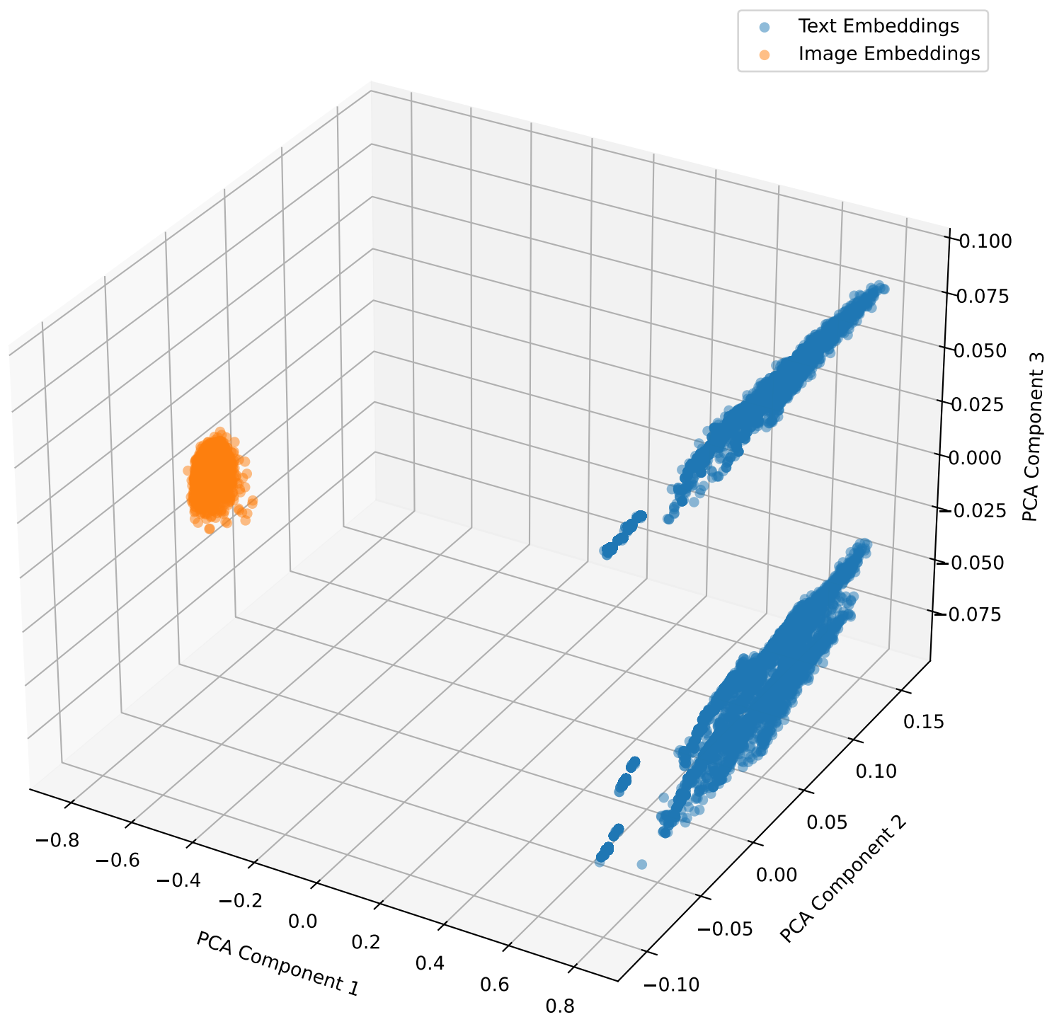
Embeddings with Lambda Shift -1.0 for brset in 3D
