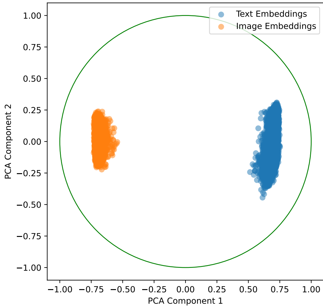
Embeddings with Lambda Shift -0.8 for Recipes5k in 2D
