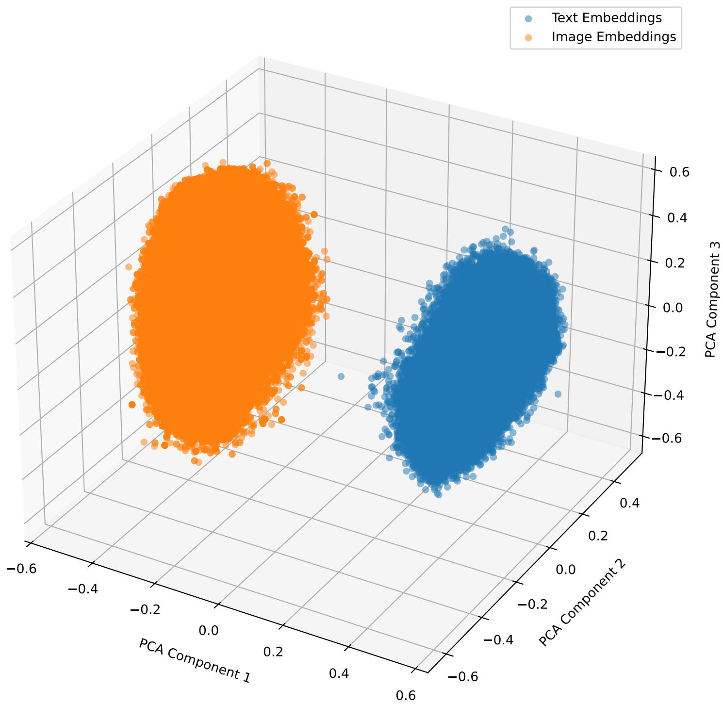
Embeddings with Lambda Shift 0.0 for coco-qa in 3D
