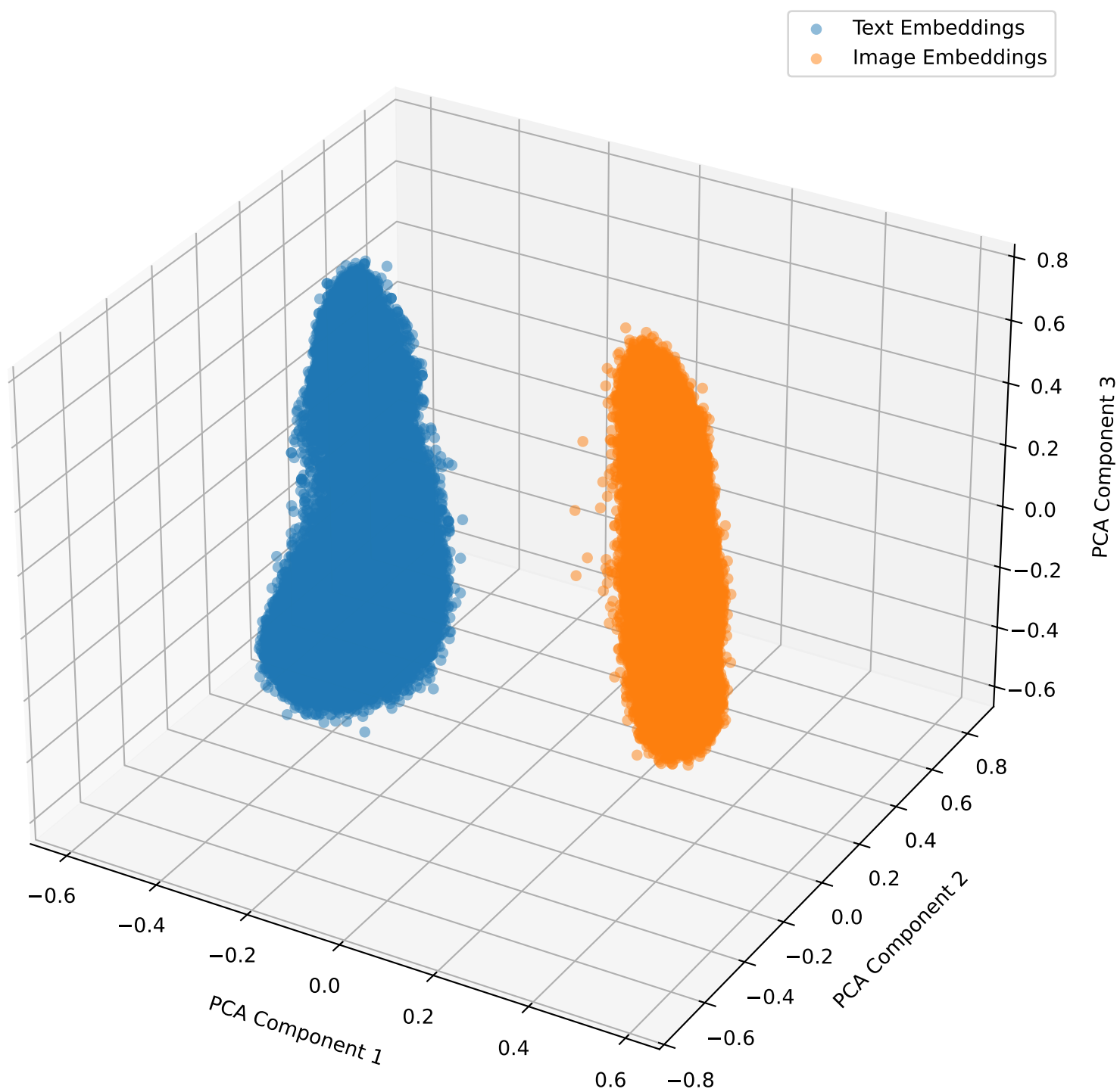
Embeddings with Lambda Shift 0.4 for mimic in 3D
