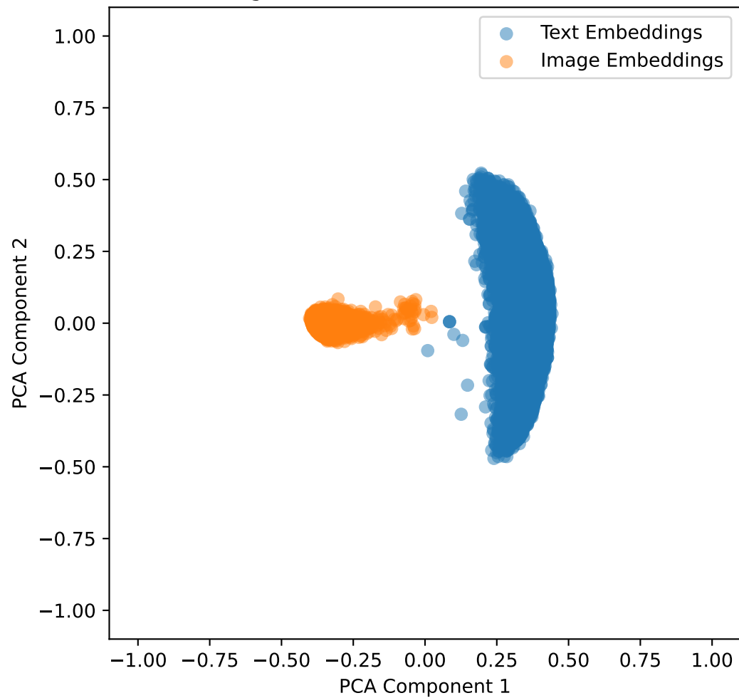
Embeddings with Lambda Shift 0.4 for mimic in 2D
