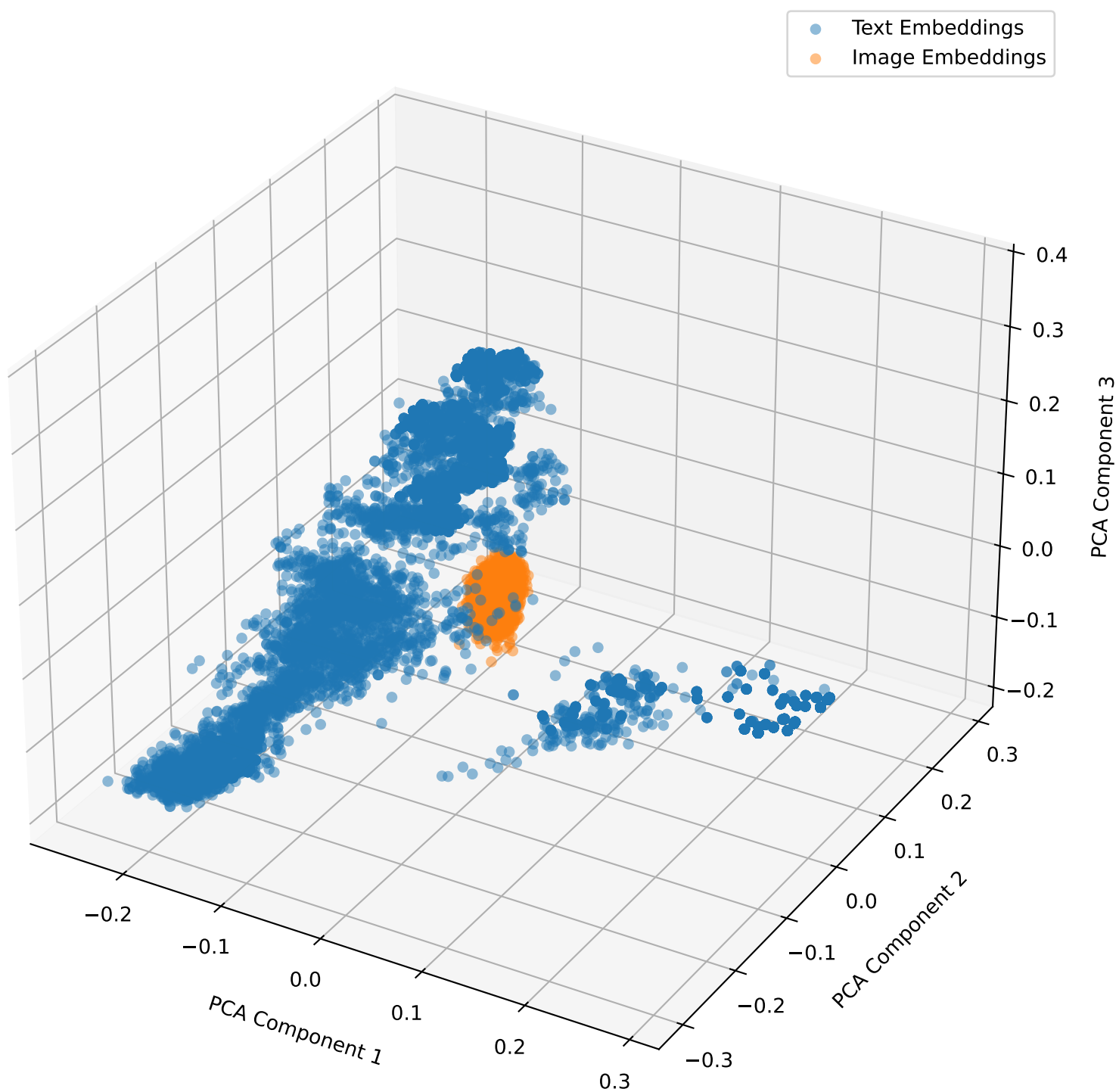
Embeddings with Lambda Shift 0.9 for brset in 3D
