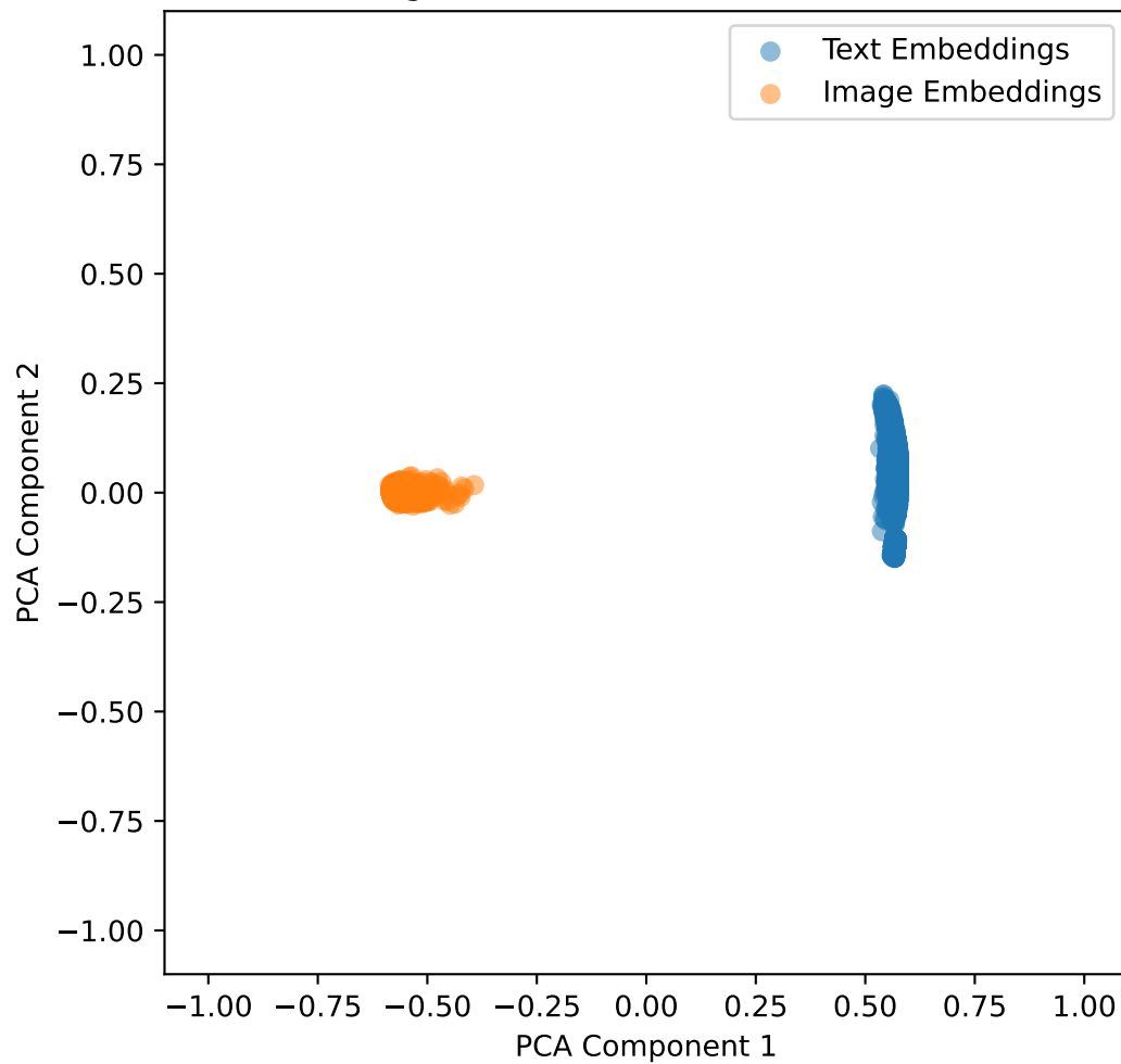
Embeddings with Lambda Shift 0 for brset in 2D
