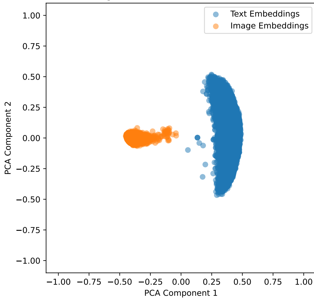
Embeddings with Lambda Shift 0.3 for mimic in 2D
