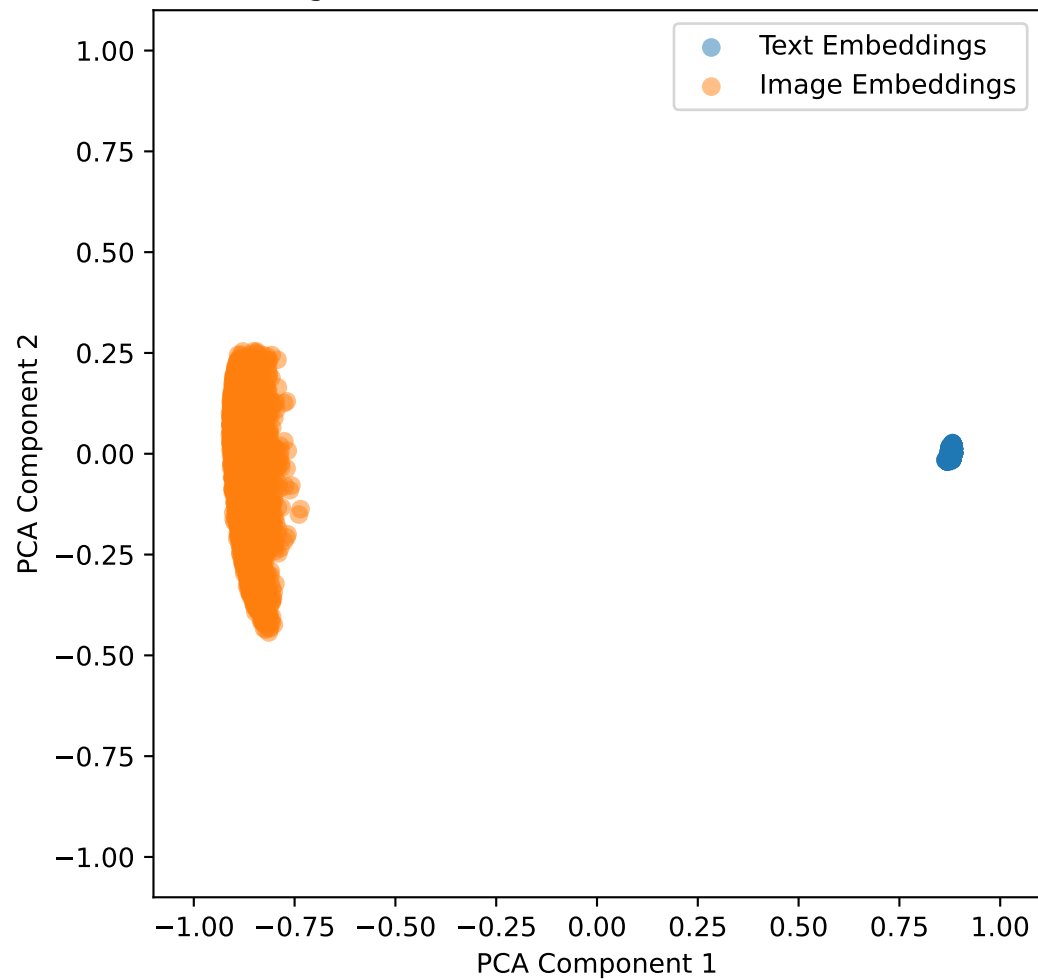
Embeddings with Lambda Shift -1.0 for ham10000 in 2D
