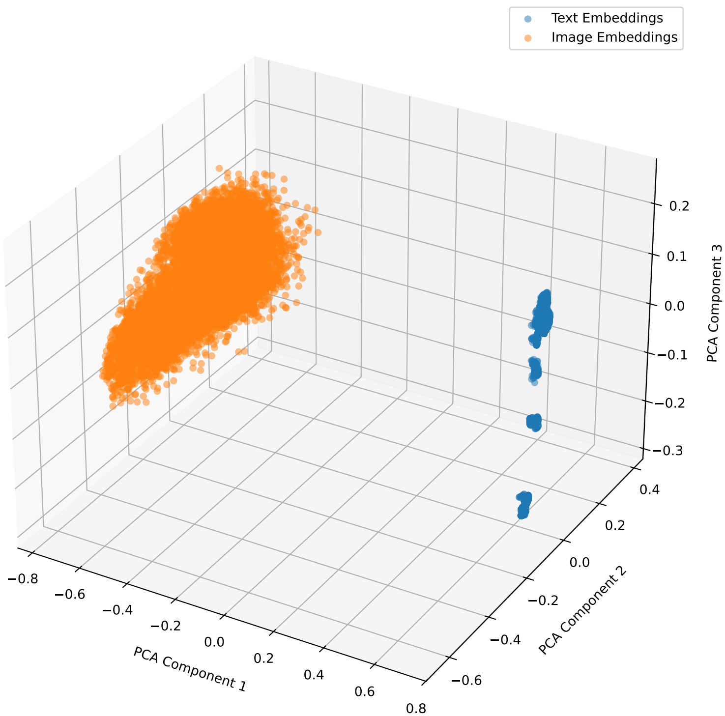
Embeddings with Lambda Shift 0.0 for ham10000 in 3D
