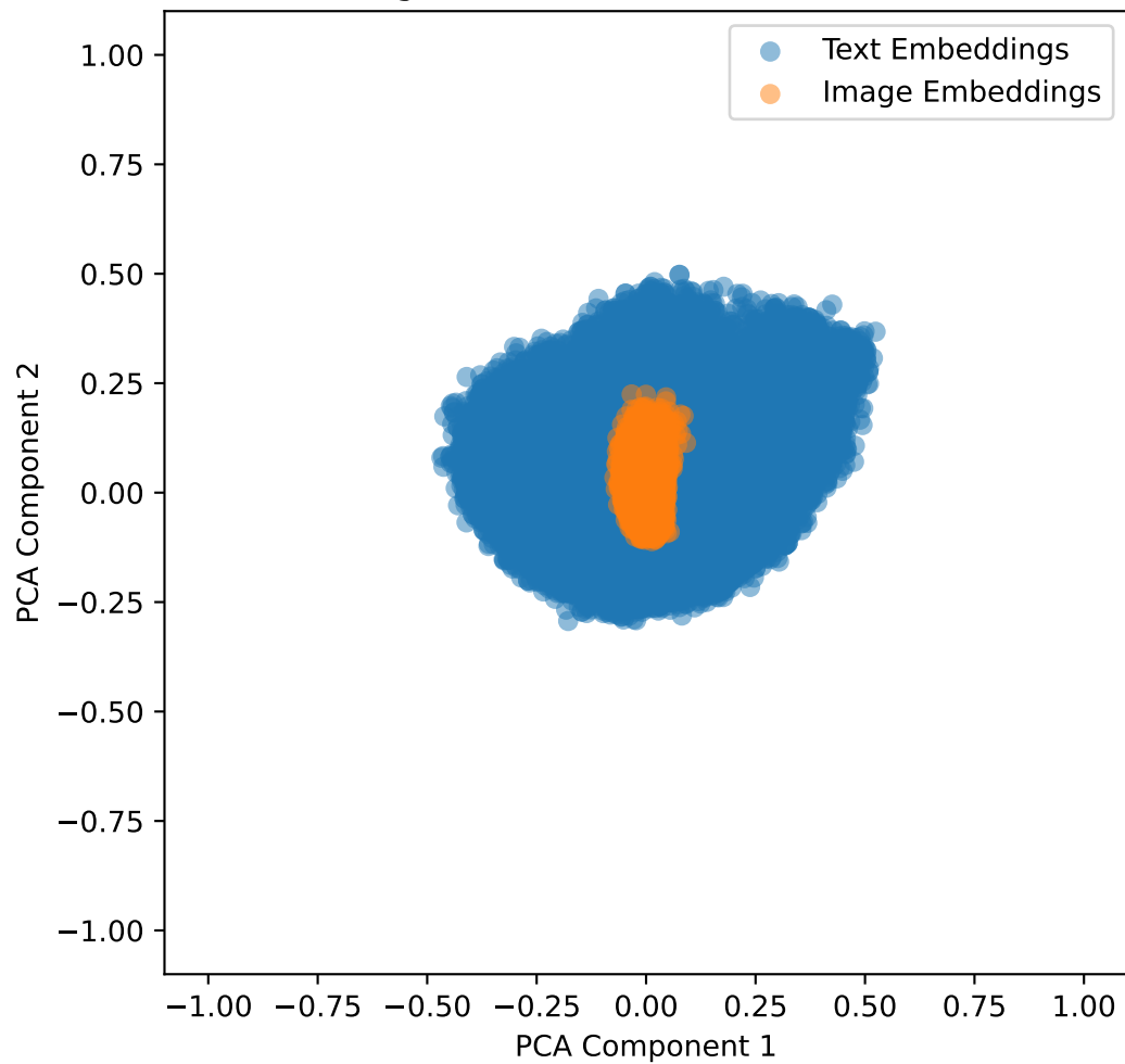
Embeddings with Lambda Shift 1 for mimic in 2D
