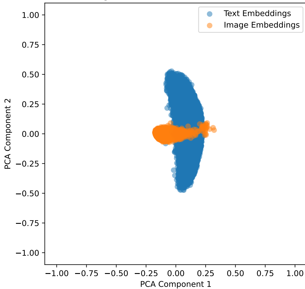
Embeddings with Lambda Shift 0.8 for mimic in 2D
