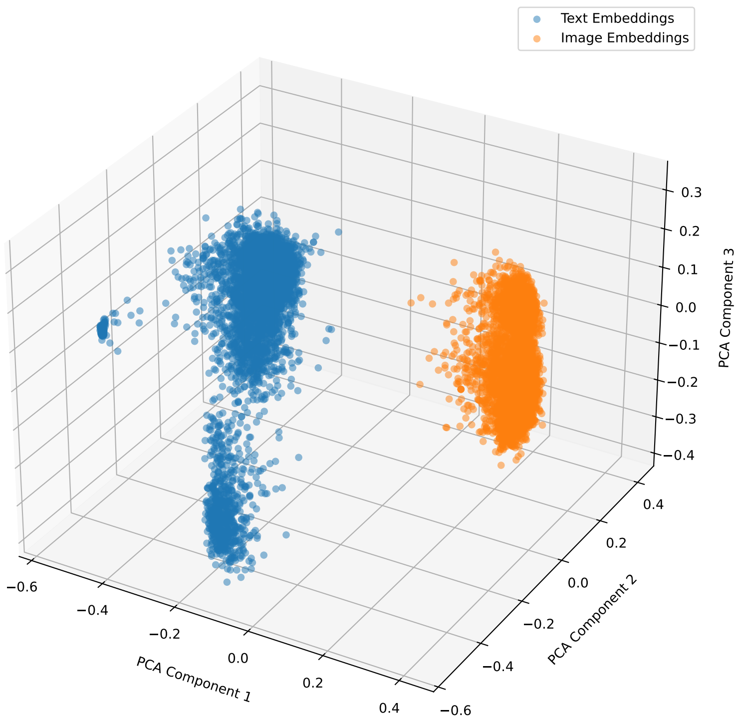
Embeddings with Lambda Shift 0.5 for Recipes5k in 3D
