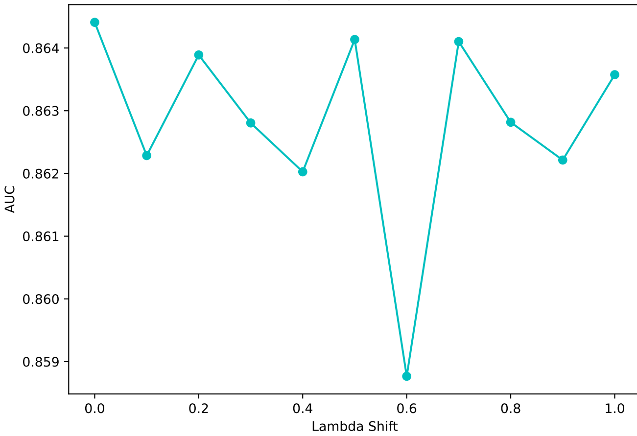
Early Fusion AUC - mimic
