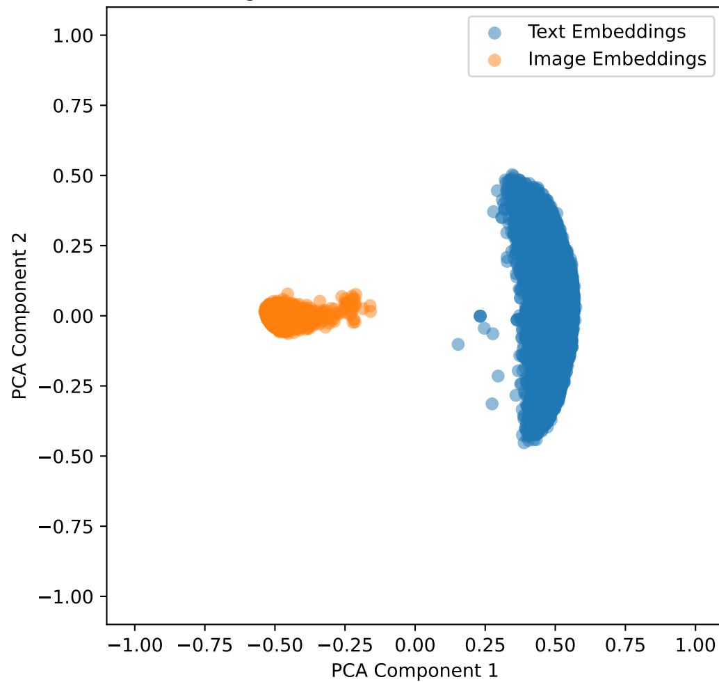
Embeddings with Lambda Shift 0.1 for mimic in 2D
