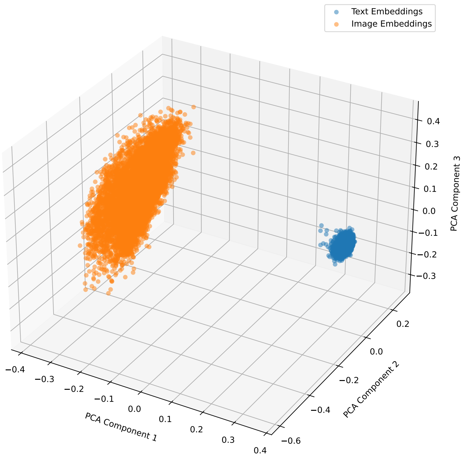
Embeddings with Lambda Shift 0.4 for brset in 3D
