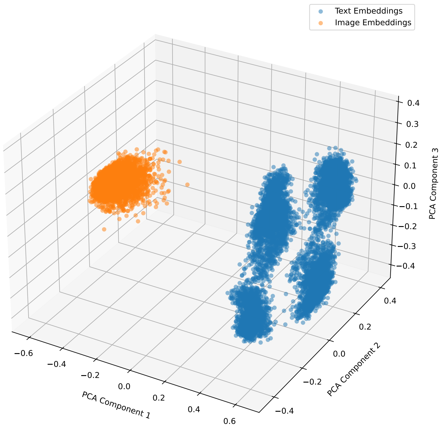
Embeddings with Lambda Shift 0.0 for ham10000 in 3D
