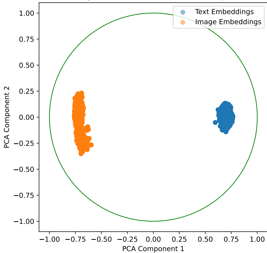
Embeddings with Lambda Shift -0.7 for daquar in 2D
