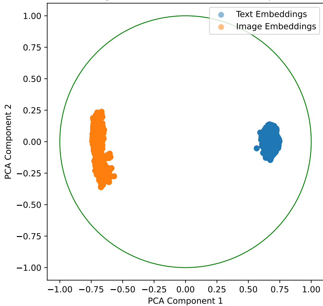
Embeddings with Lambda Shift -0.6 for daquar in 2D
