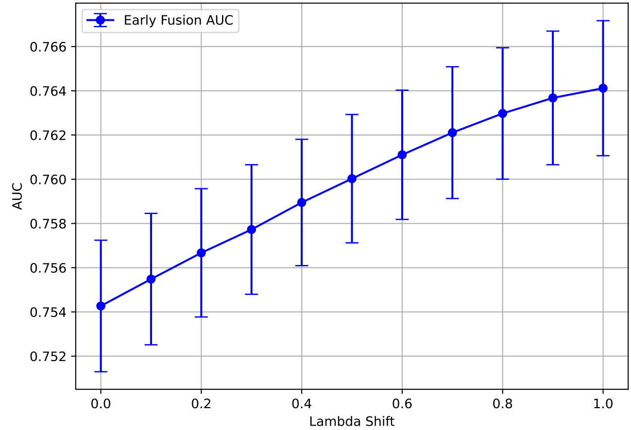
Early Fusion AUC - mbrset
