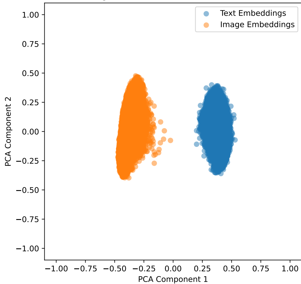
Embeddings with Lambda Shift 0.2 for mimic in 2D
