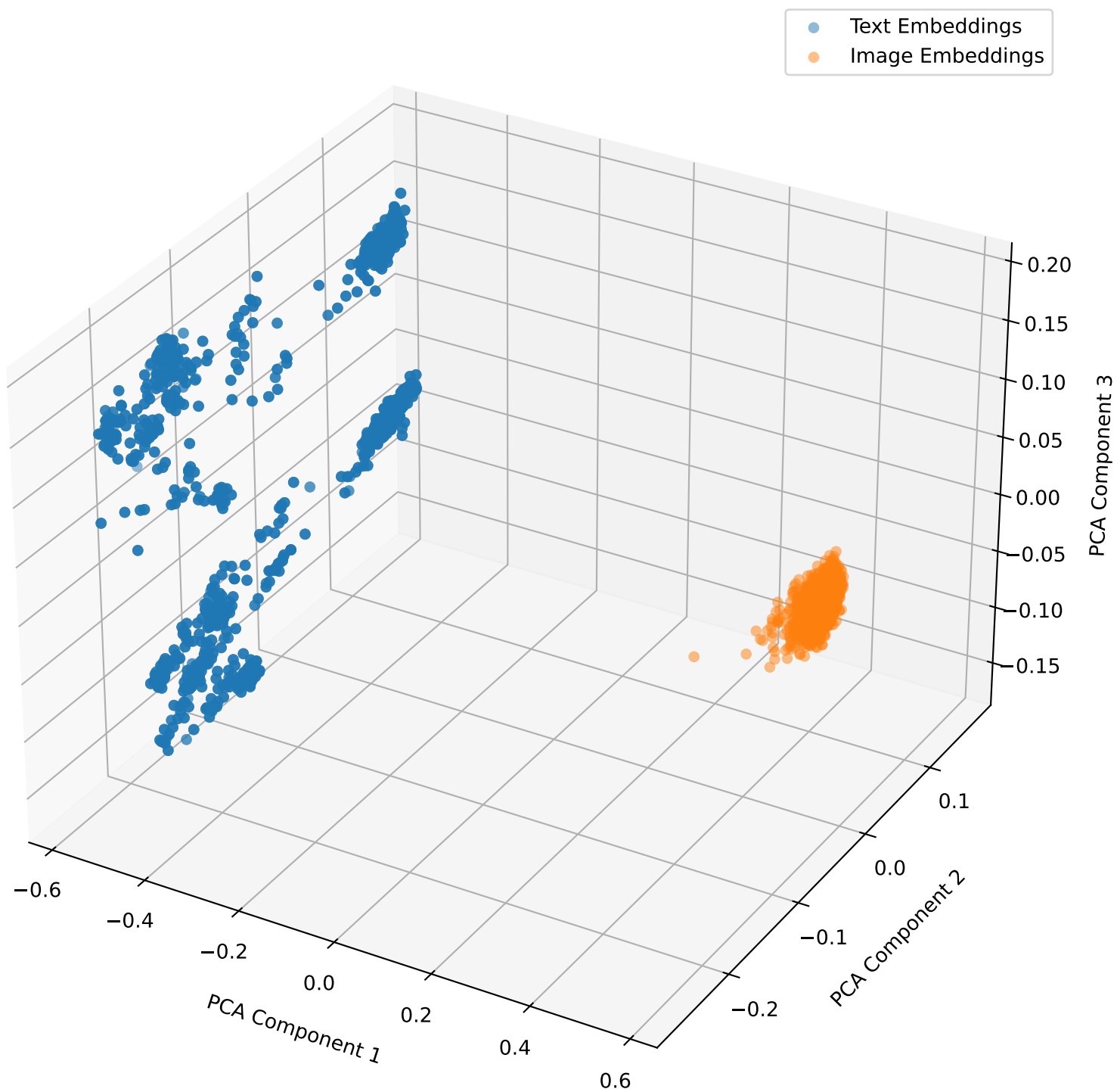
Embeddings with Lambda Shift 0.3 for mbrset in 3D
