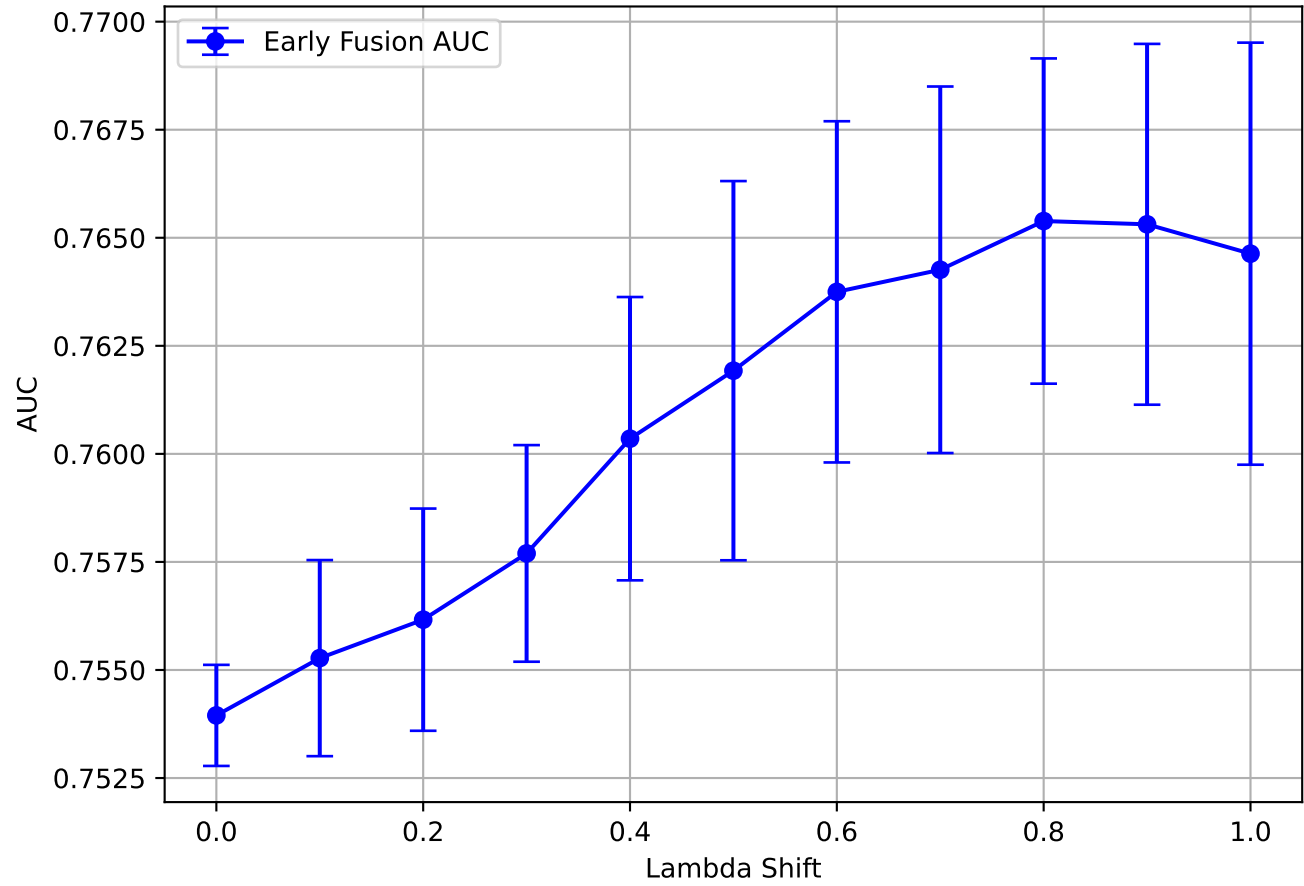
Early Fusion AUC - ham10000
