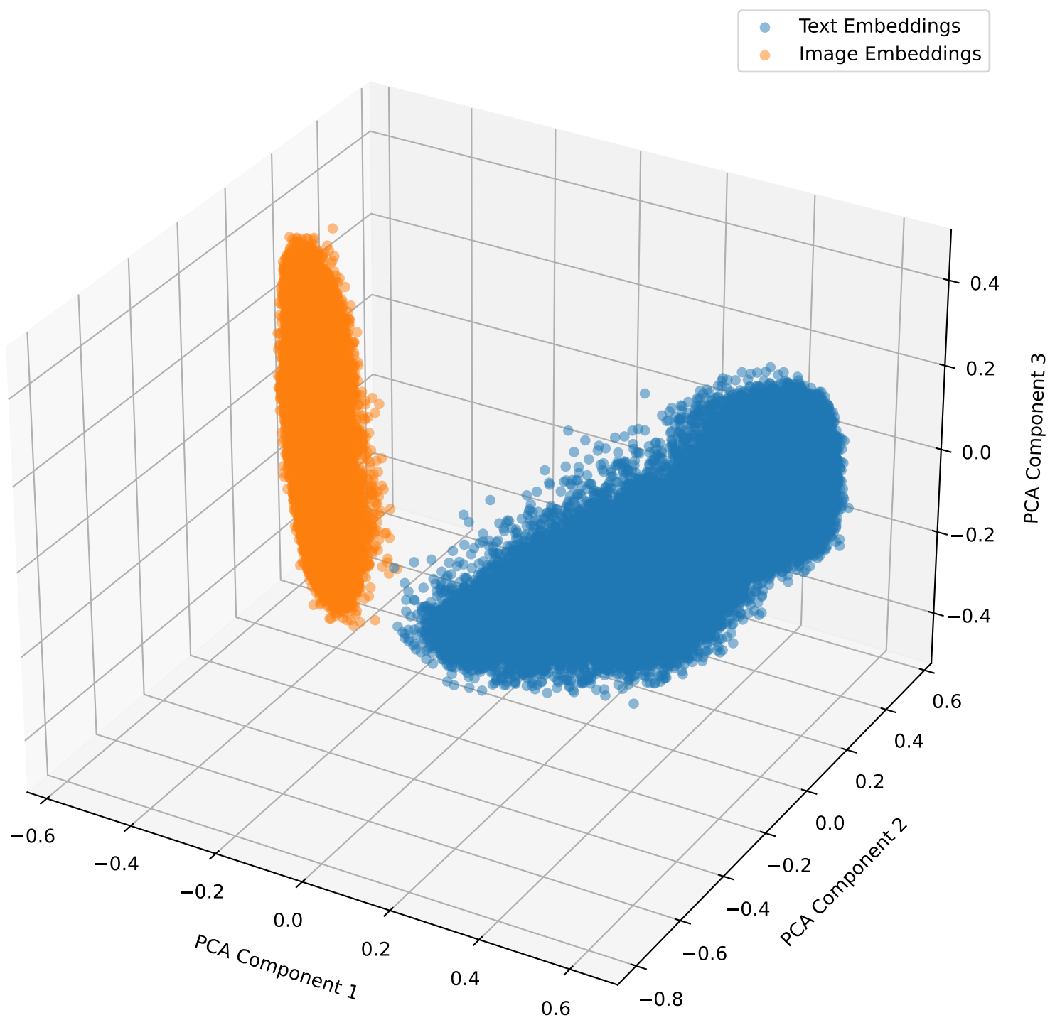
Embeddings with Lambda Shift 0.0 for fakeddit in 3D
