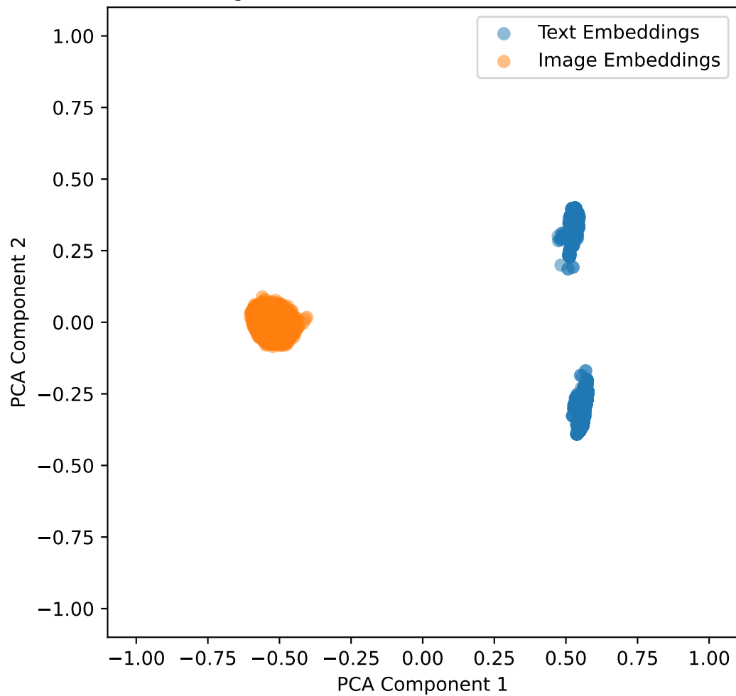
Embeddings with Lambda Shift 0 for ham10000 in 2D
