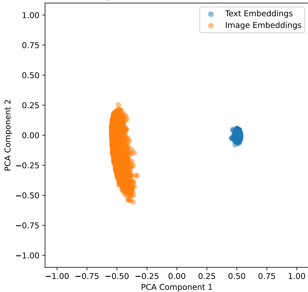
Embeddings with Lambda Shift 0.0 for brset in 2D
