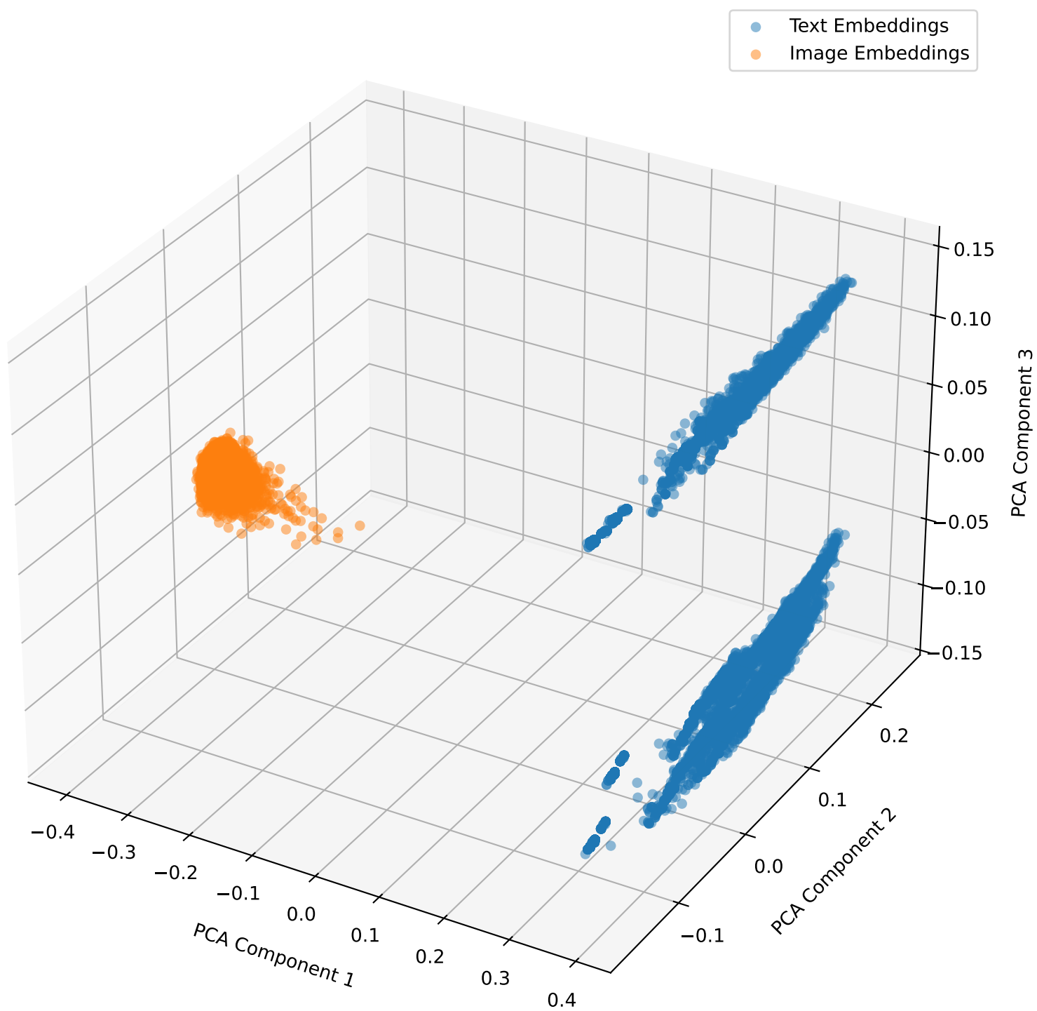
Embeddings with Lambda Shift 0.4 for brset in 3D
