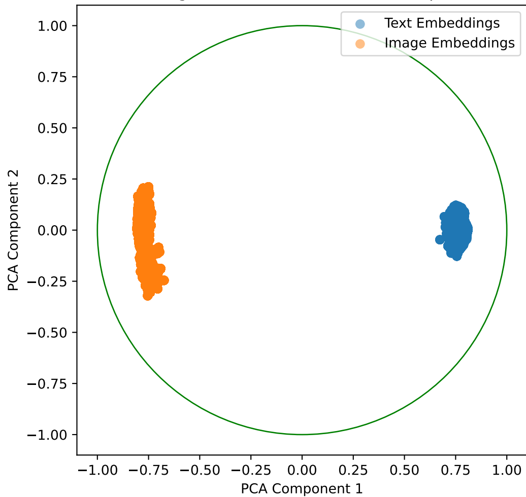
Embeddings with Lambda Shift -1 for daquar in 2D
