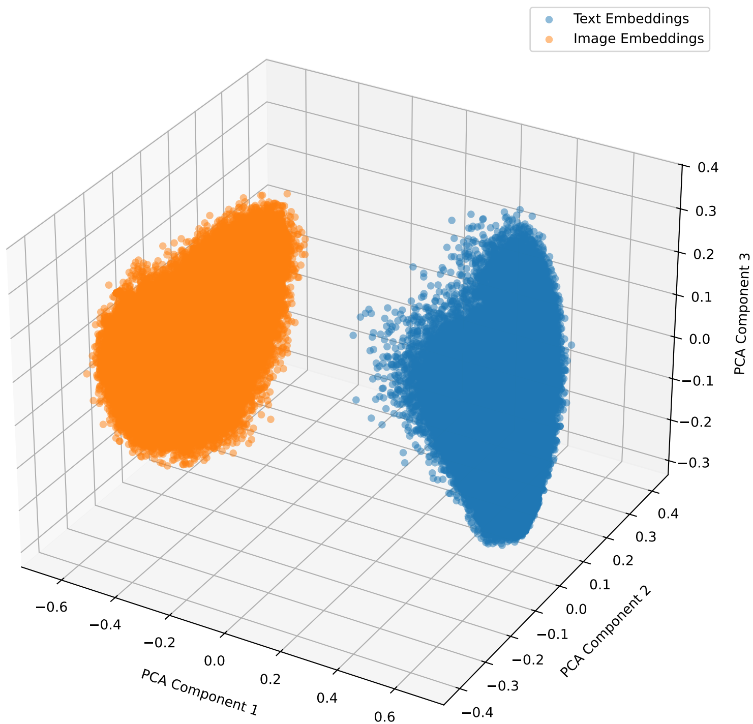
Embeddings with Lambda Shift -0.5 for fakeddit in 3D
