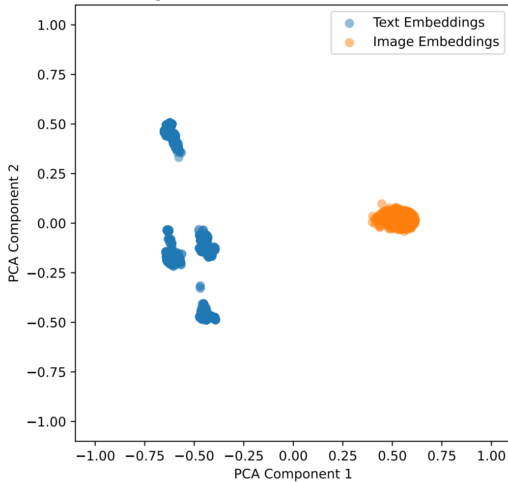
Embeddings with Lambda Shift 0.2 for ham10000 in 2D
