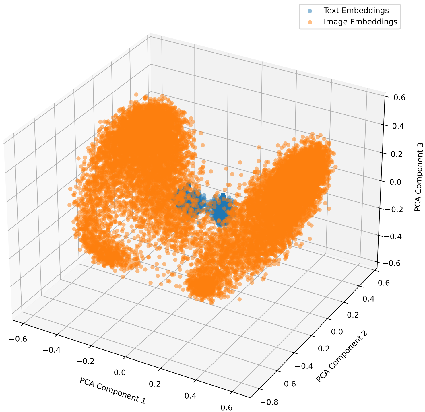
Embeddings with Lambda Shift 0.9 for brset in 3D
