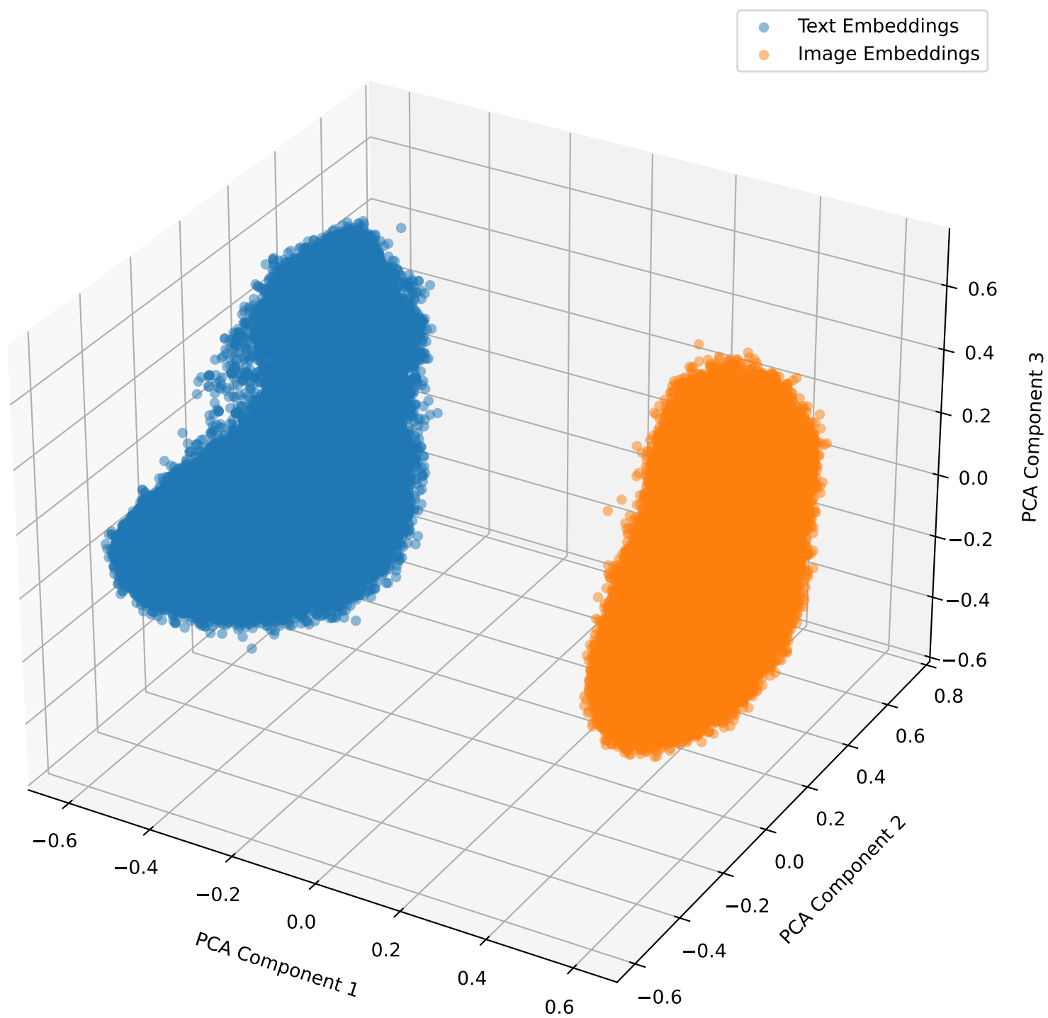
Embeddings with Lambda Shift 0 for mimic in 3D
