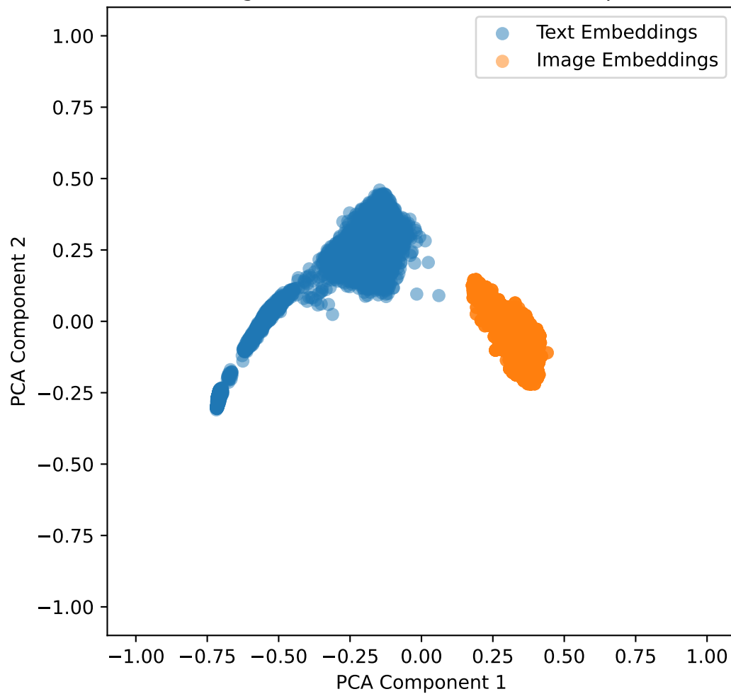
Embeddings with Lambda Shift 0.5 for daquar in 2D
