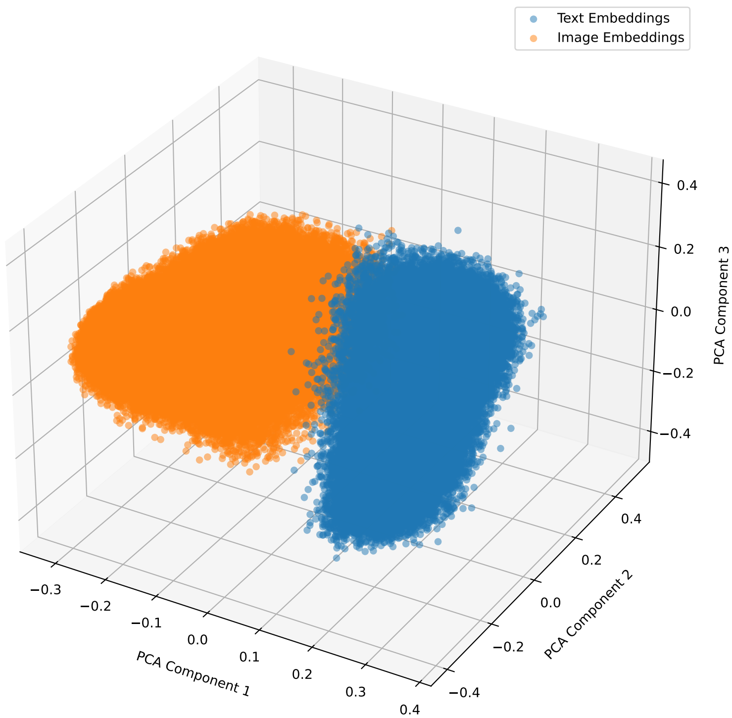
Embeddings with Lambda Shift 0.6 for mimic in 3D
