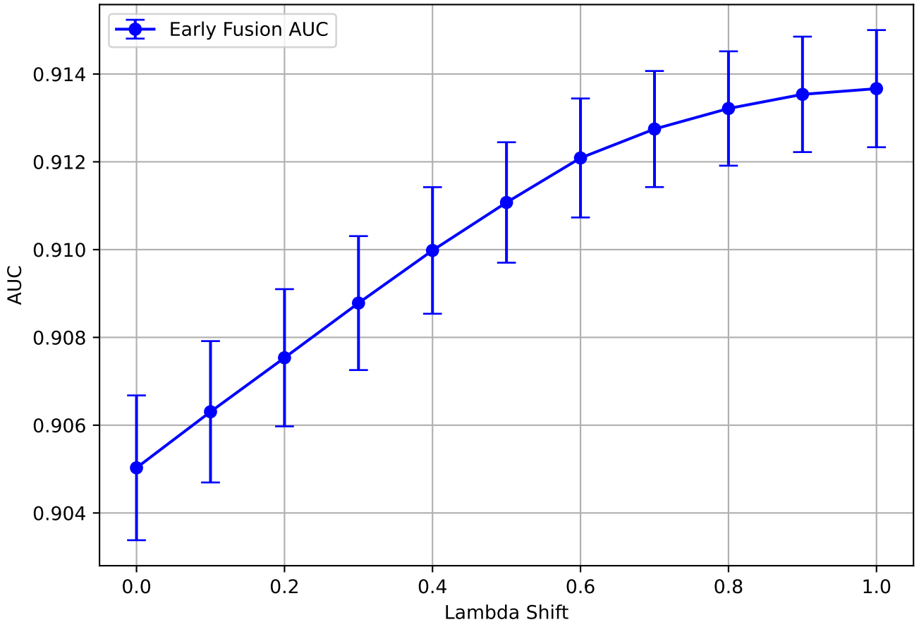
Early Fusion AUC - brset
