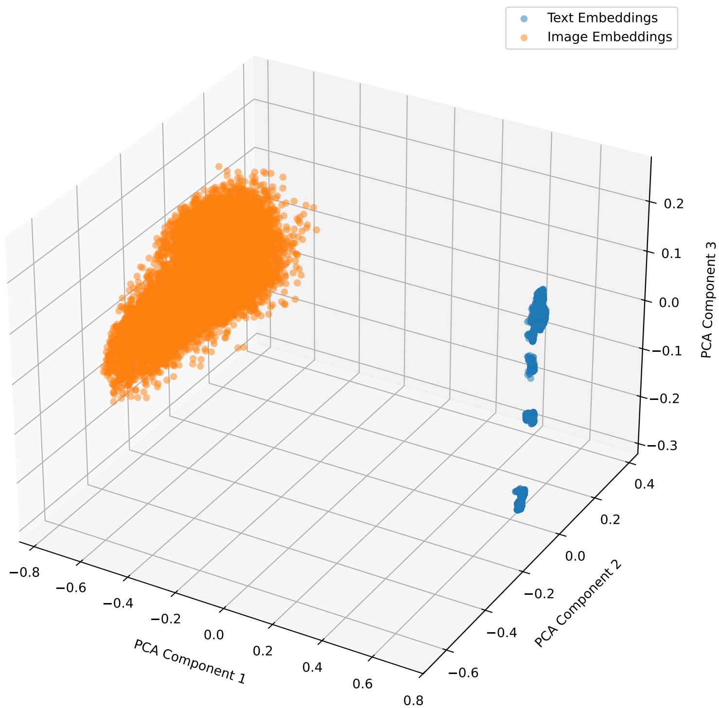
Embeddings with Lambda Shift 0 for ham10000 in 3D
