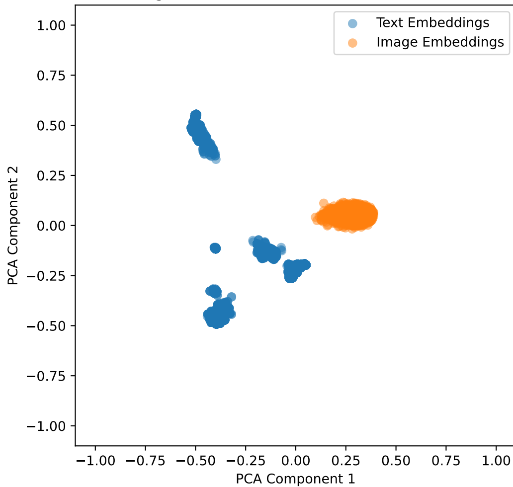
Embeddings with Lambda Shift 0.6 for ham10000 in 2D
