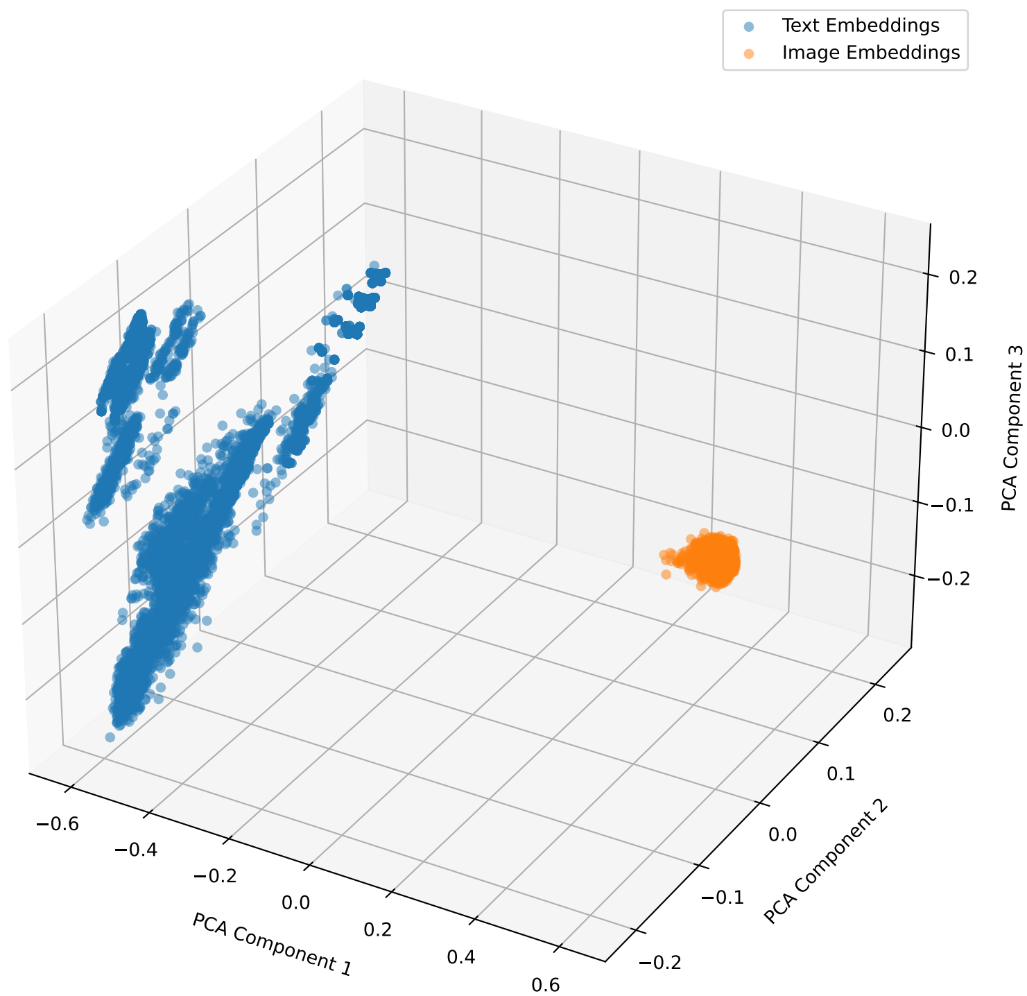
Embeddings with Lambda Shift 0.1 for brset in 3D
