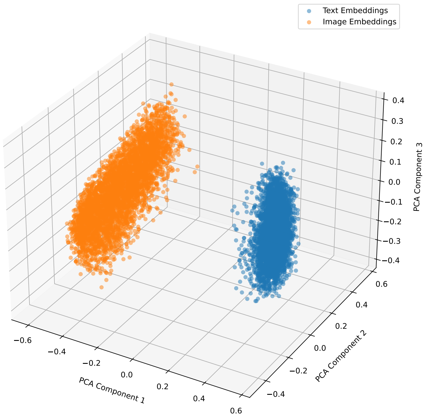
Embeddings with Lambda Shift 0.0 for Recipes5k in 3D
