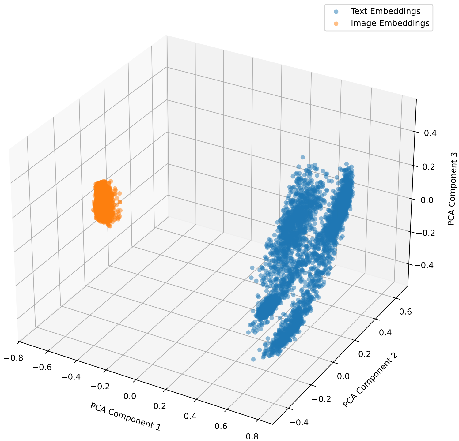
Embeddings with Lambda Shift -0.5 for Recipes5k in 3D
