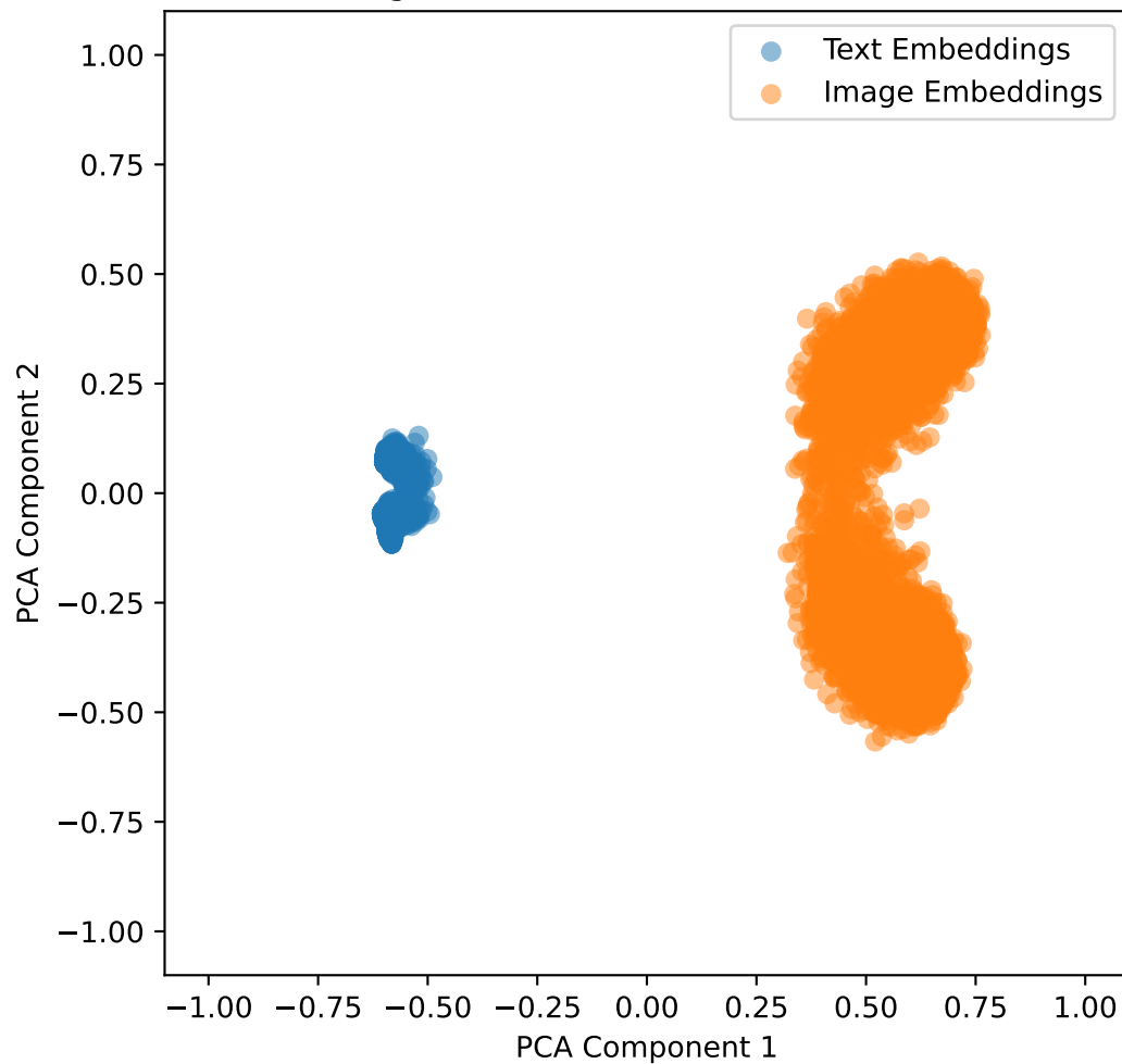
Embeddings with Lambda Shift 0.1 for brset in 2D
