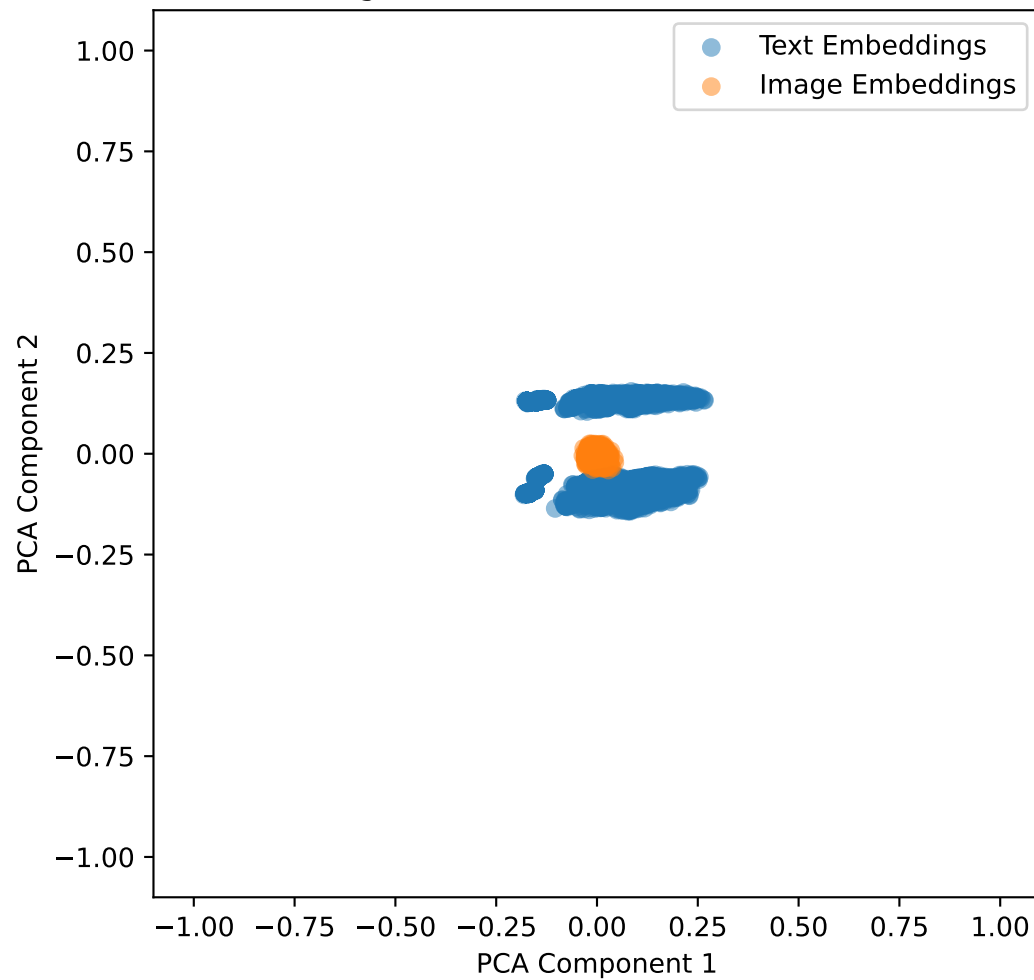
Embeddings with Lambda Shift 1.0 for brset in 2D
