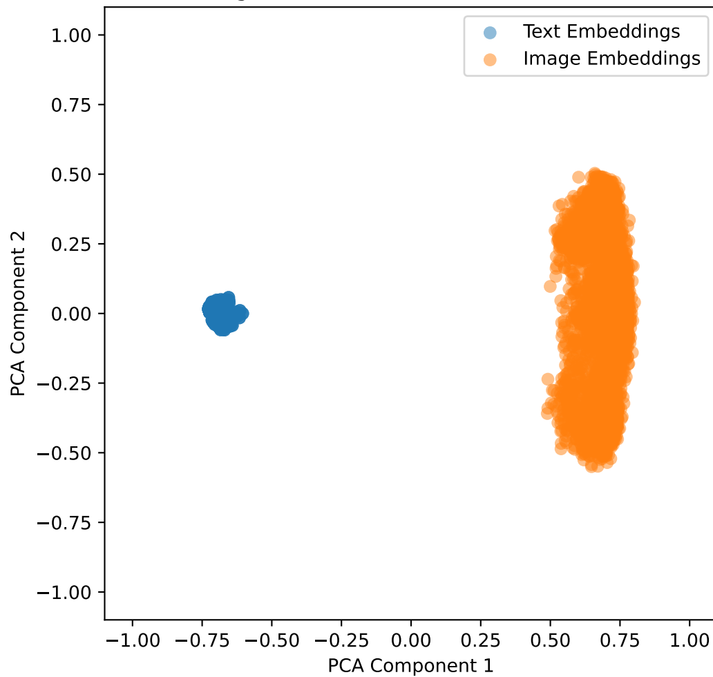
Embeddings with Lambda Shift 0.0 for mbrset in 2D
