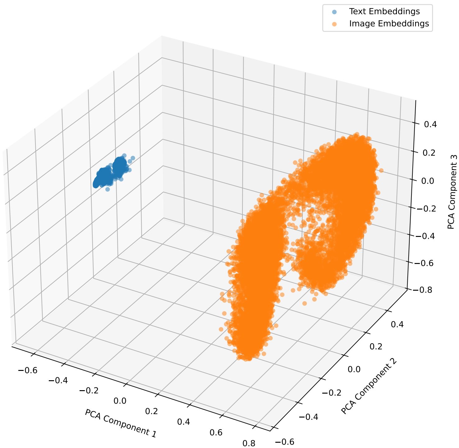
Embeddings with Lambda Shift 0.0 for brset in 3D
