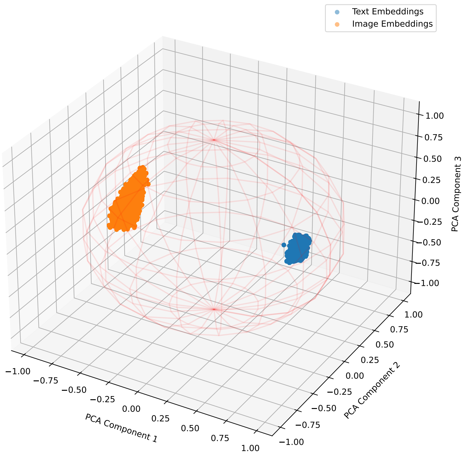
Embeddings with Lambda Shift -0.8 for daquar in 3D
