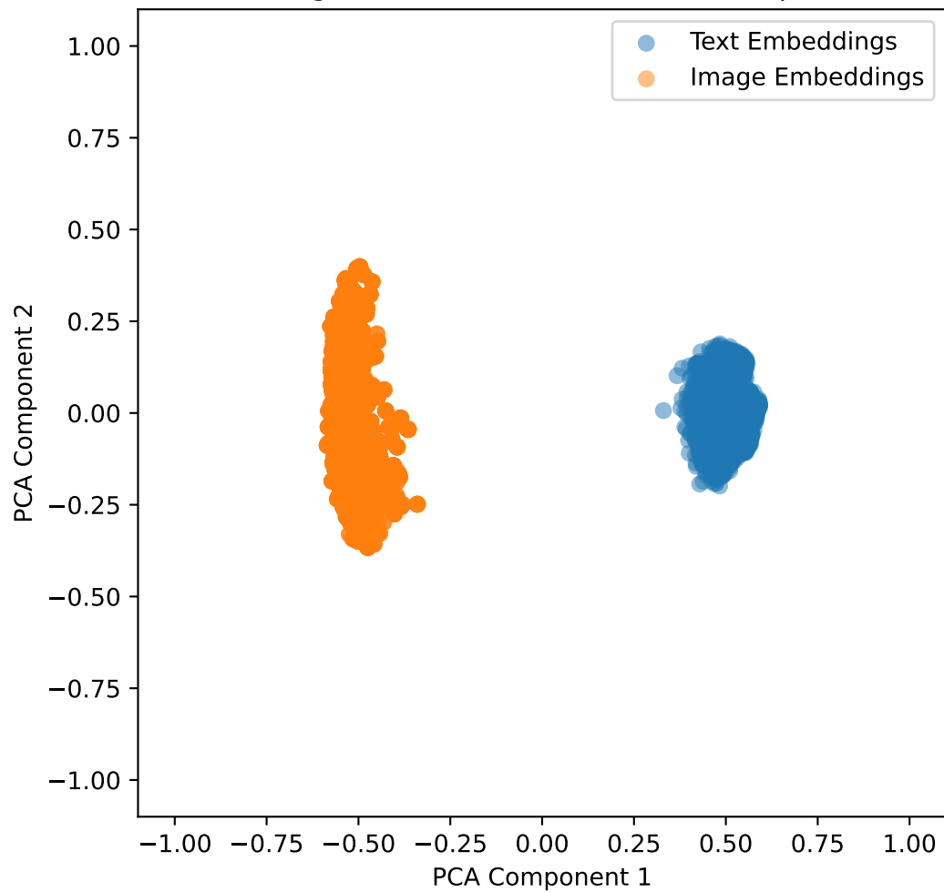
Embeddings with Lambda Shift 0.0 for daquar in 2D
