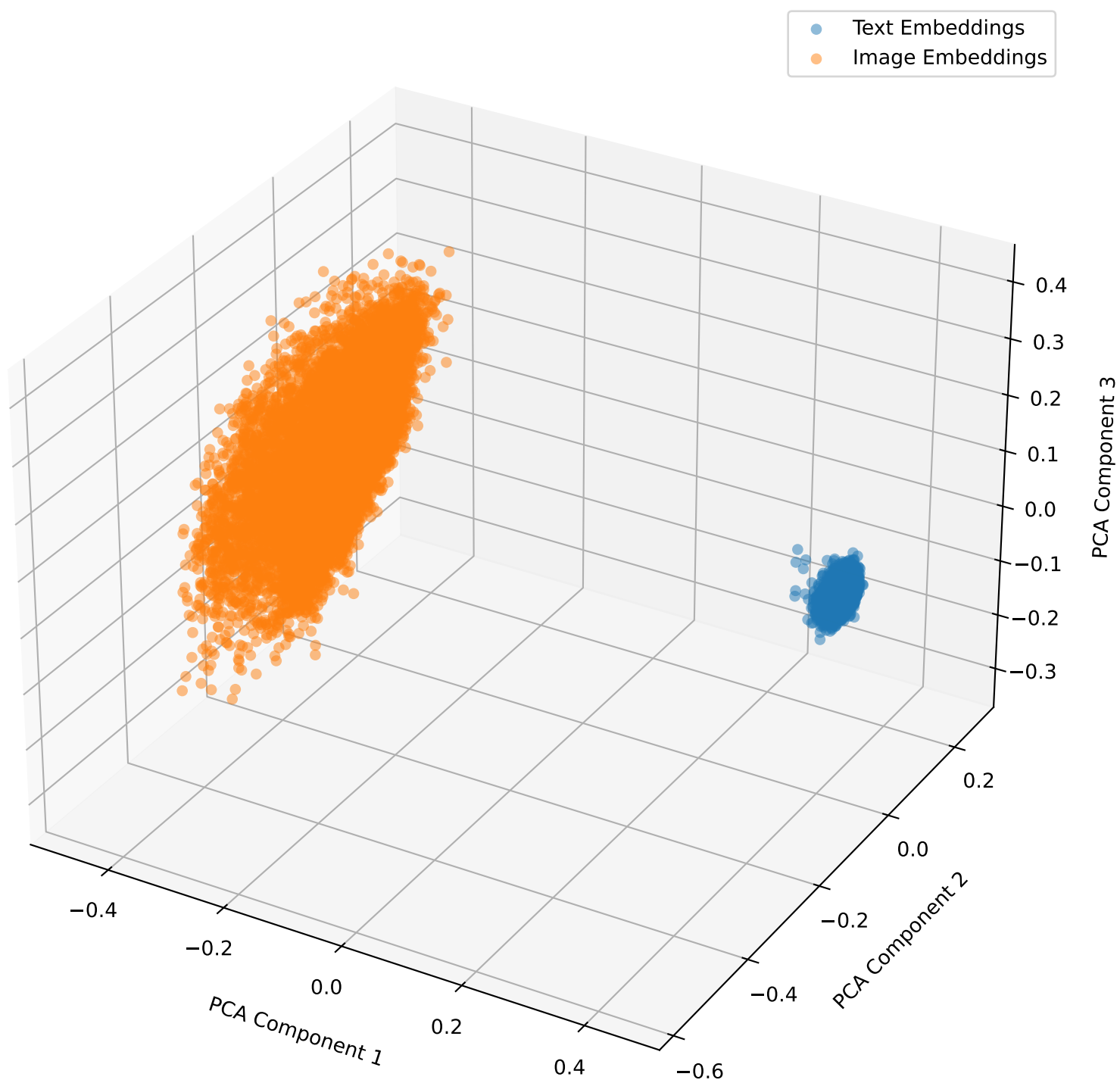
Embeddings with Lambda Shift 0.2 for brset in 3D
