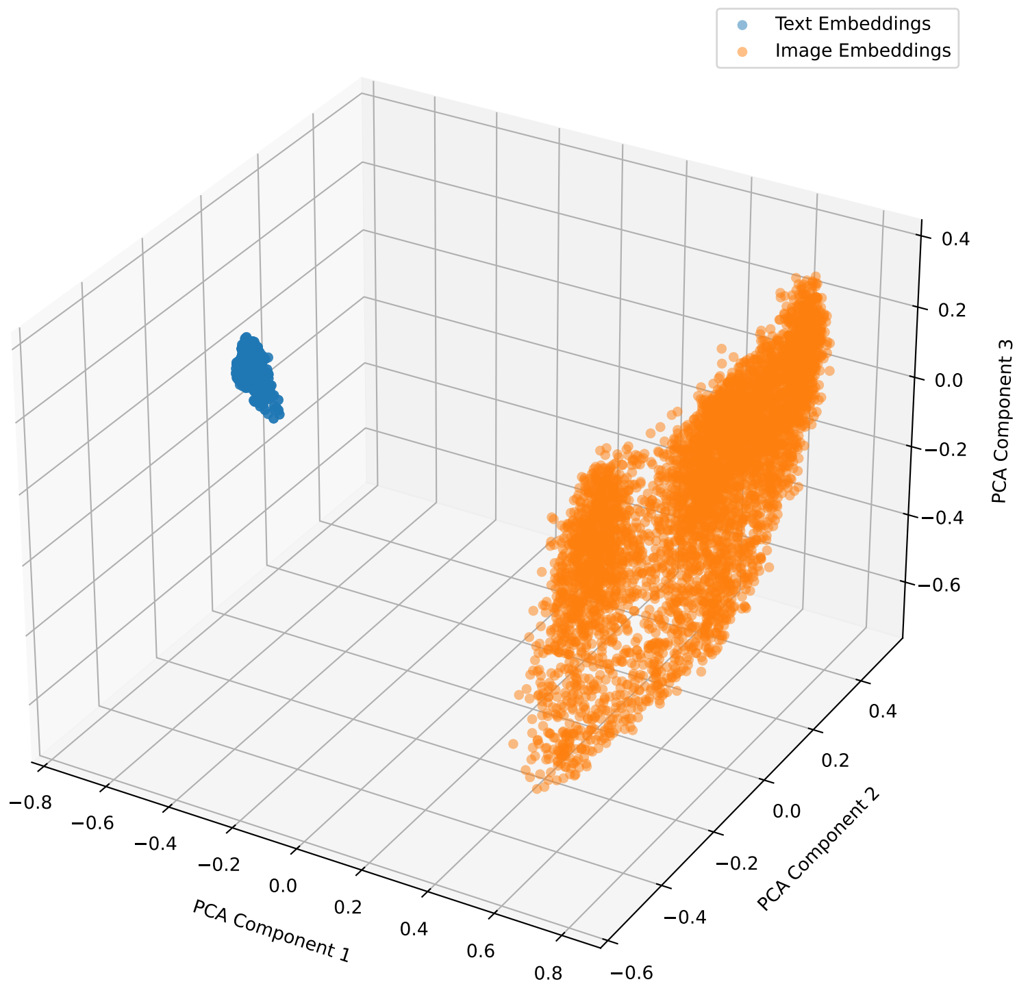
Embeddings with Lambda Shift 0.0 for mbrset in 3D
