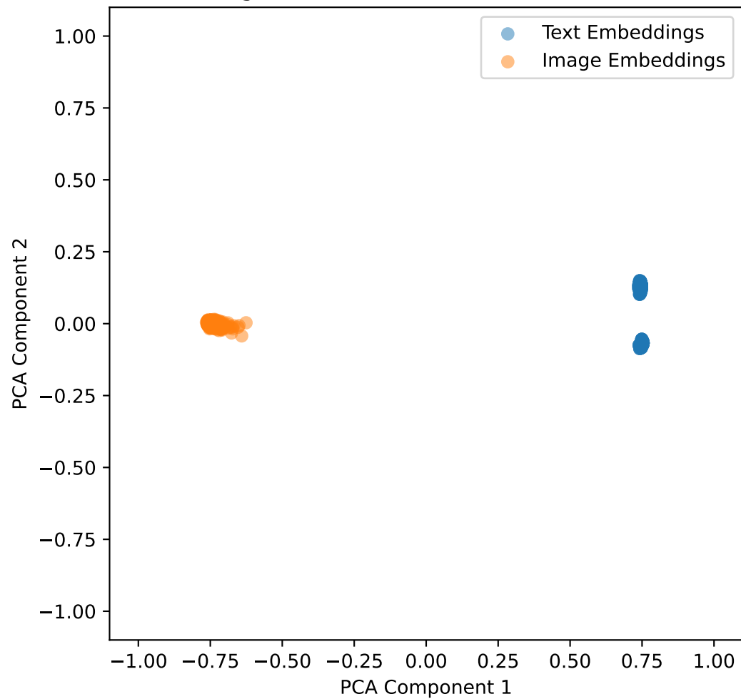
Embeddings with Lambda Shift -0.5 for mbrset in 2D
