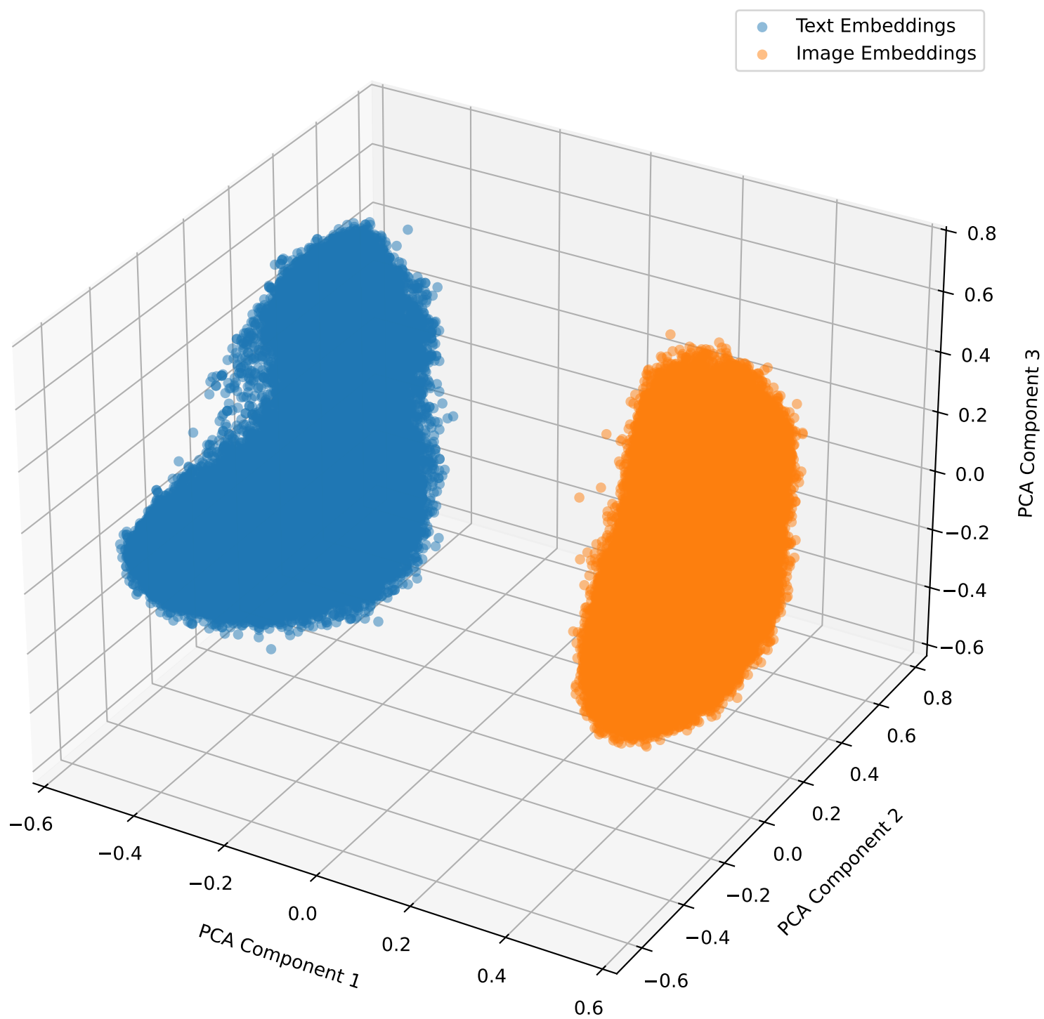
Embeddings with Lambda Shift 0.2 for mimic in 3D
