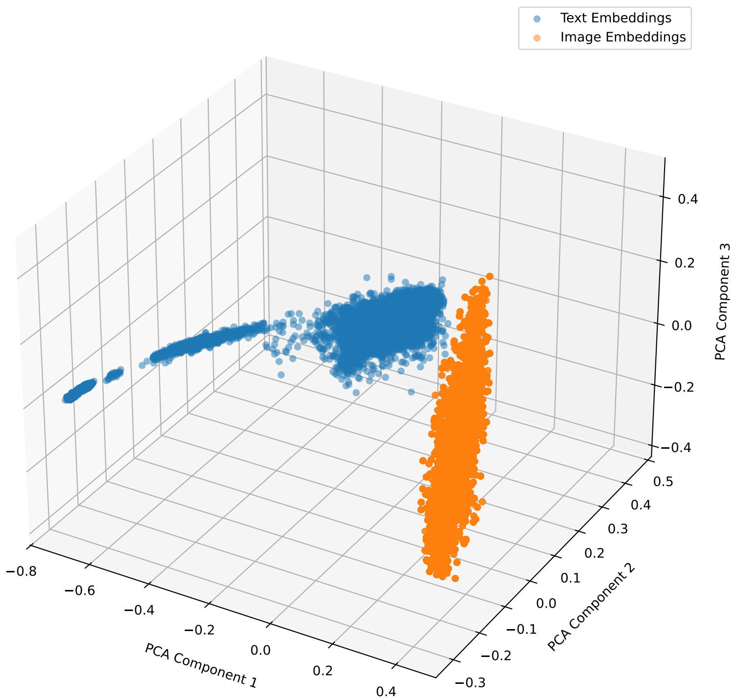
Embeddings with Lambda Shift 0.5 for daquar in 3D
