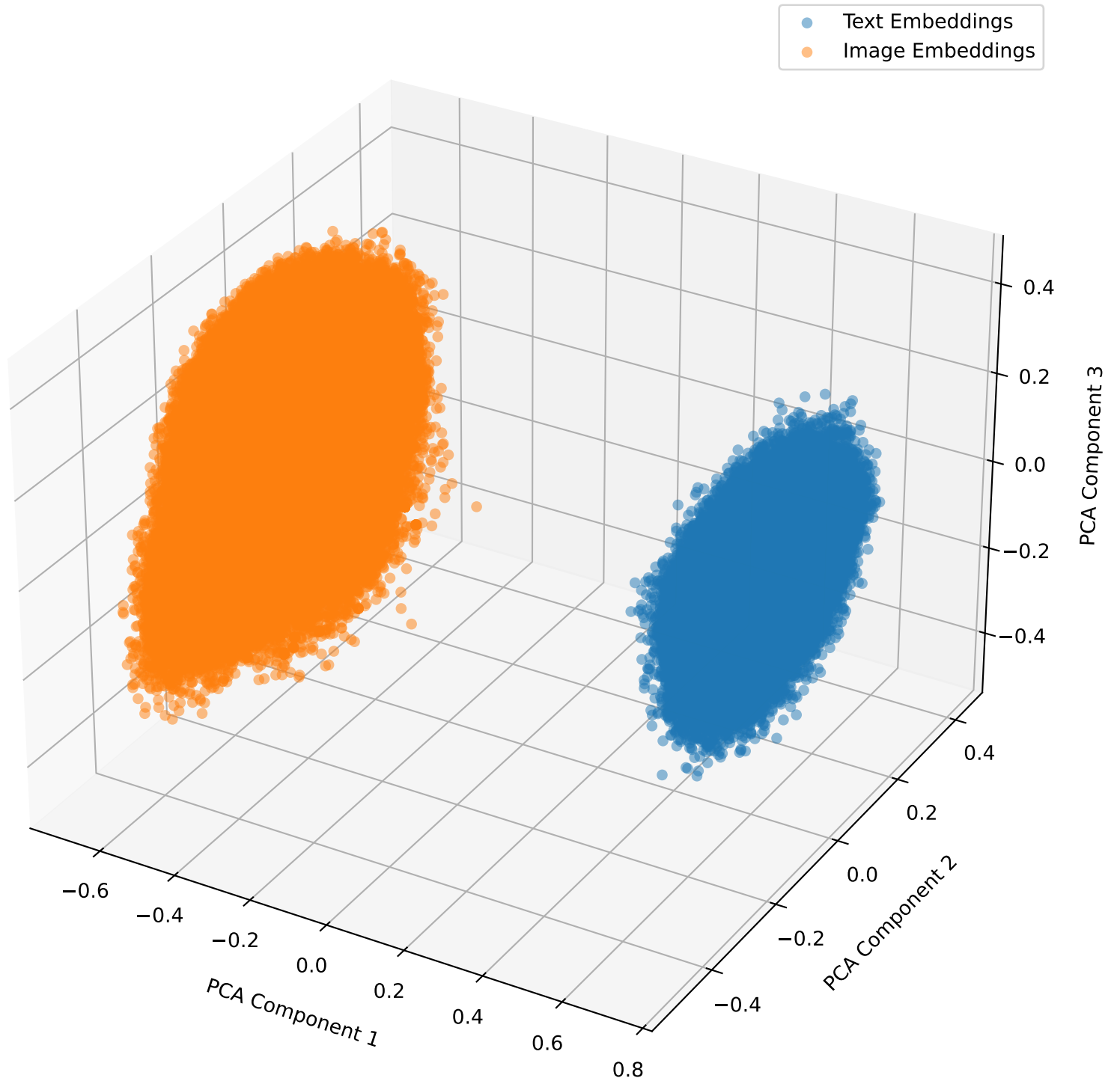
Embeddings with Lambda Shift -1.0 for fakeddit in 3D
