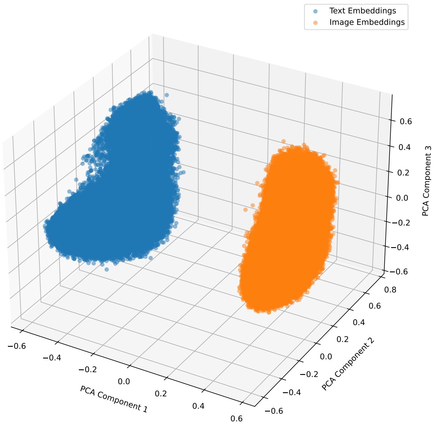
Embeddings with Lambda Shift 0.1 for mimic in 3D
