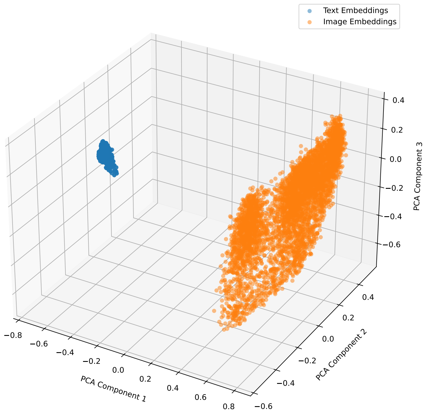
Embeddings with Lambda Shift 0 for mbrset in 3D
