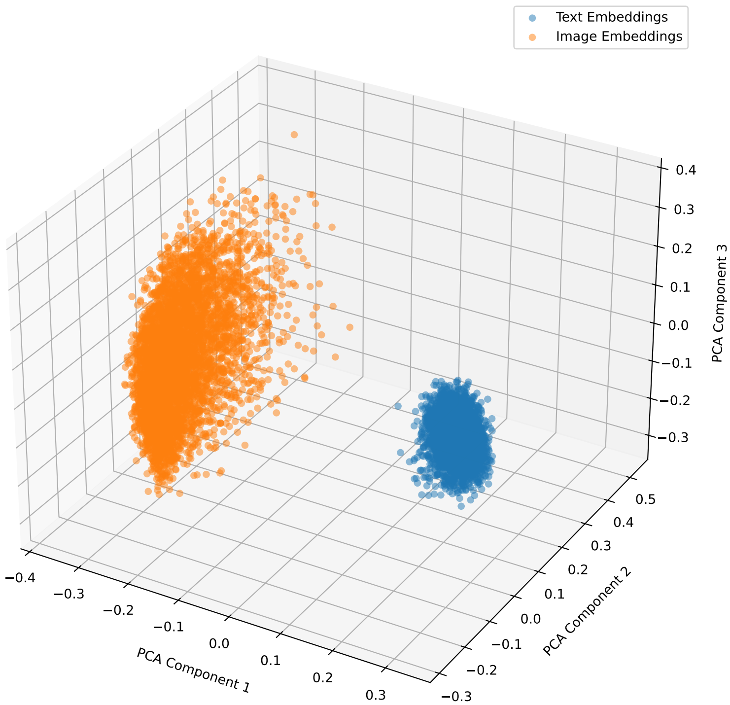
Embeddings with Lambda Shift 0.6 for mbrset in 3D
