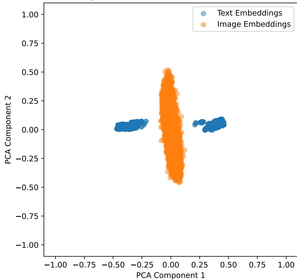
Embeddings with Lambda Shift 0.8 for ham10000 in 2D
