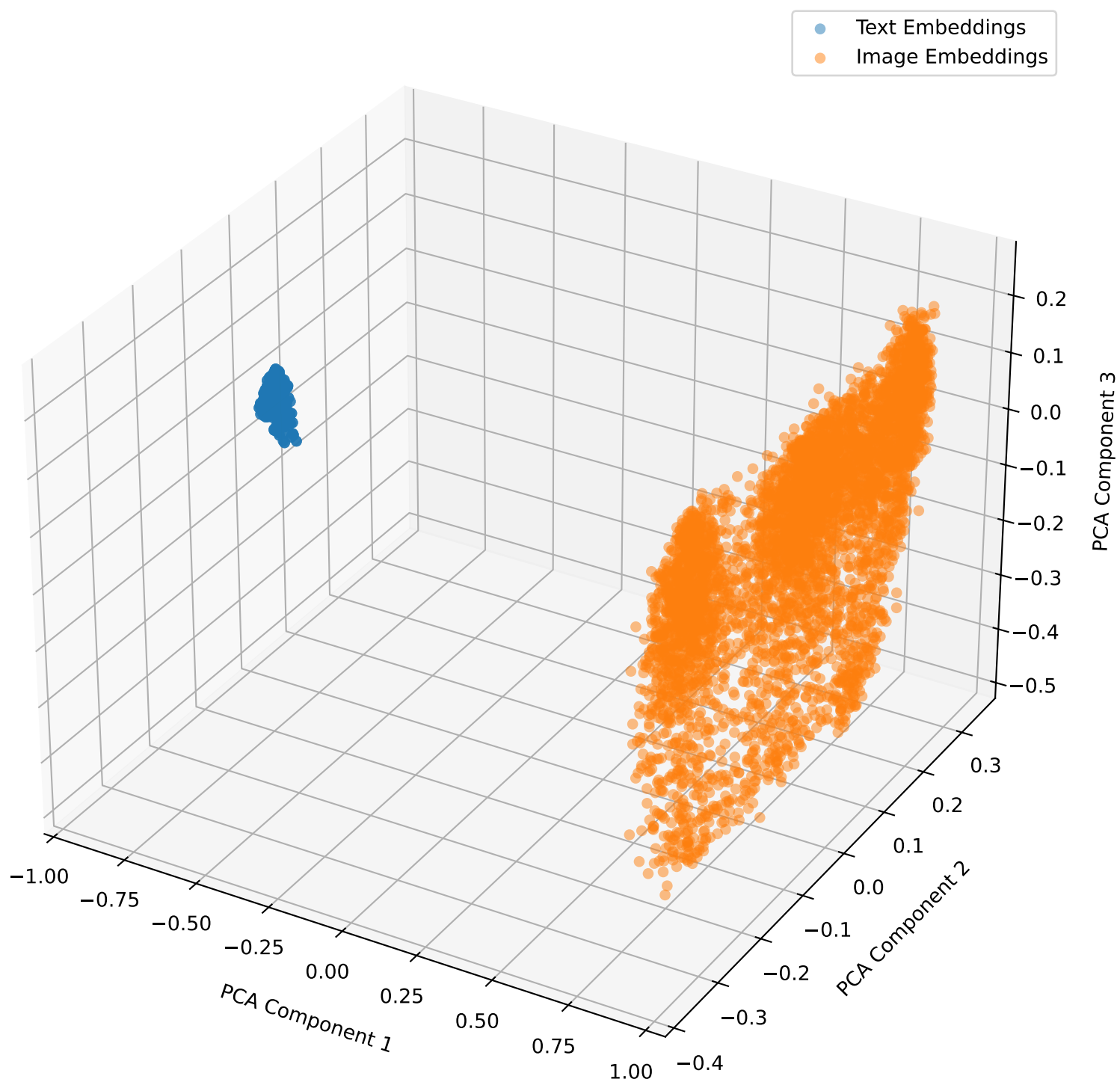
Embeddings with Lambda Shift -1.0 for mbrset in 3D
