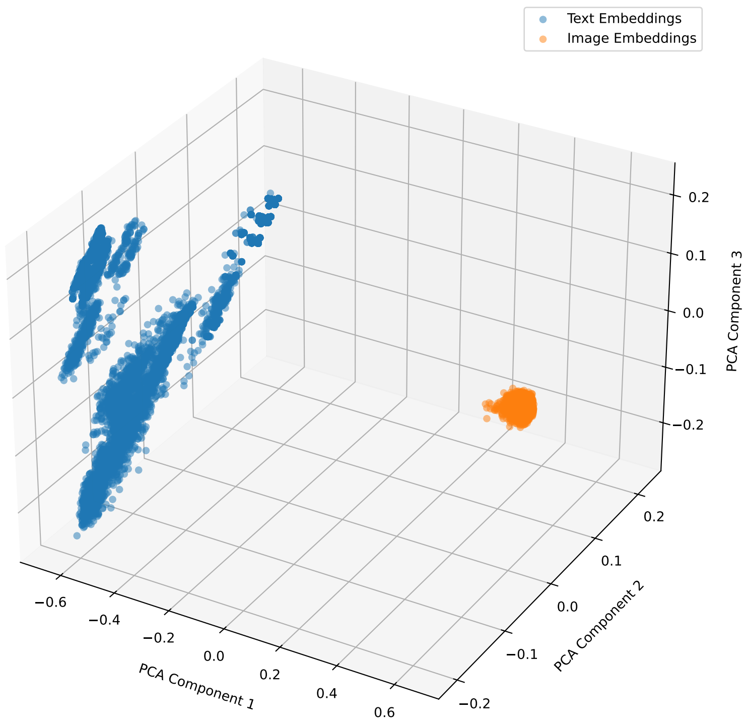
Embeddings with Lambda Shift 0.0 for brset in 3D
