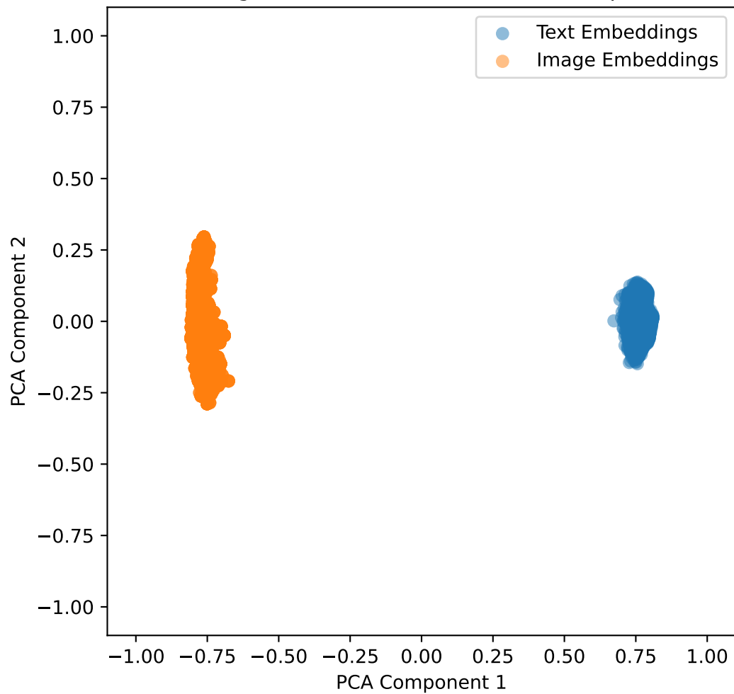
Embeddings with Lambda Shift -1.0 for daquar in 2D
