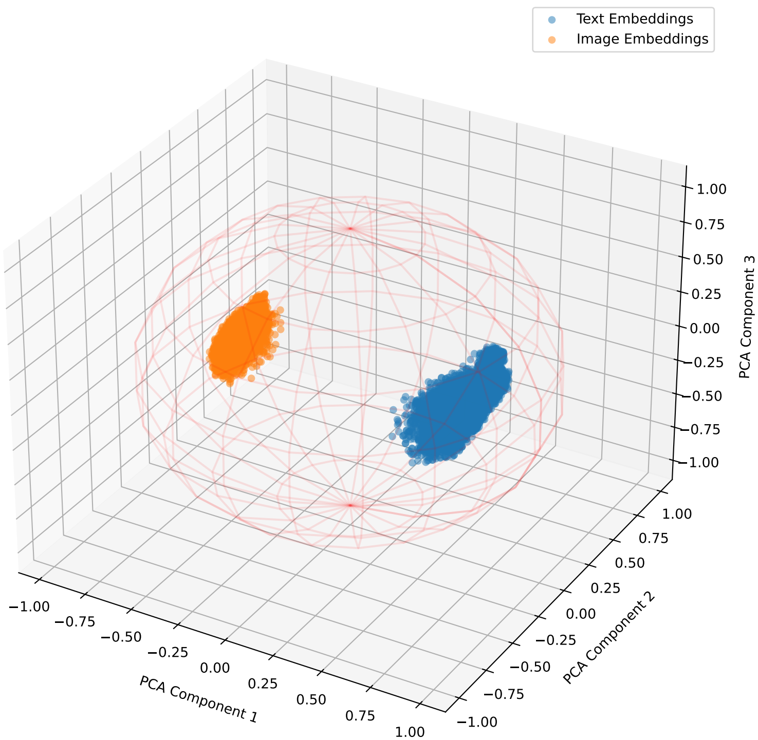
Embeddings with Lambda Shift -0.4 for Recipes5k in 3D
