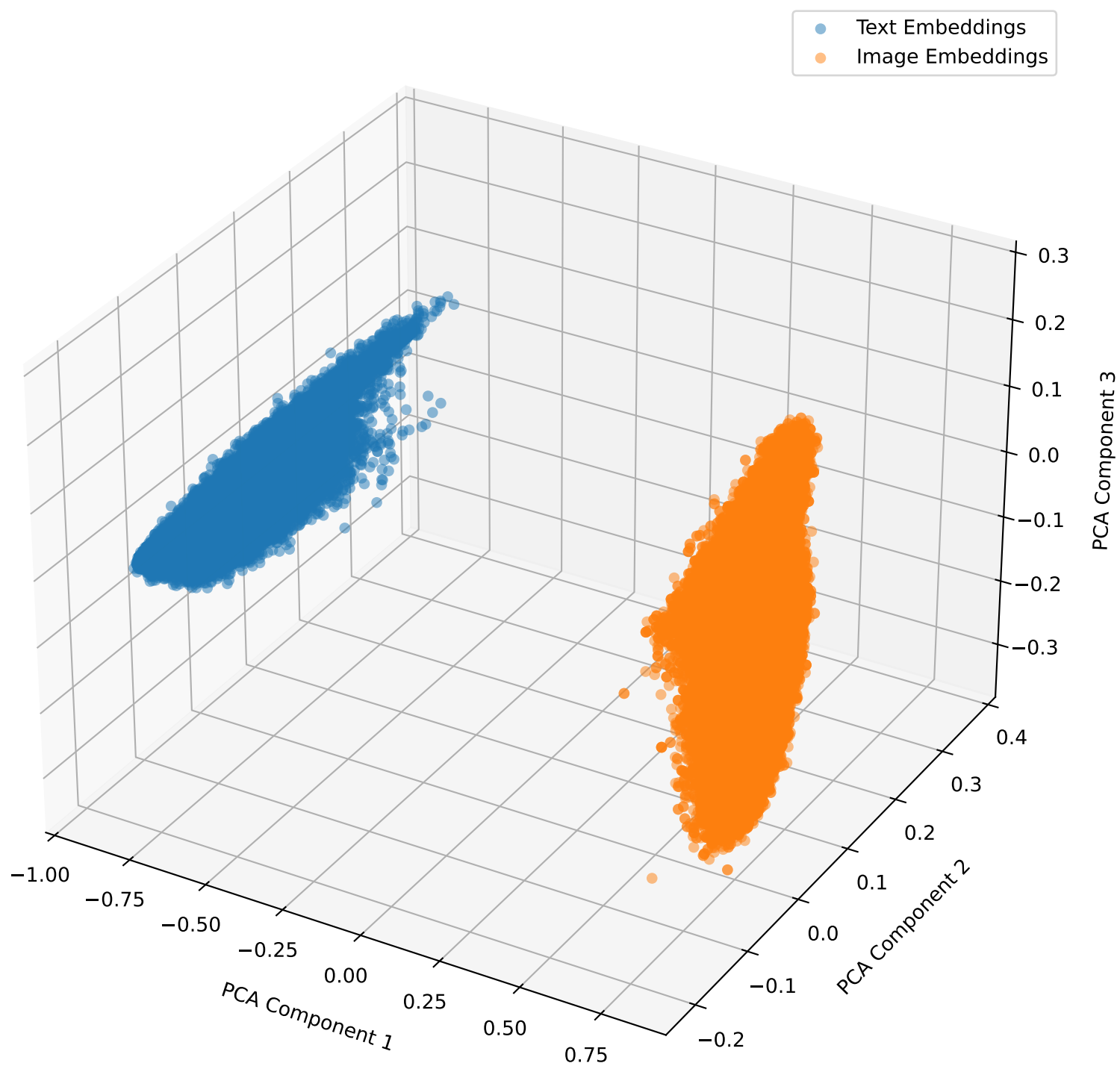
Embeddings with Lambda Shift -1.0 for coco-qa in 3D
