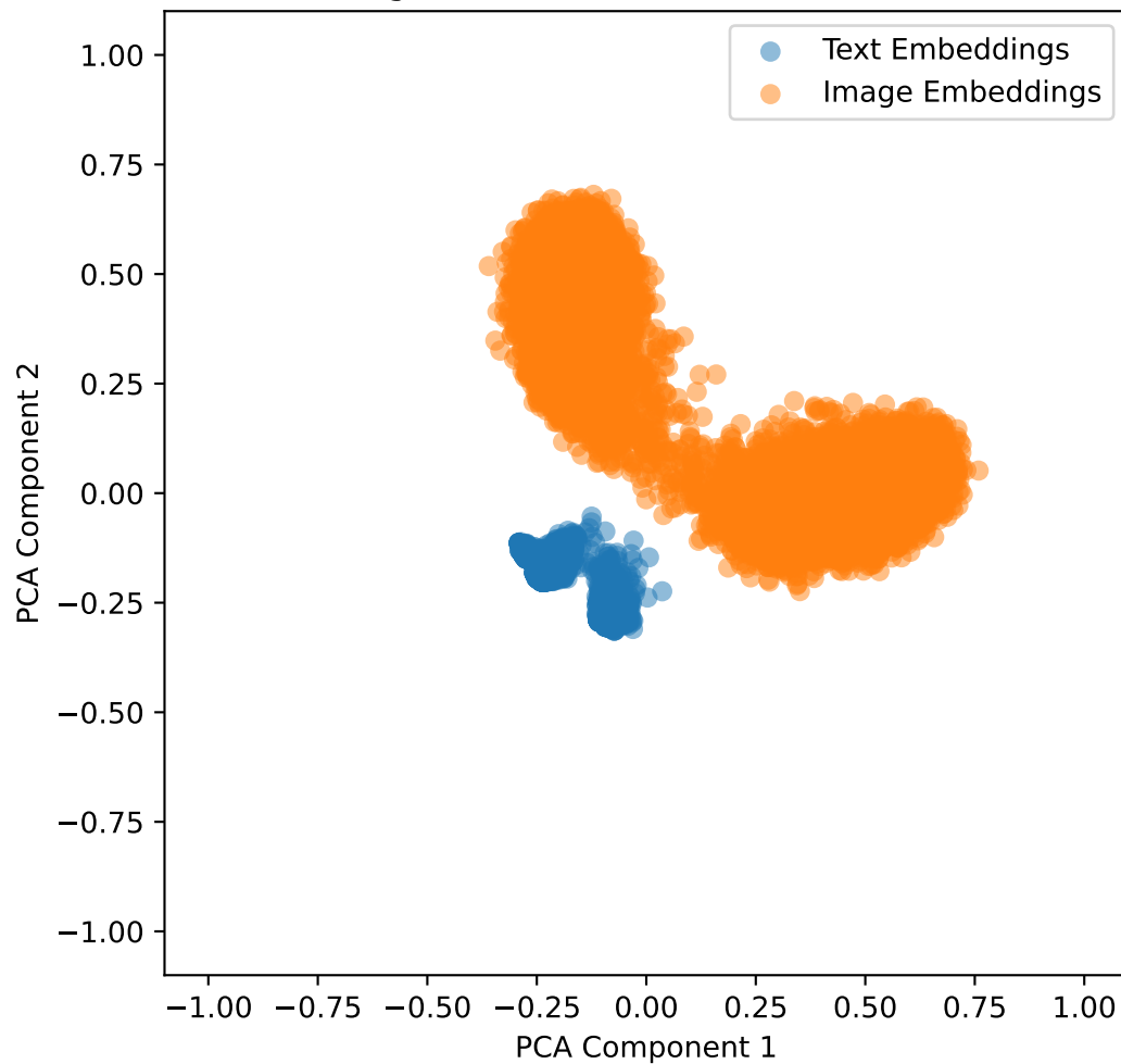
Embeddings with Lambda Shift 0.7 for brset in 2D
