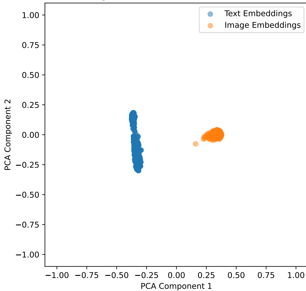
Embeddings with Lambda Shift 0.6 for mbrset in 2D
