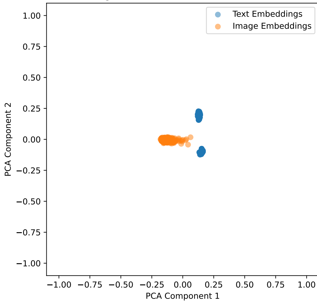
Embeddings with Lambda Shift 0.8 for mbrset in 2D
