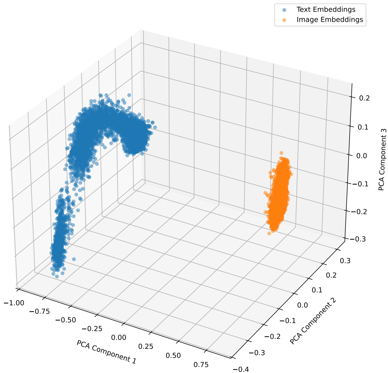
Embeddings with Lambda Shift -1.0 for Recipes5k in 3D
