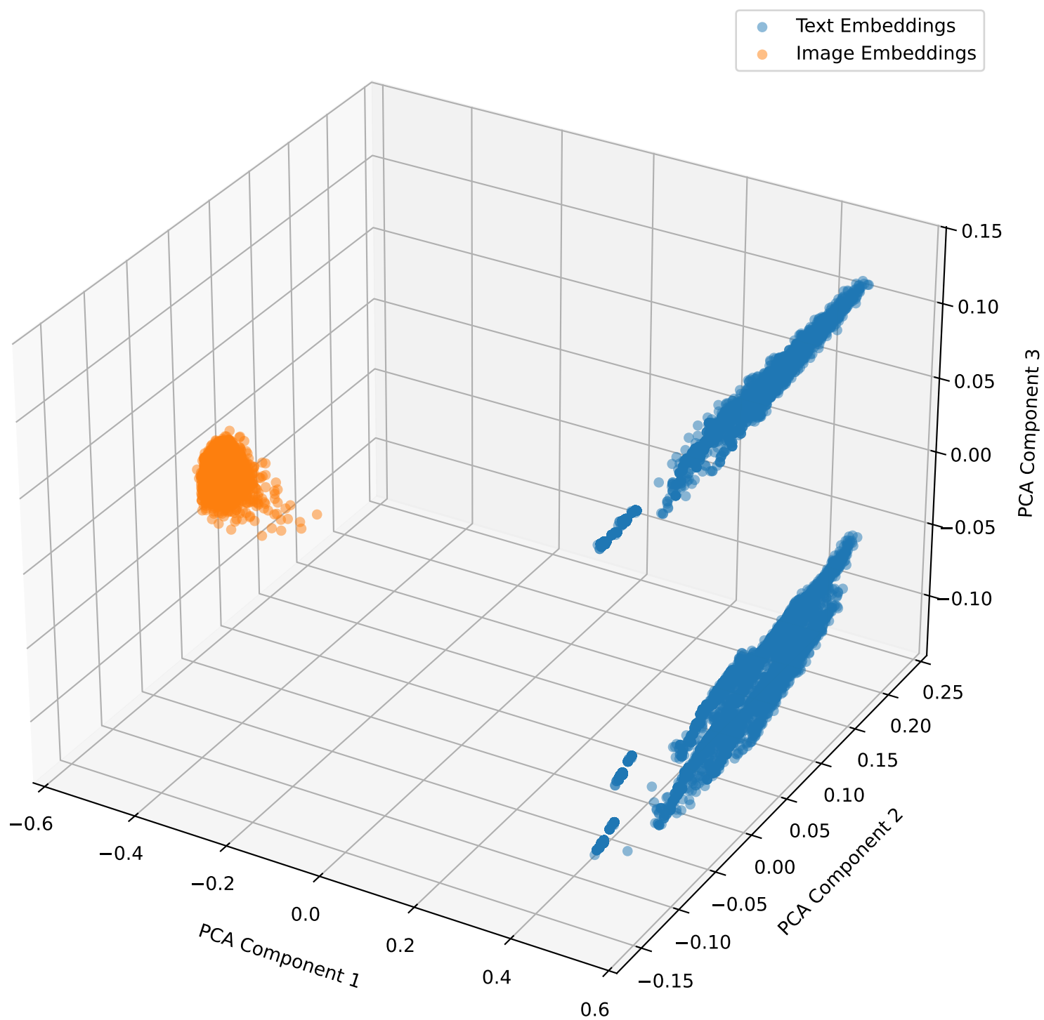
Embeddings with Lambda Shift 0.1 for brset in 3D
