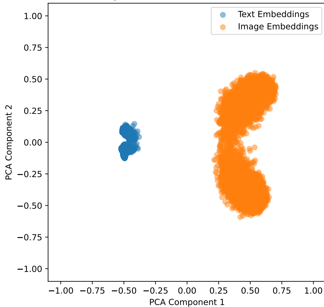
Embeddings with Lambda Shift 0.3 for brset in 2D
