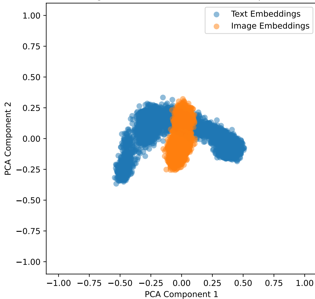
Embeddings with Lambda Shift 1.0 for Recipes5k in 2D
