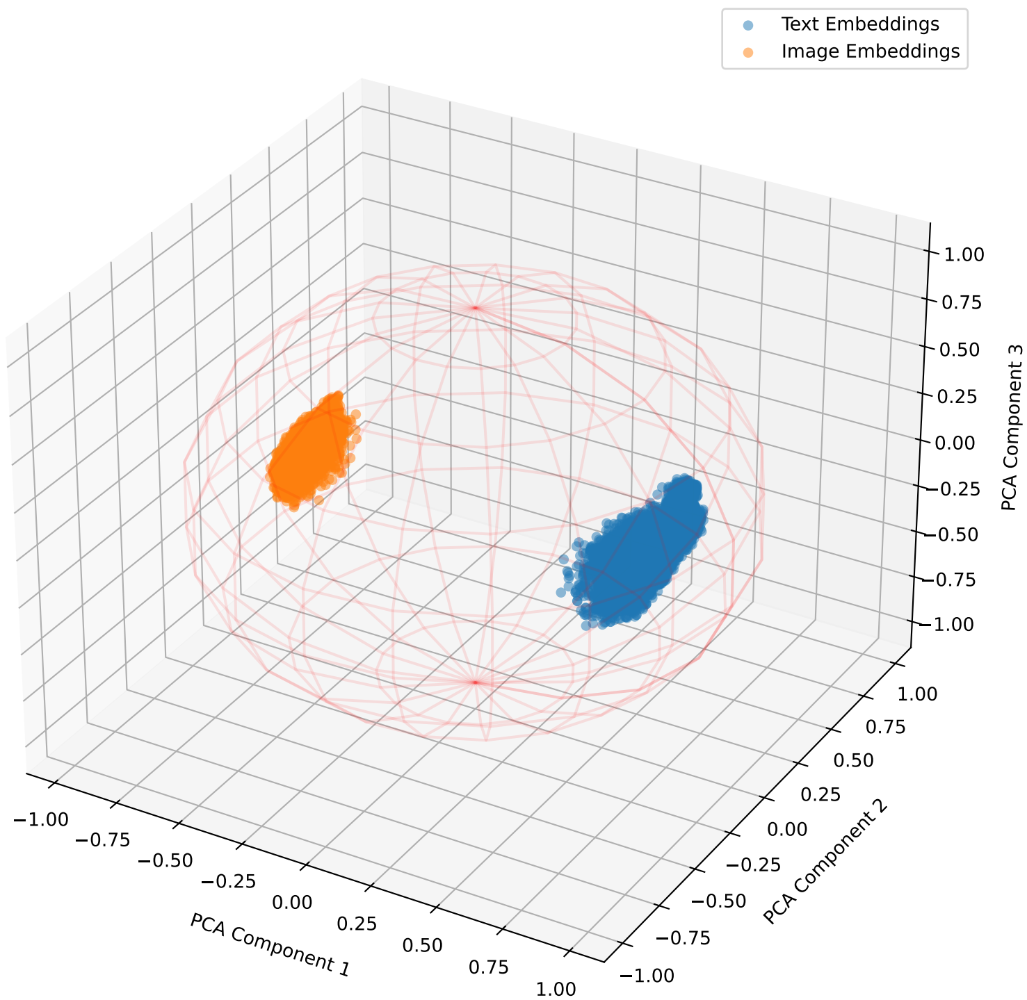
Embeddings with Lambda Shift -0.7 for Recipes5k in 3D
