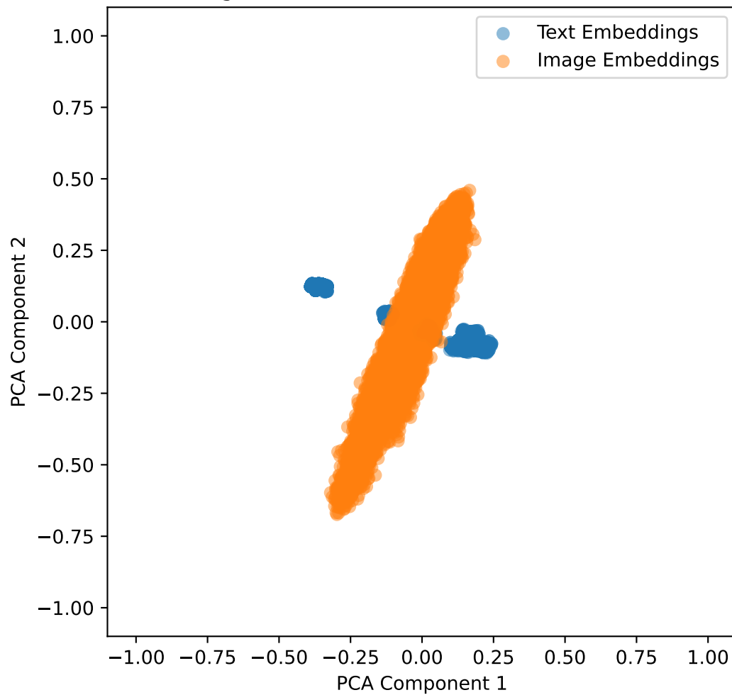
Embeddings with Lambda Shift 0.9 for ham10000 in 2D
