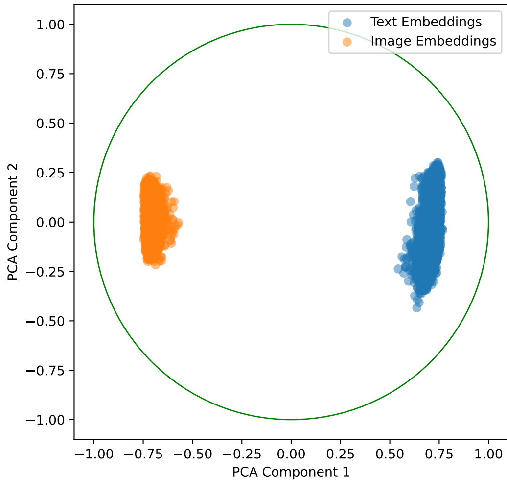
Embeddings with Lambda Shift -0.9 for Recipes5k in 2D
