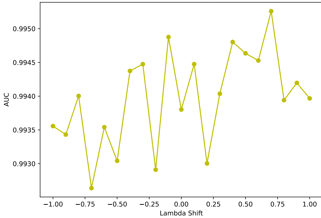
Late Fusion AUC - Recipes5k
