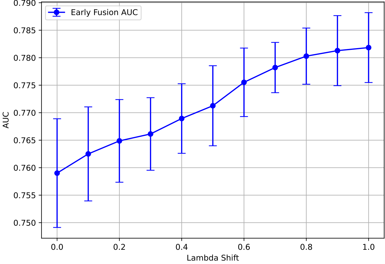
Early Fusion AUC - ham10000
