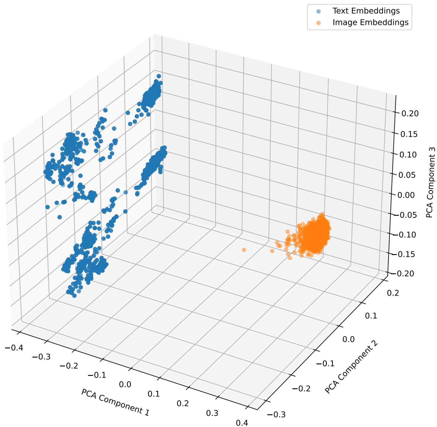
Embeddings with Lambda Shift 0.6 for mbrset in 3D
