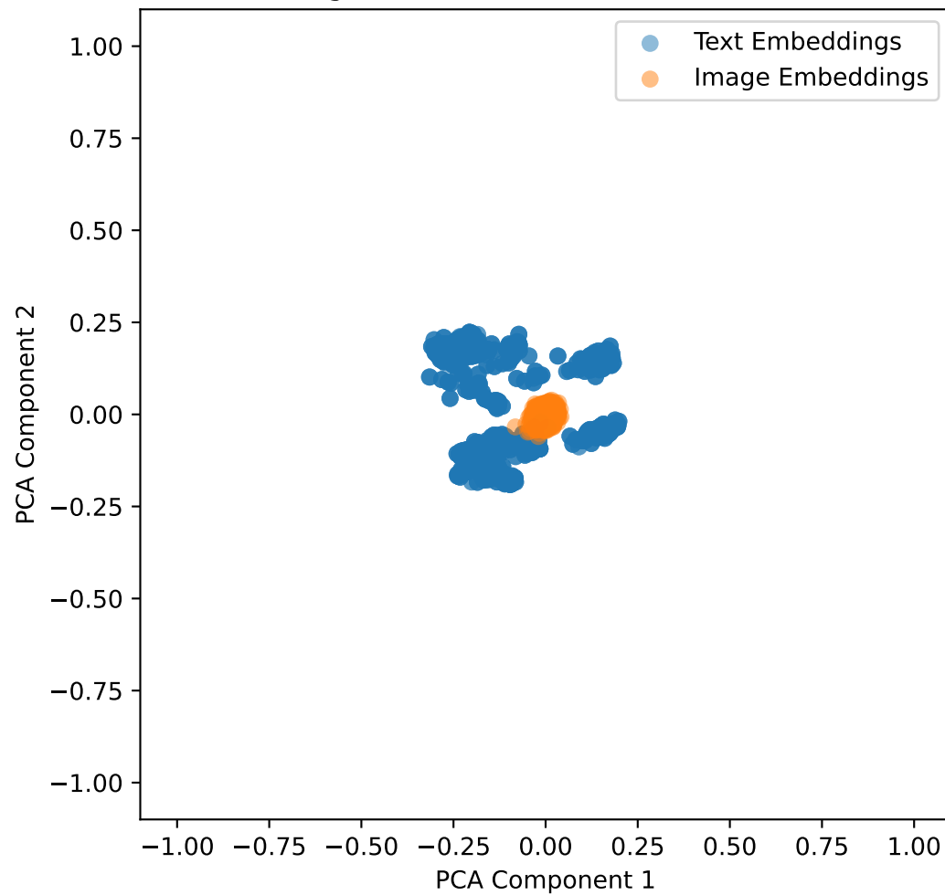
Embeddings with Lambda Shift 1 for mbrset in 2D
