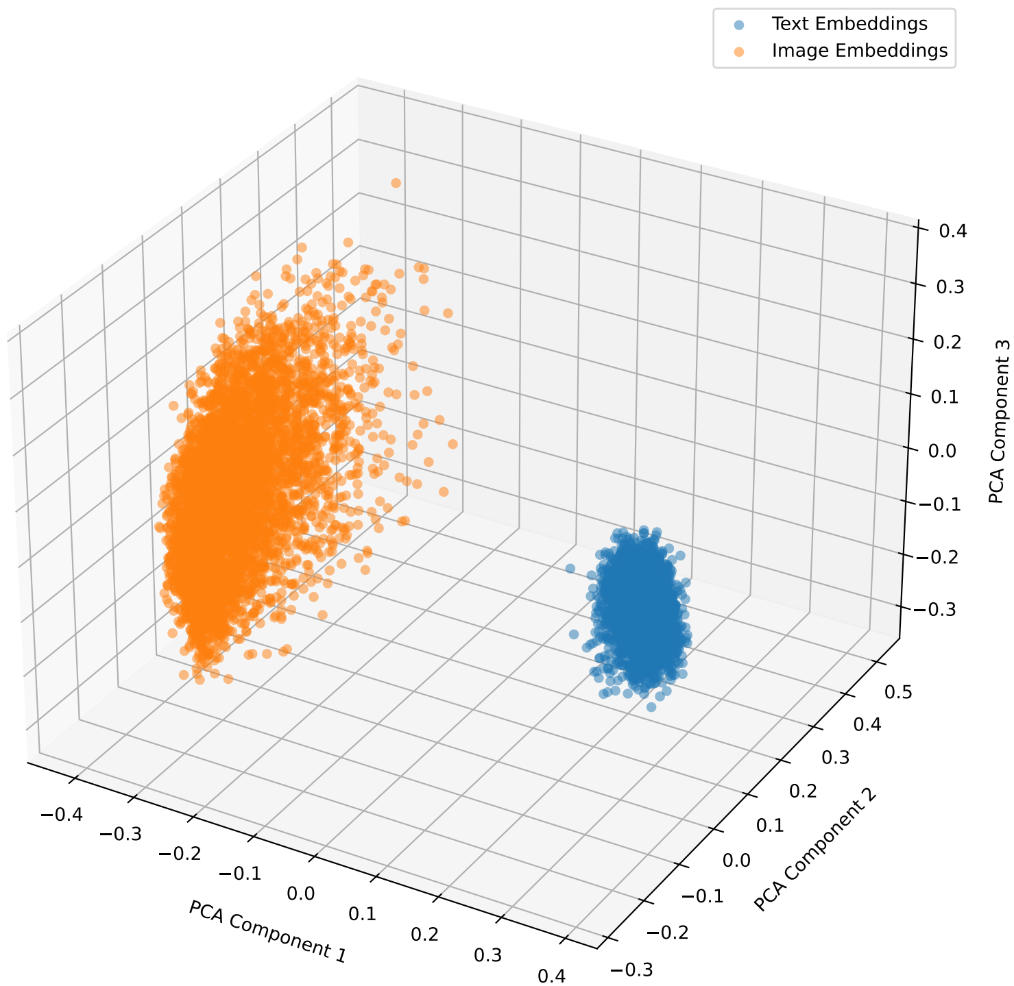
Embeddings with Lambda Shift 0.5 for mbrset in 3D
