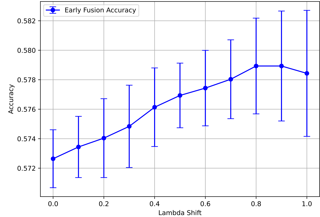
Early Fusion Accuracy - ham10000
