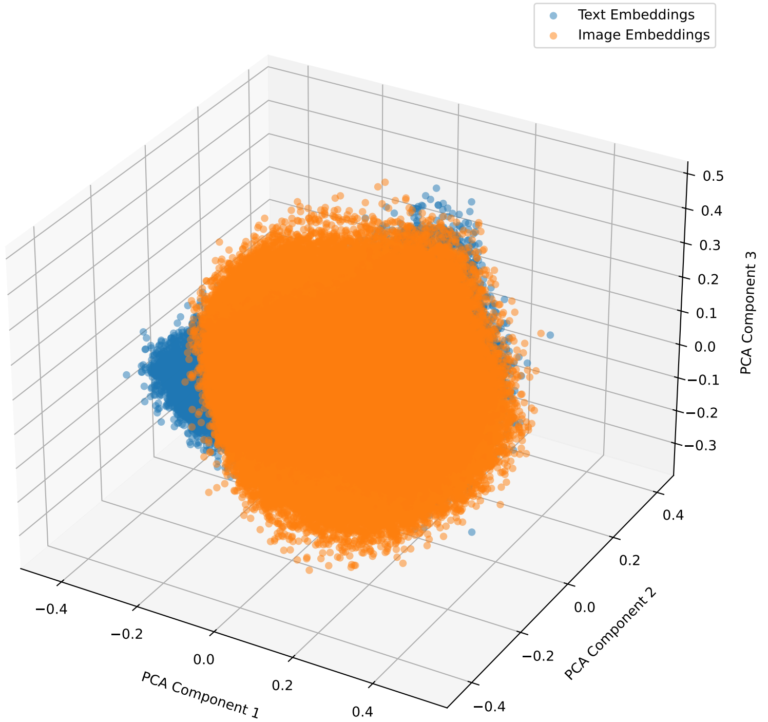
Embeddings with Lambda Shift 1 for mimic in 3D
