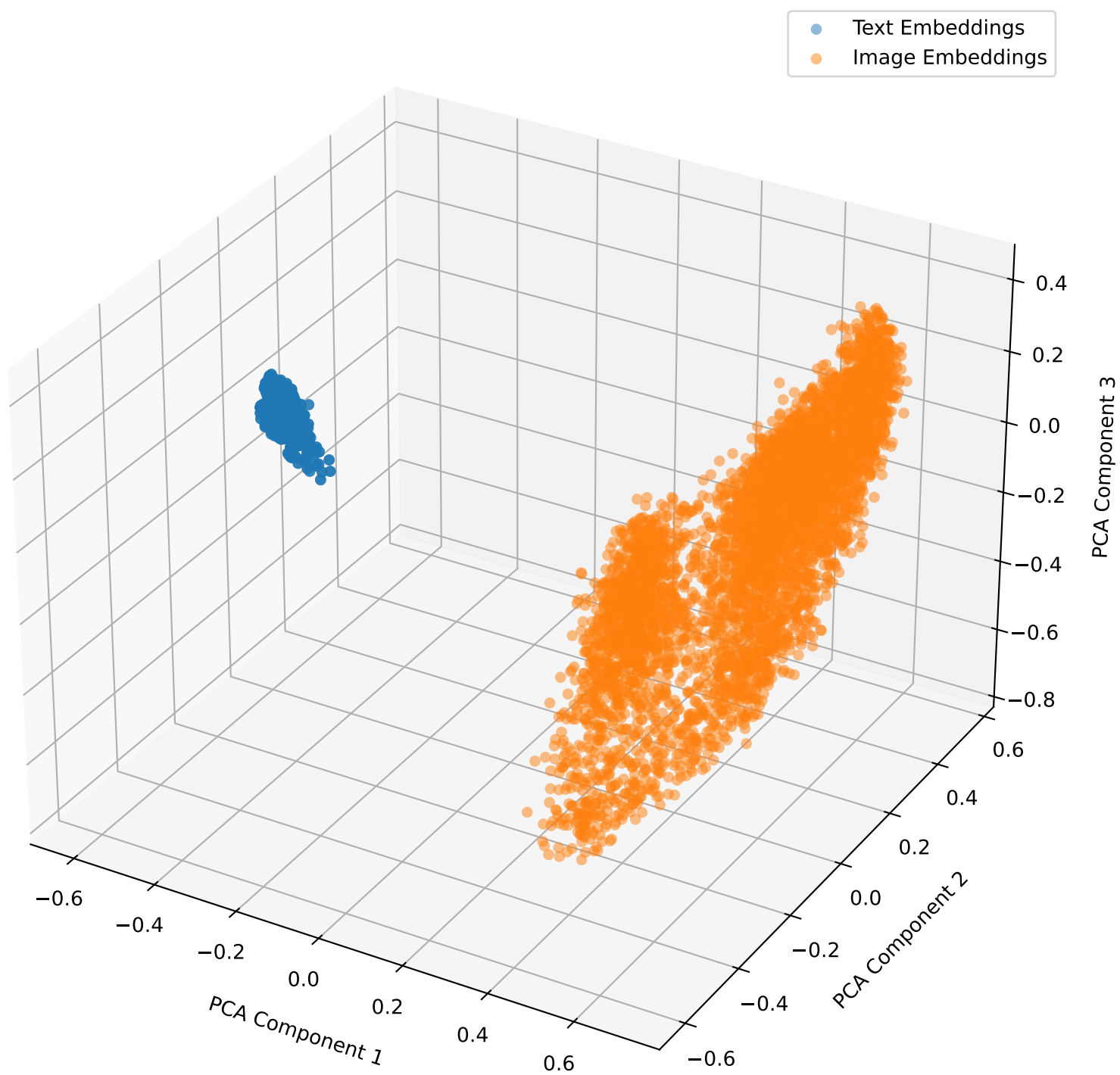
Embeddings with Lambda Shift 0.3 for mbrset in 3D
