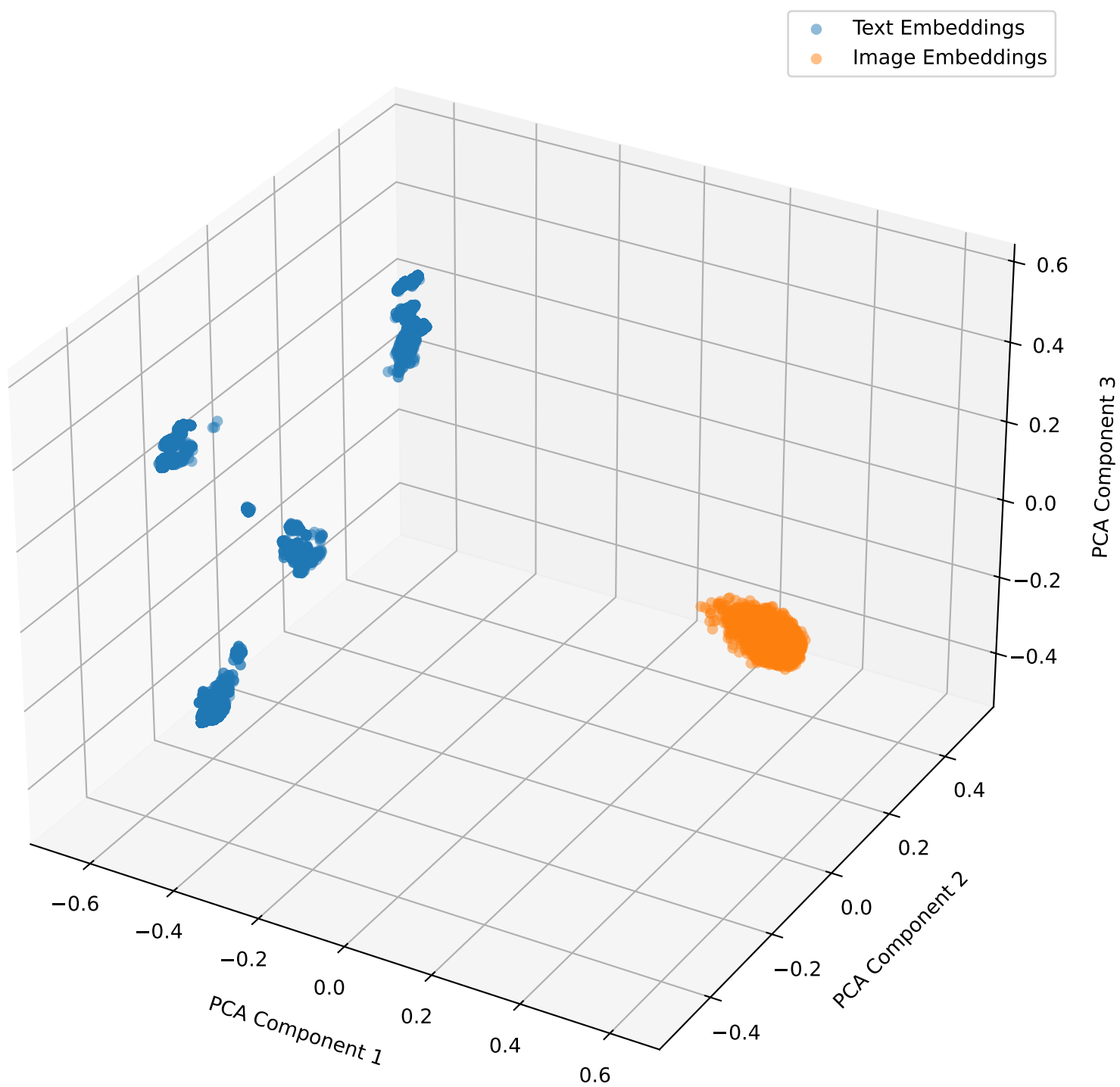
Embeddings with Lambda Shift 0.2 for ham10000 in 3D
