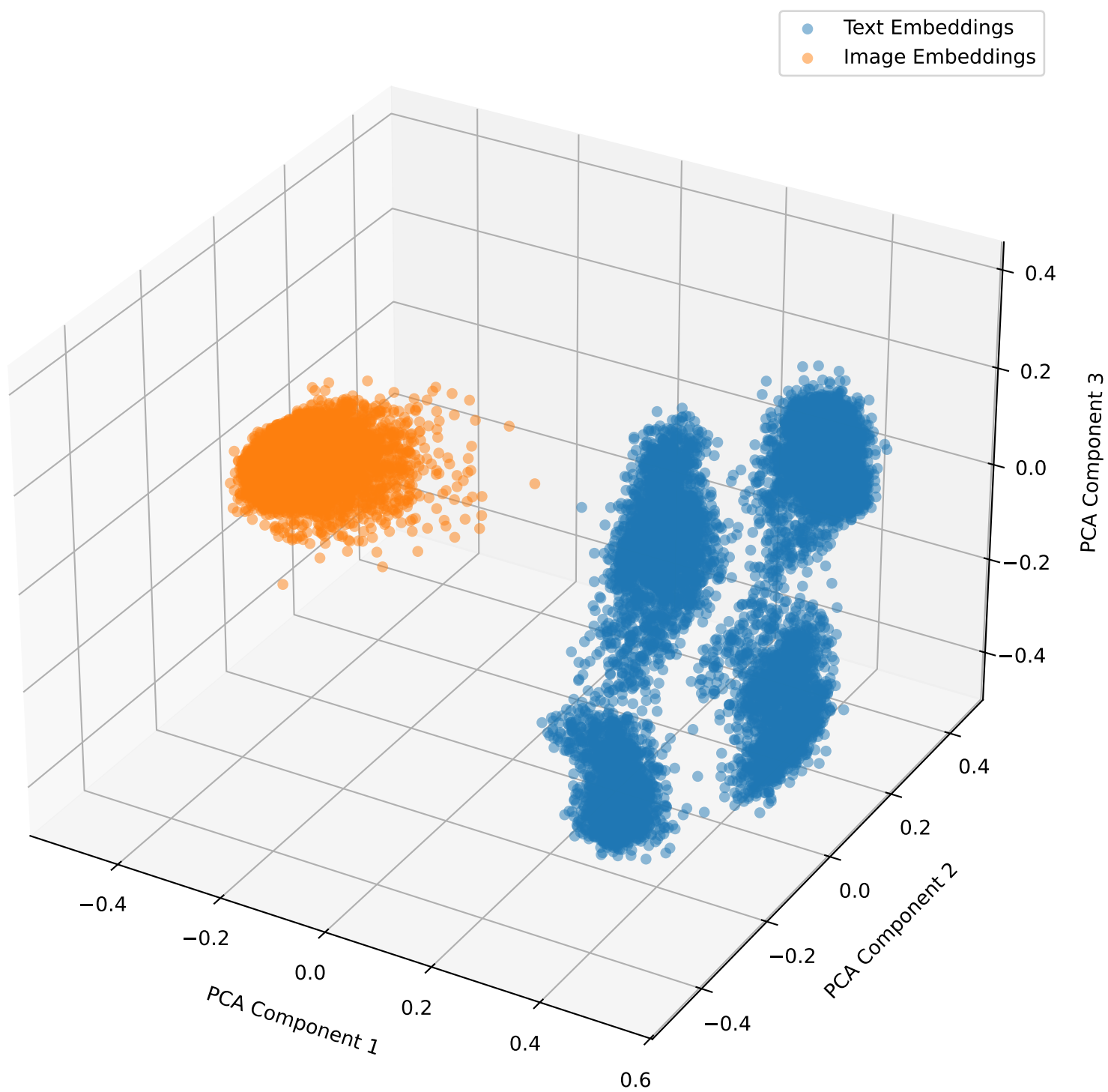
Embeddings with Lambda Shift 0.3 for ham10000 in 3D
