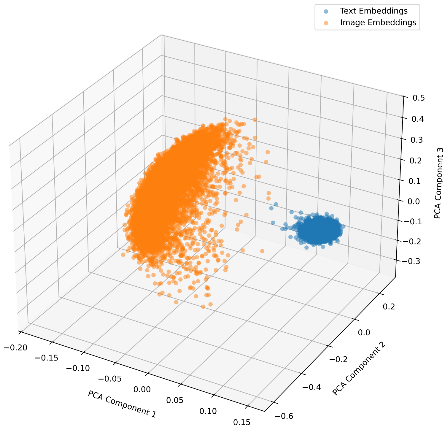
Embeddings with Lambda Shift 0.8 for brset in 3D
