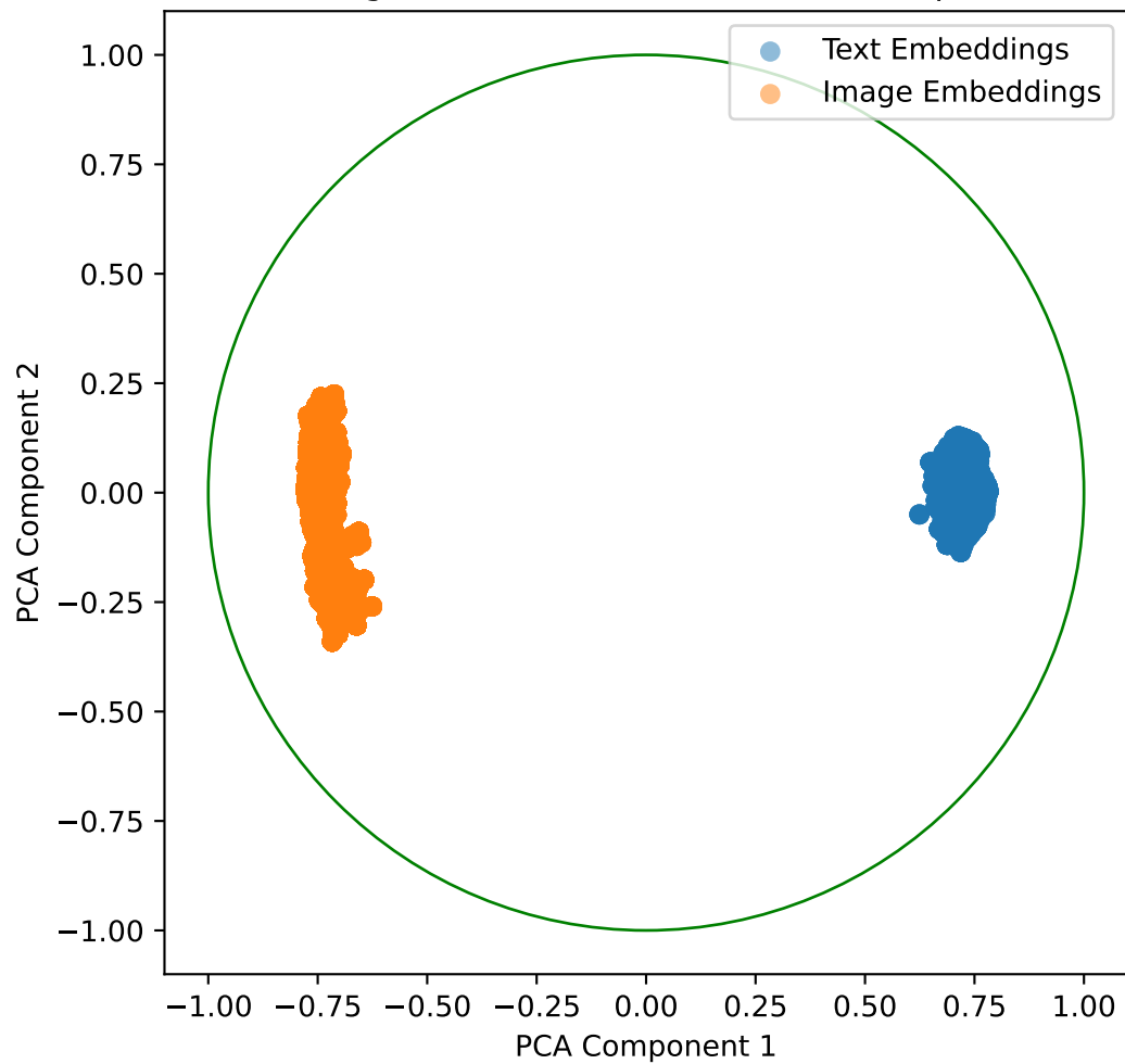
Embeddings with Lambda Shift -0.8 for daquar in 2D
