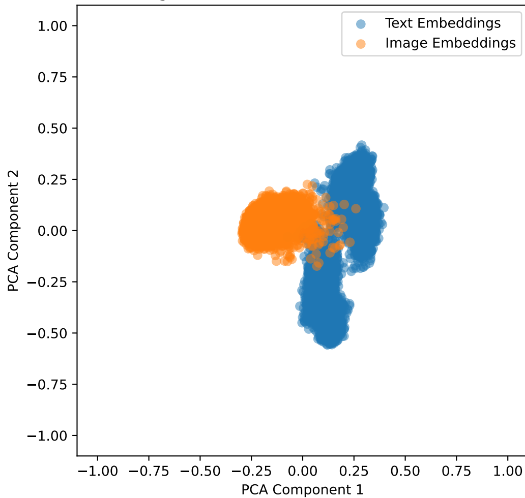
Embeddings with Lambda Shift 0.7 for ham10000 in 2D
