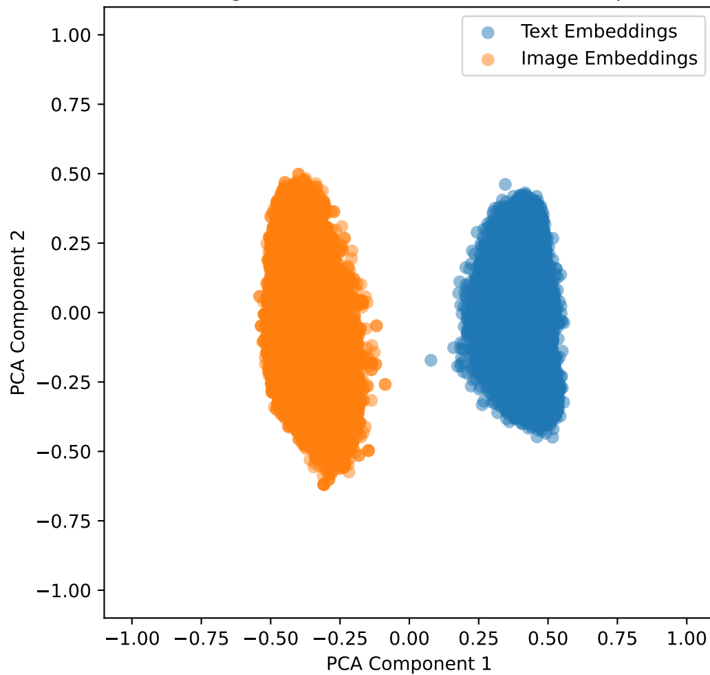
Embeddings with Lambda Shift 0.0 for coco-qa in 2D
