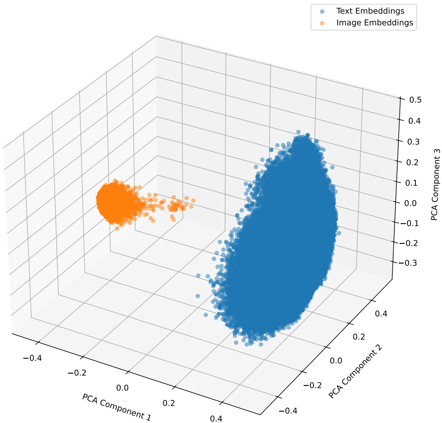
Embeddings with Lambda Shift 0.3 for mimic in 3D
