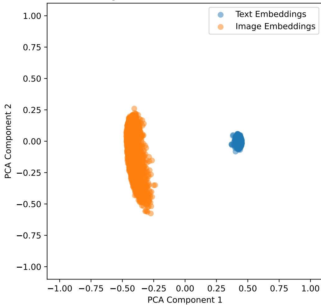
Embeddings with Lambda Shift 0.2 for brset in 2D
