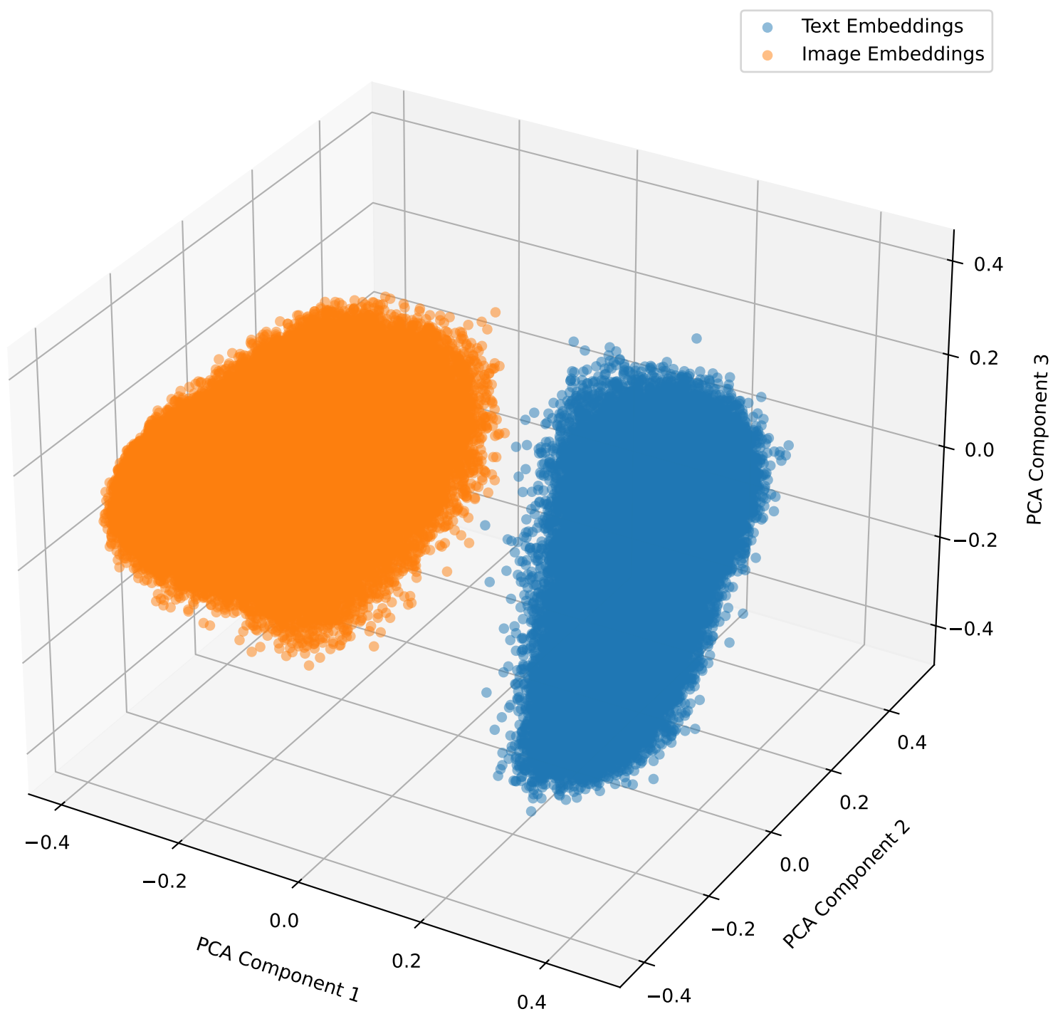
Embeddings with Lambda Shift 0.4 for mimic in 3D
