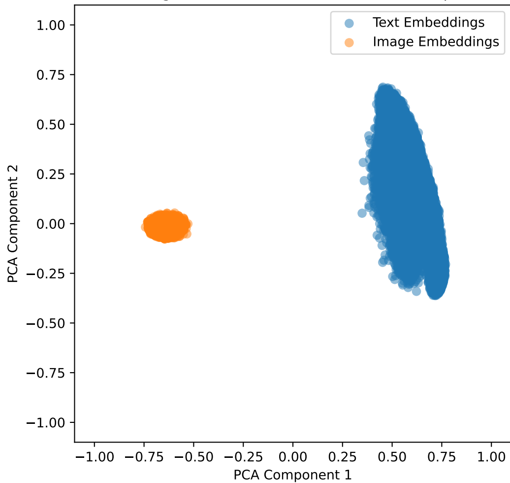
Embeddings with Lambda Shift -0.5 for coco-qa in 2D
