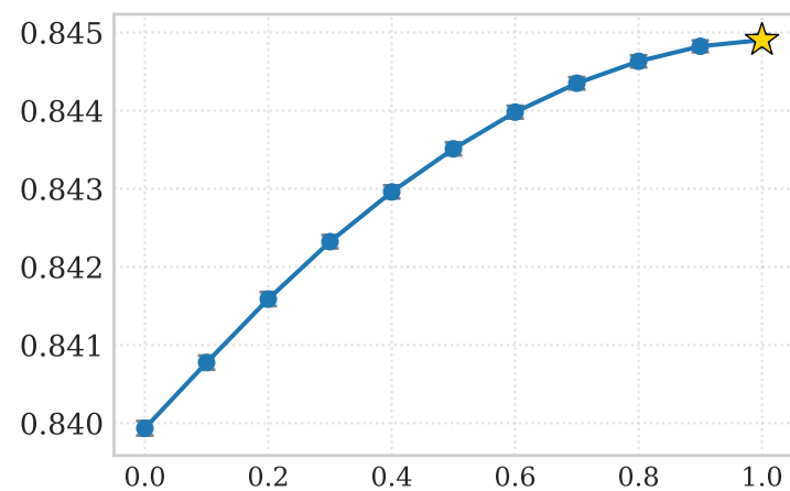
CLIP (General)
