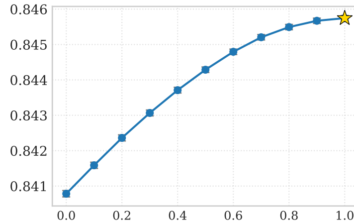
SigLIP (General)
