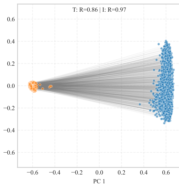
SigLIP (General)
