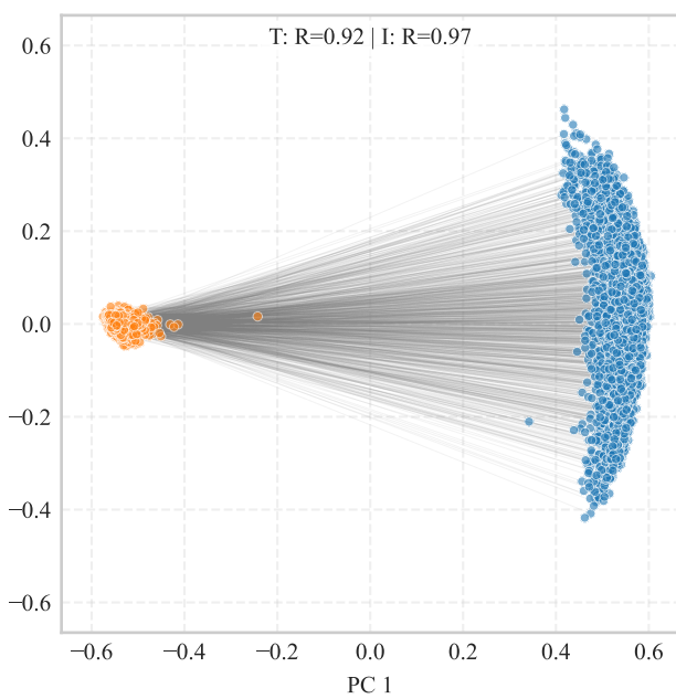
CLIP (General)
