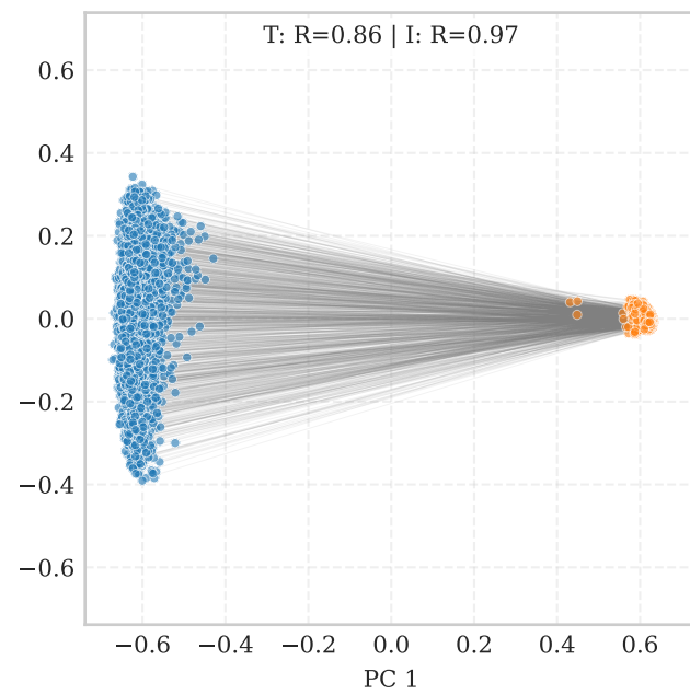
SigLIP (General)
