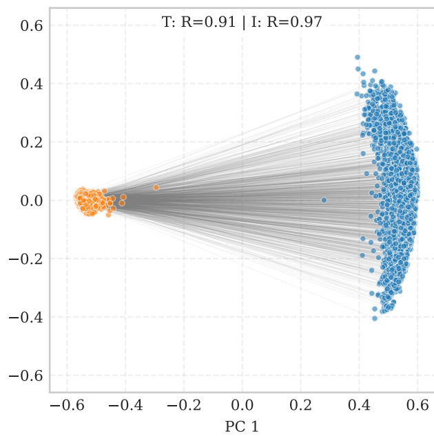
CLIP (General)
