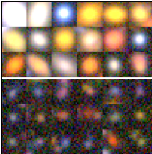
SED (union) detections
