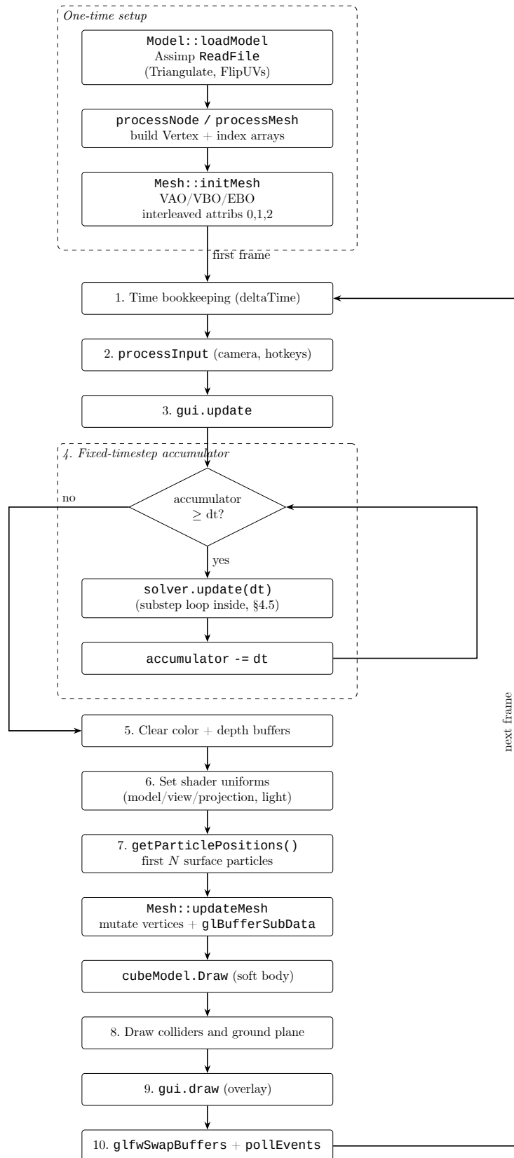
Слика 7.1: The rendering pipeline. One-time asset setup (top) feeds the GPU buffers once. The per-frame loop handles input, then advances physics via a fixed-timestep accumulator, and only afterwards clears the buffers and re-uploads the surface particles for drawing. Step numbers correspond to the annotated frame loop in main.cpp .
