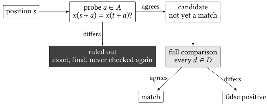
Figure 1. The filter as bench/driver/bench_ancorae_lattice.c:193-239 implements it. A probe settles only one outcome for certain, ruling the position out. The other two need the full comparison, and everything below the candidate box costs time.
