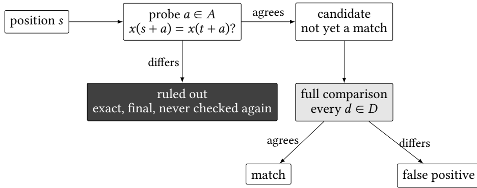
Figure 1. The filter as the benches implement it. A probe settles only one outcome for certain, ruling the position out. The other two need the full comparison, and everything below the candidate box costs time.
