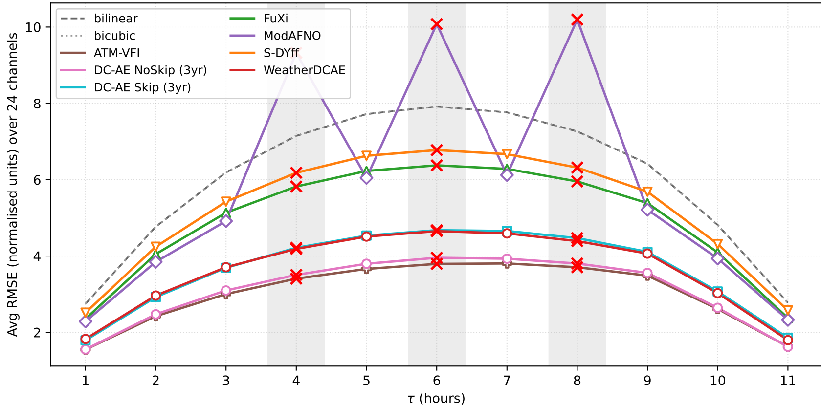
RMSE vs interpolation step \tau for the 12 h window Held-out \tau \in \{4, 6, 8\} — measures continuous-time generalization
