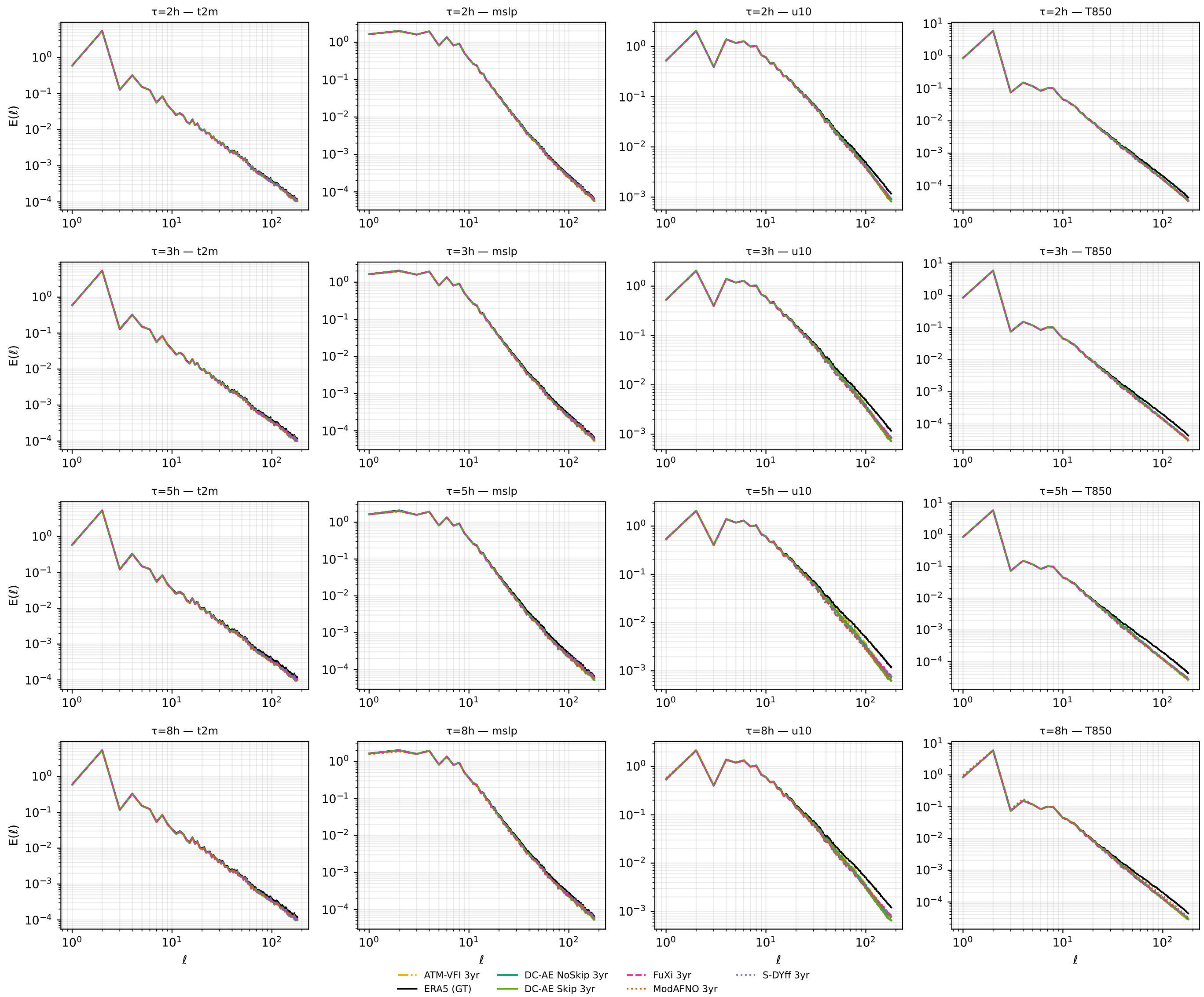
Angular SH power spectra E(\ell) — 12h interpolation, ep10 ckpts
