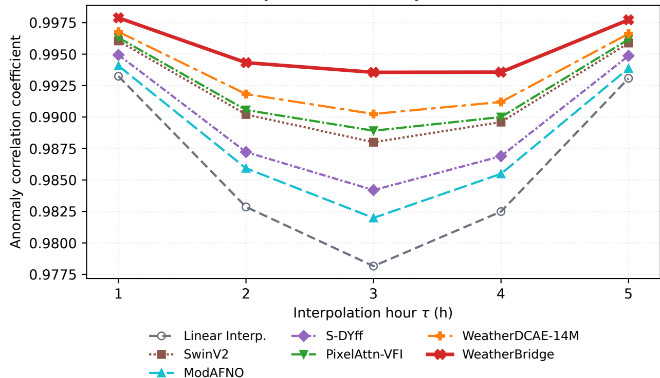
Full-year 2020 anomaly correlation
