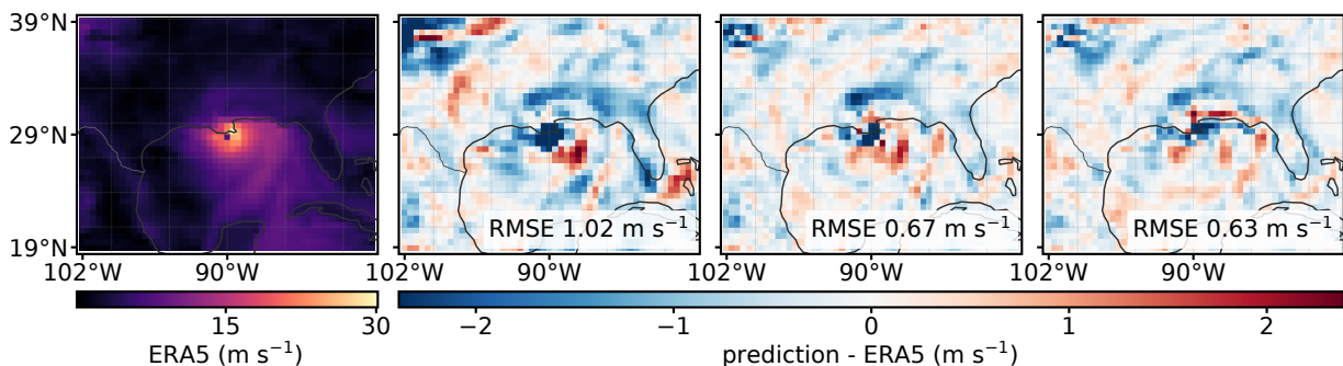
c) Ida | 10-m wind | 29 Aug 2021, 15 UTC
