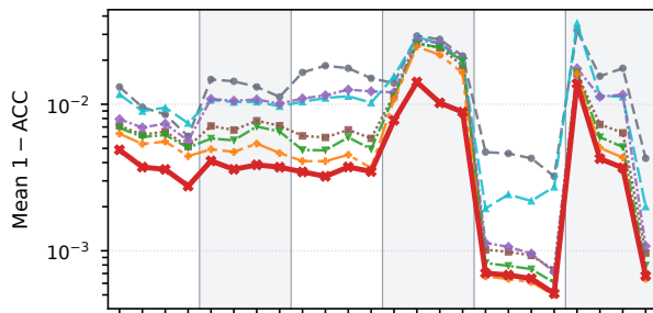
b) 6 h: WeatherBridge best on 19/24 fields
