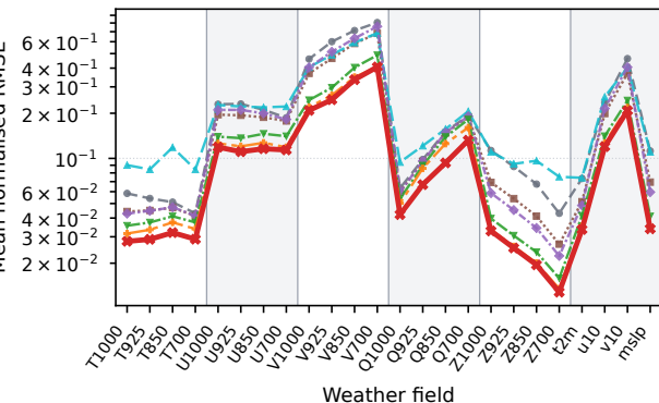
c) 12 h: WeatherBridge best on 23/24 fields
