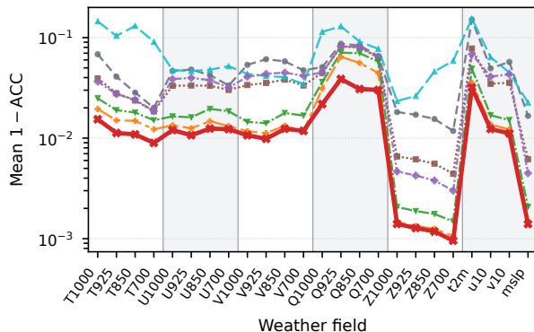
d) 12 h: WeatherBridge best on 23/24 fields
