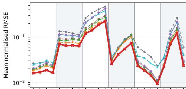
a) 6 h: WeatherBridge best on 19/24 fields
