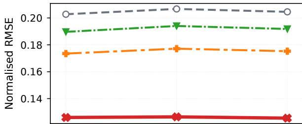
a) Specific humidity, 850 hPa
