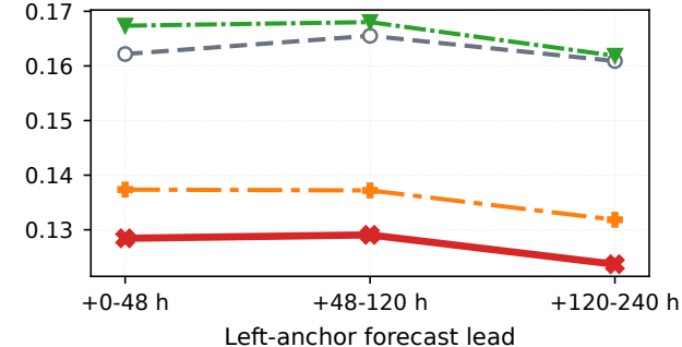
d) Mean sea-level pressure
