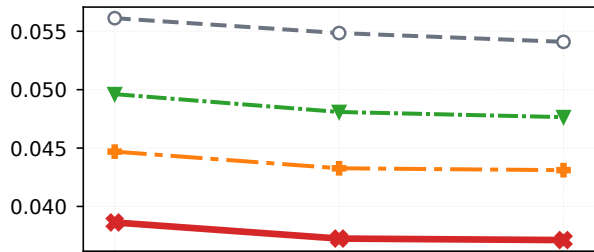
b) Temperature, 700 hPa
