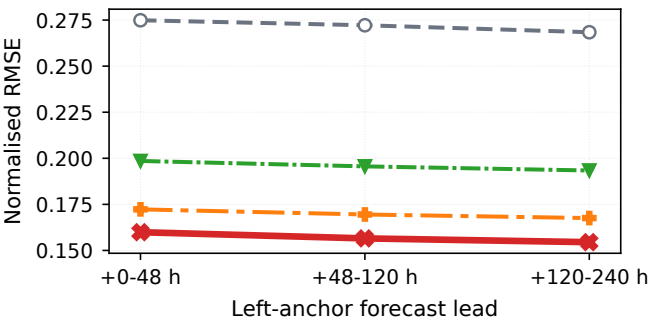
c) Zonal wind, 850 hPa
