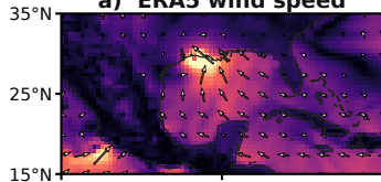
a) ERA5 wind speed
