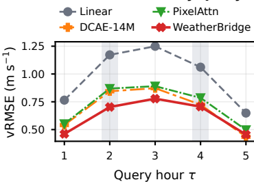
f) Vector RMSE by query hour
