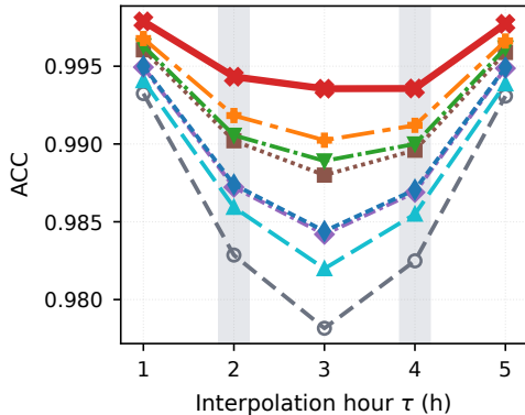
b) Anomaly correlation
