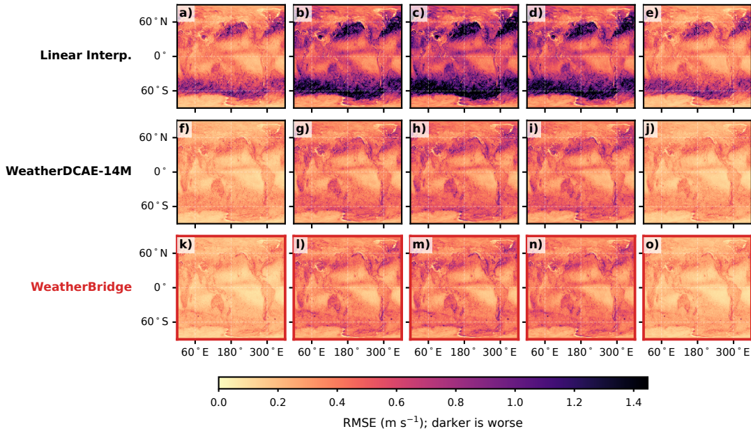
10 m zonal wind: per-grid-cell RMSE over 96 uniformly sampled 2020 windows \tau = 1 h \tau = 2 h \tau = 3 h \tau = 4 h \tau = 5 h
