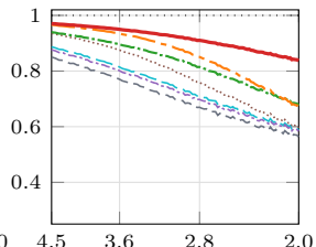
h) U850, \tau = 3
