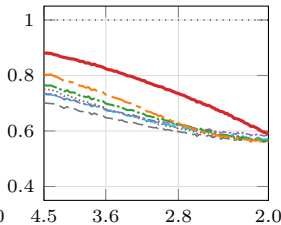
f) Q850, \tau = 3
