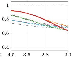
g) U850, \tau = 2
