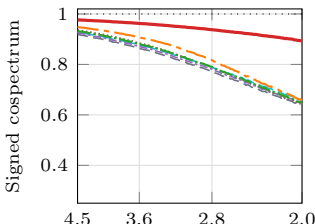
e) Q850, \tau = 2
