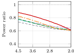
e) Q850, \tau = 2
