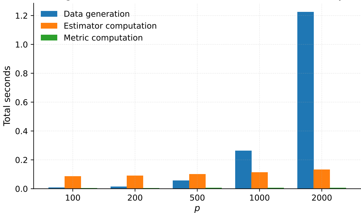
Single simulation runtime breakdown (Student-t) - Cholesky
