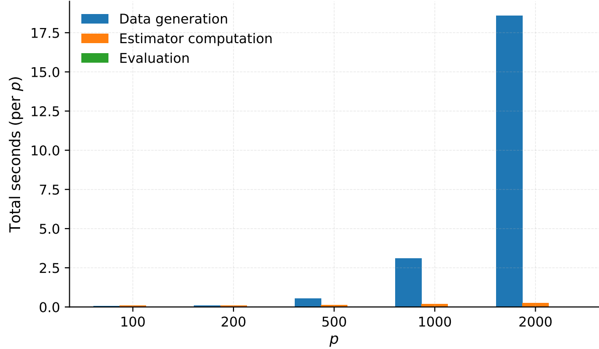
Convergence simulation runtime breakdown (all SNRs) - Cholesky + Parallelization
