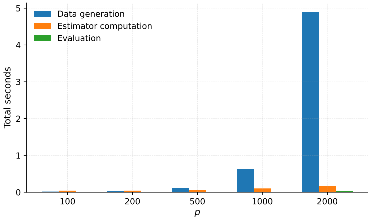
Multi simulation runtime breakdown (Normal) - Cholesky + Parallelization
