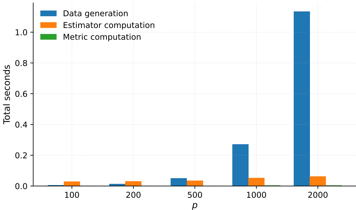
Multi simulation runtime breakdown (Normal) - Cholesky
