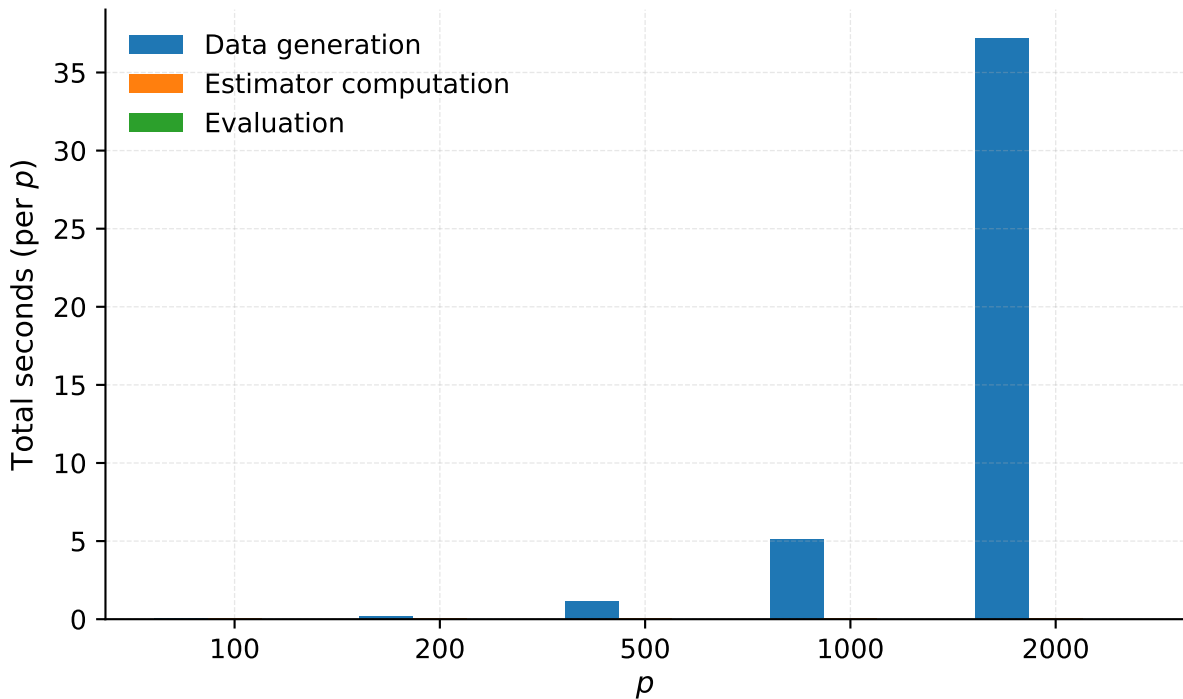
Multi simulation runtime breakdown (Normal) - Baseline
