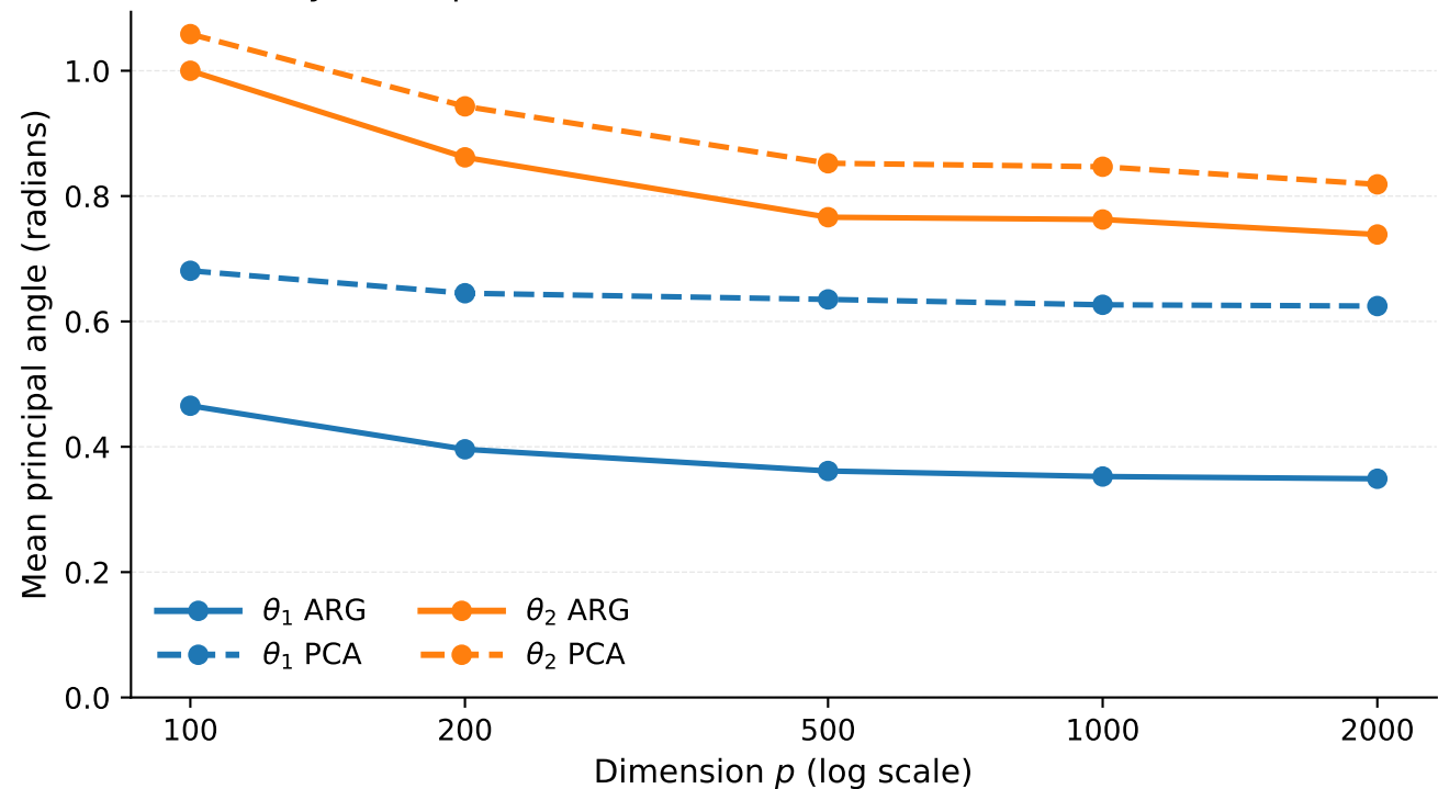
[cholesky] Two-spike, two-reference (normal) — \theta_1 / \theta_2 across methods
