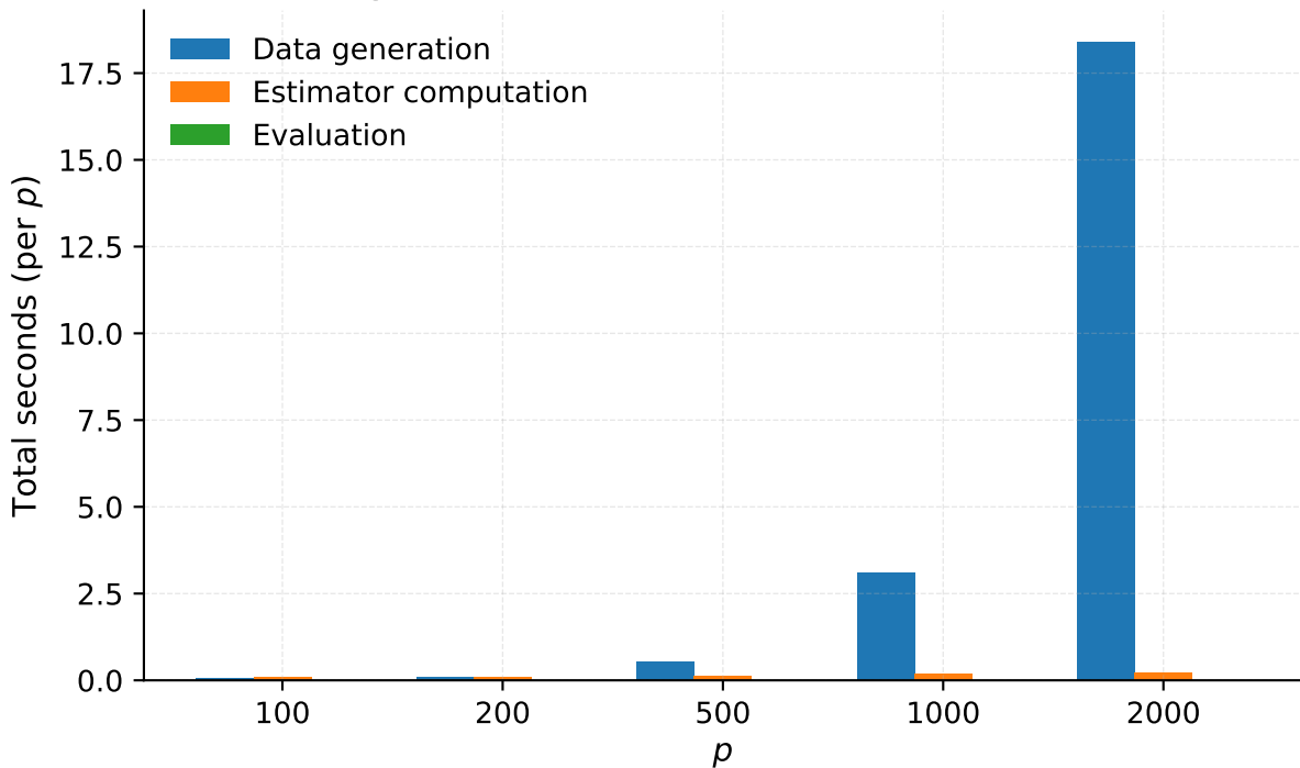
Convergence simulation runtime breakdown (all SNRs)
