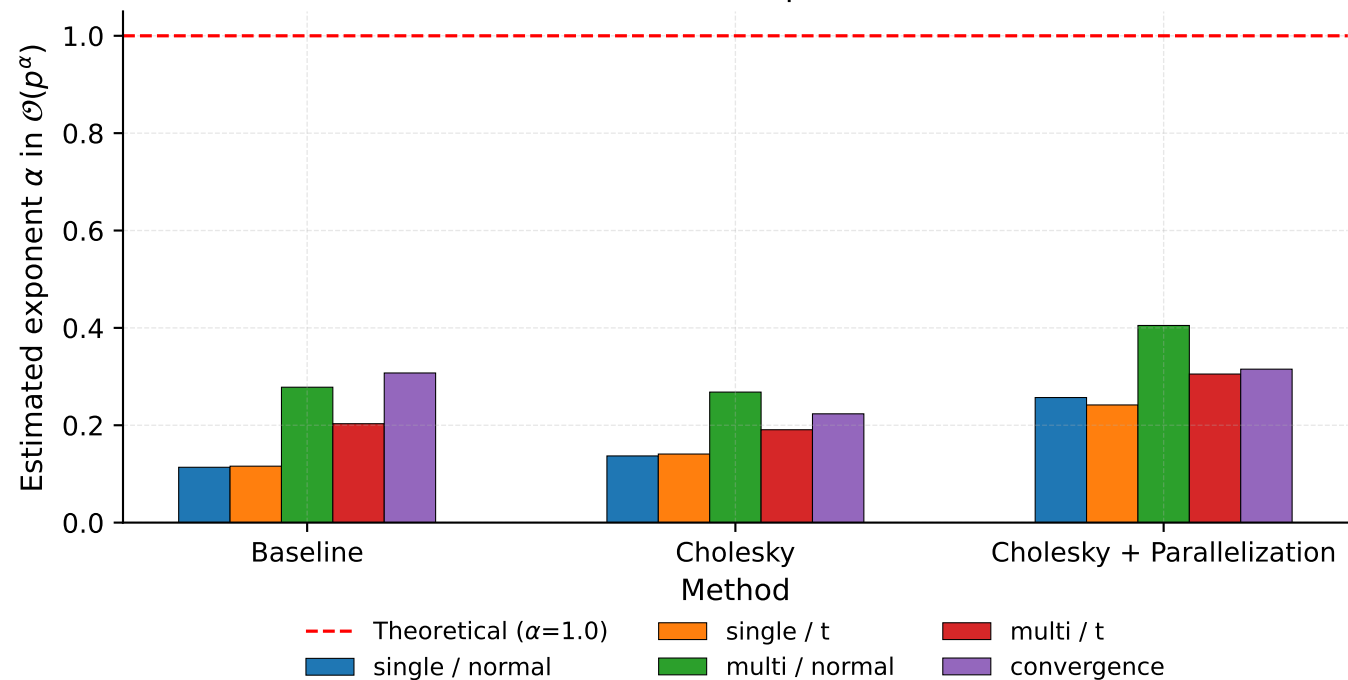
Complexity exponents by method and experiment (Estimator computation)
