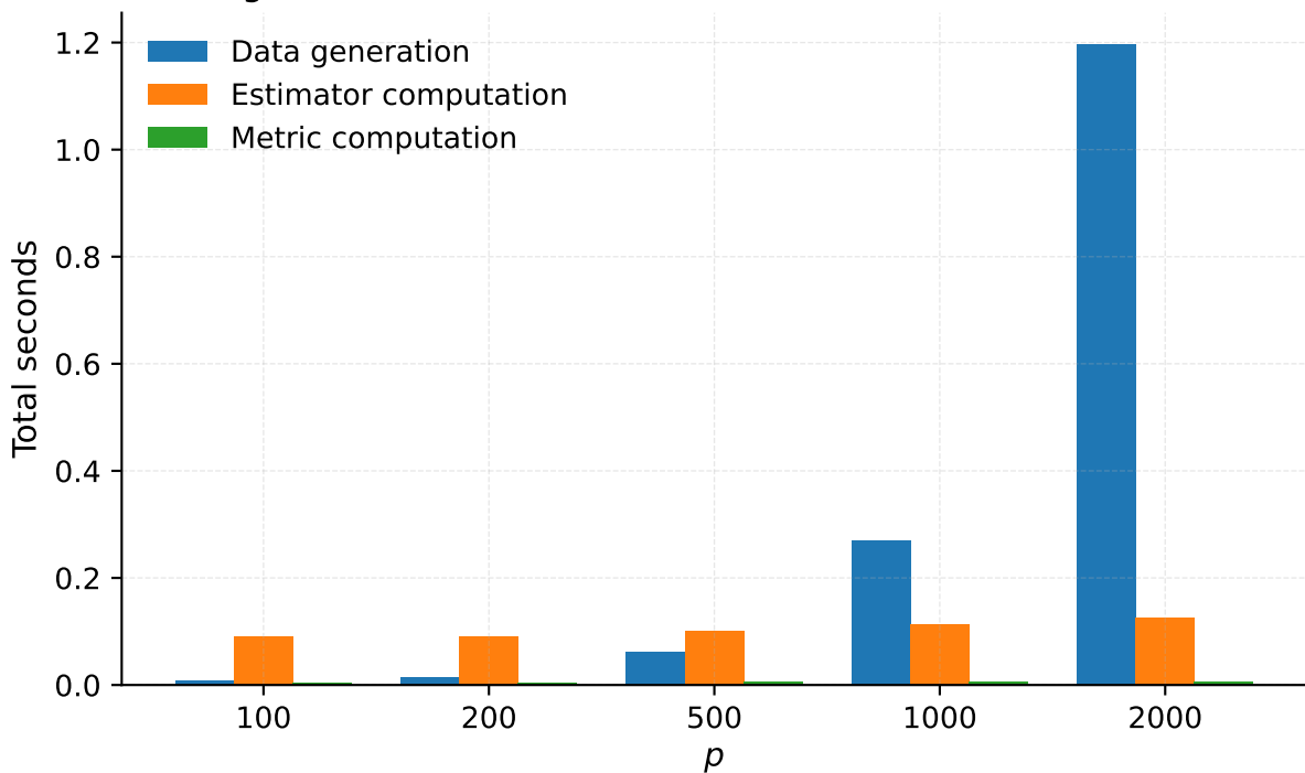
Single simulation runtime breakdown (Student-t) - Baseline
