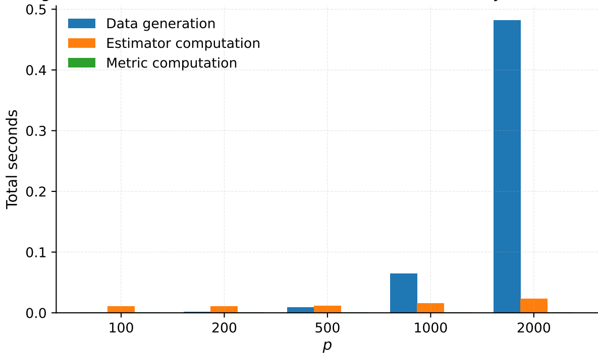
Single simulation runtime breakdown (Student-t) - Cholesky + Parallelization
