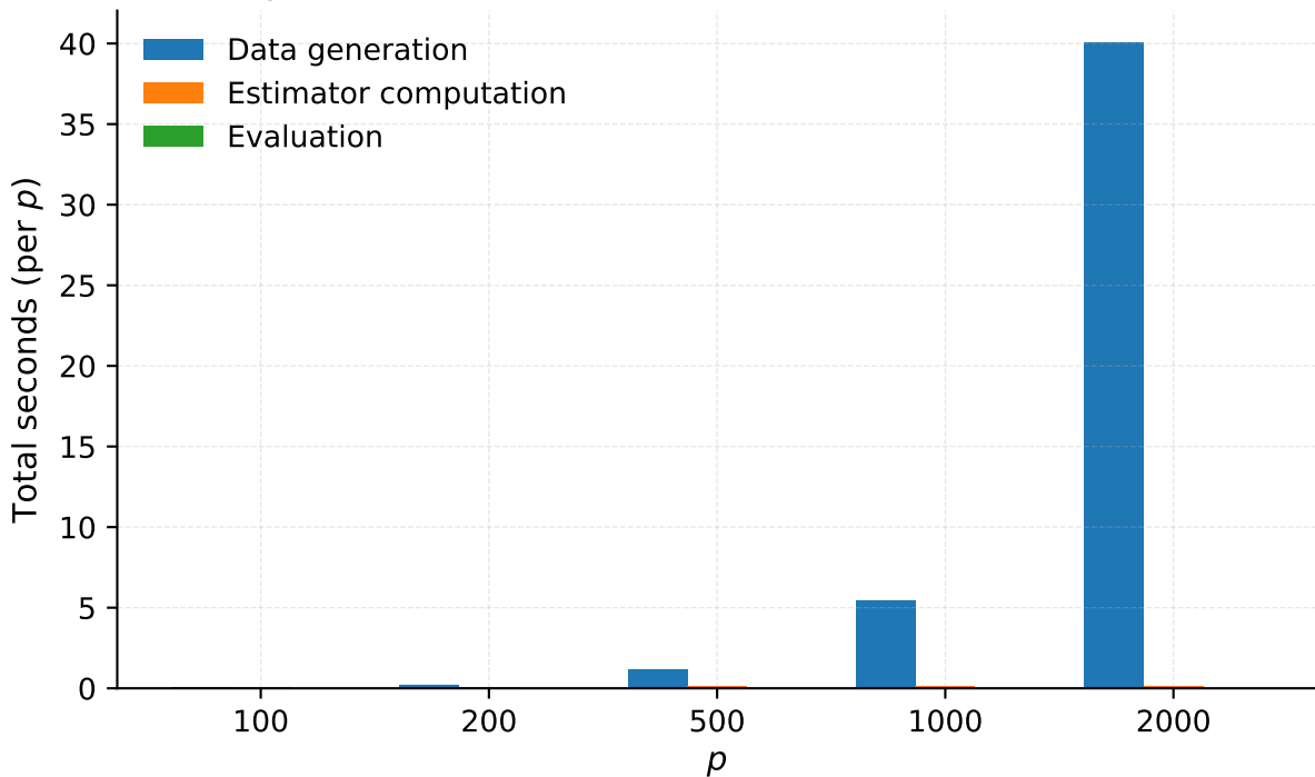
Single simulation runtime breakdown (Normal) - Baseline
