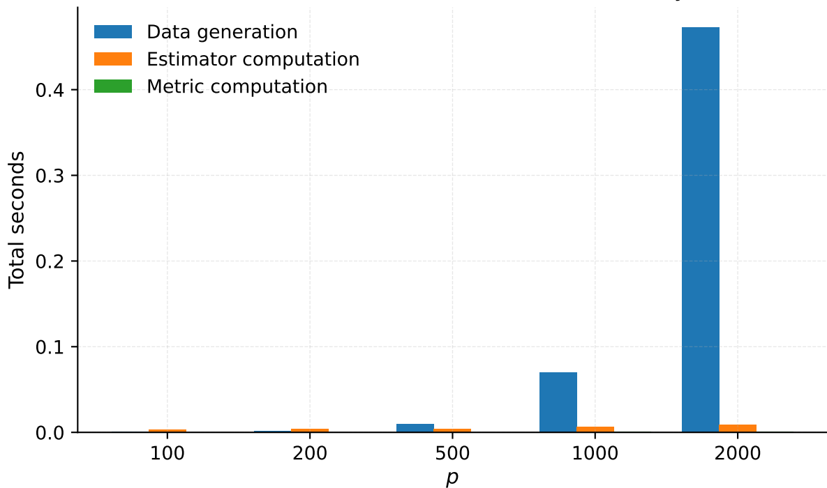
Multi simulation runtime breakdown (Student-t) - Cholesky + Parallelization
