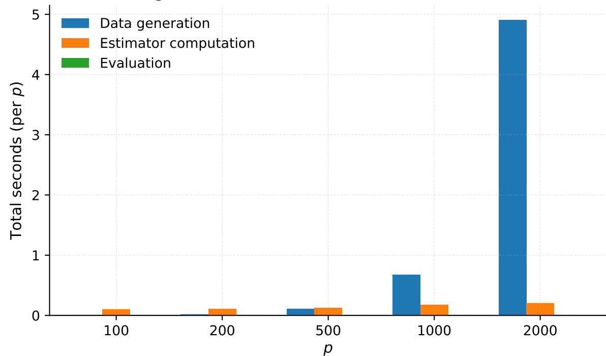
Single simulation runtime breakdown (Student-t)
