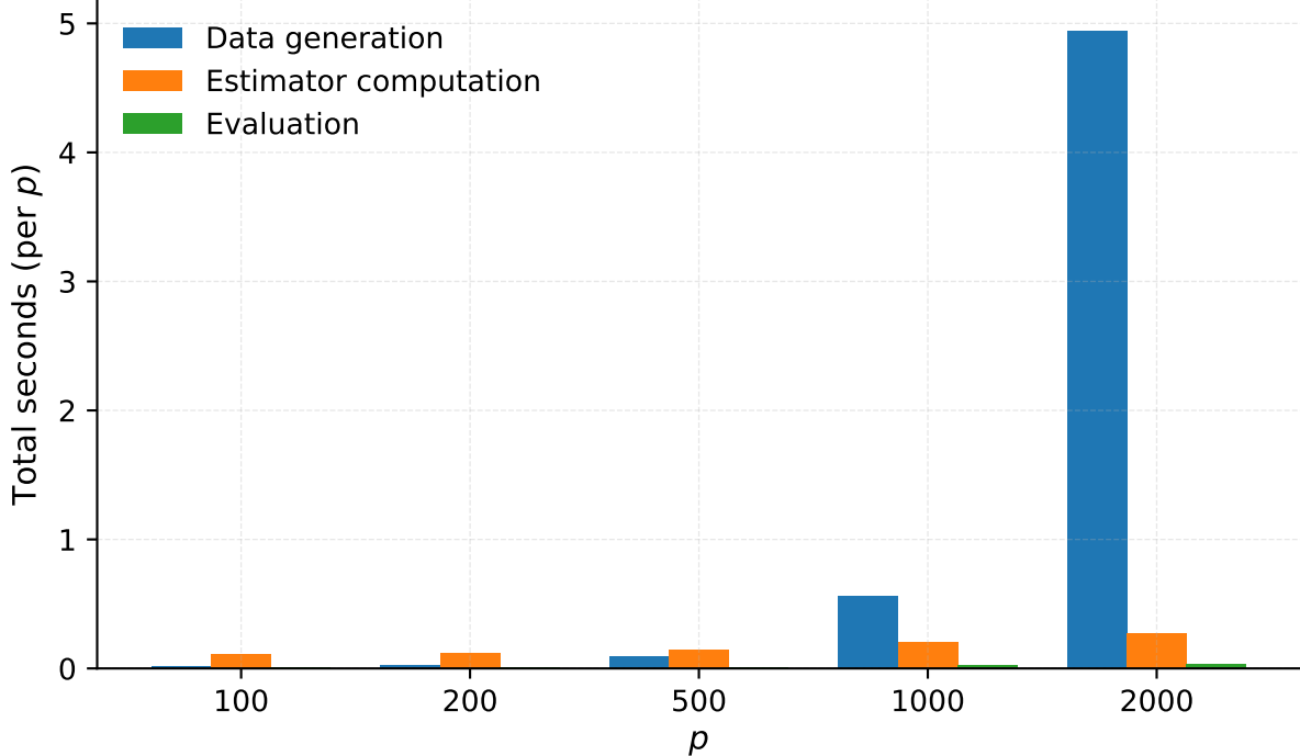
Single simulation runtime breakdown (Normal) - Cholesky + Parallelization
