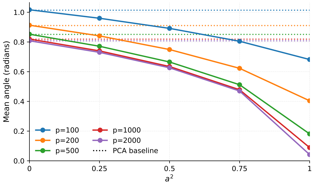
[cholesky+parallelization] Single-spike, single-reference (normal) — trend over a^2
