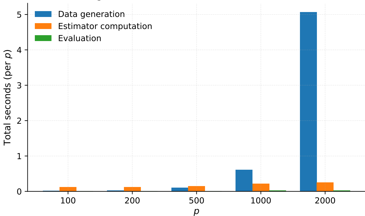
Single simulation runtime breakdown (Normal)
