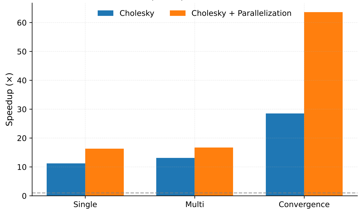
Overall speedup relative to Baseline
