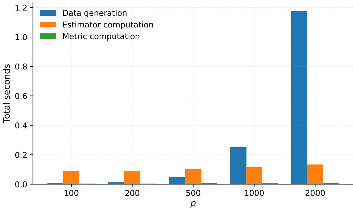
Single simulation runtime breakdown (Normal) - Cholesky
