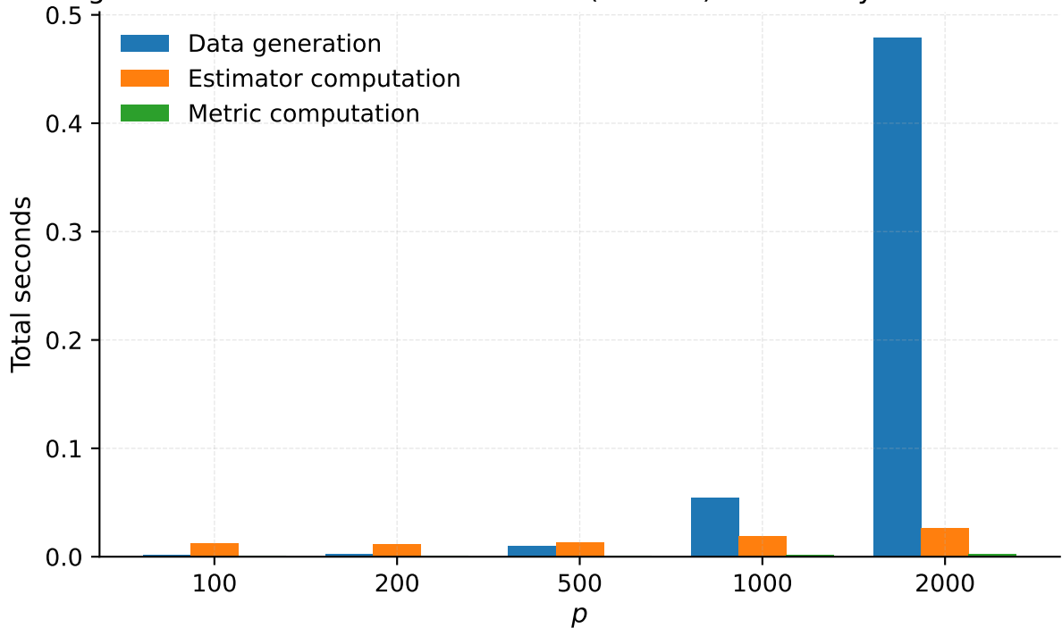
Single simulation runtime breakdown (Normal) - Cholesky + Parallelization
