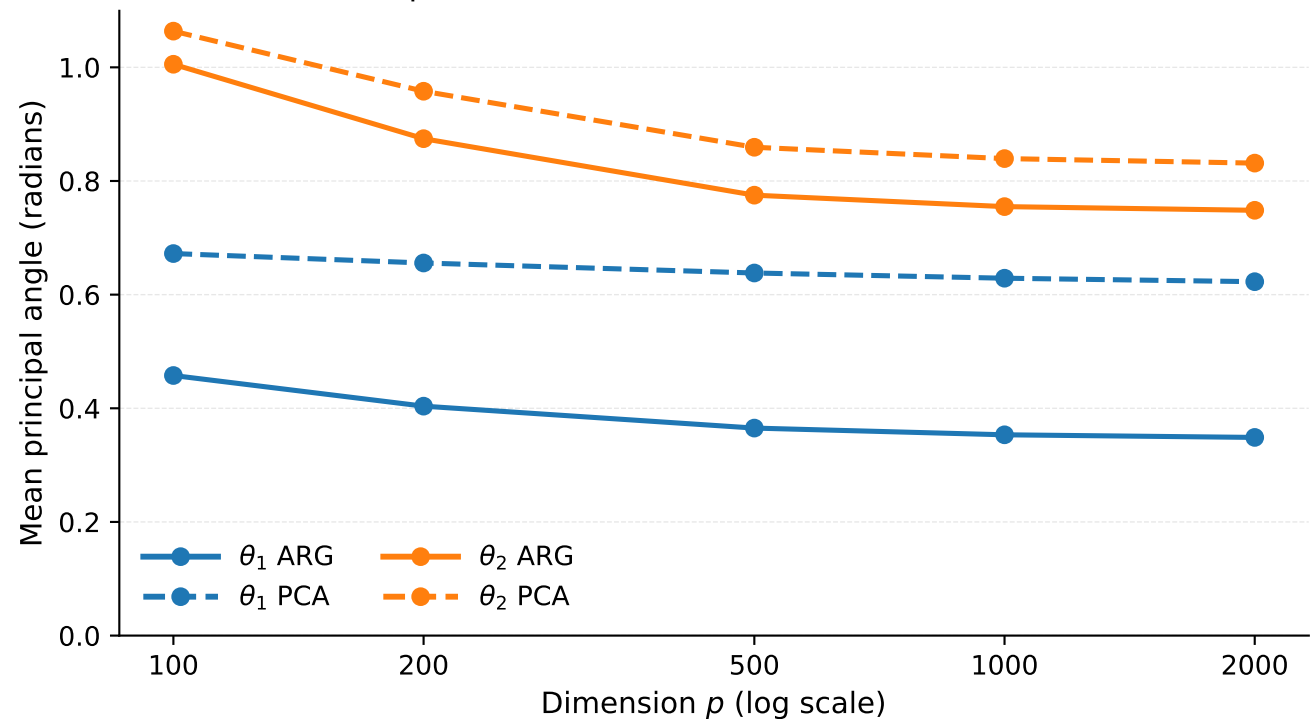
[baseline] Two-spike, two-reference (normal) — \theta_1 / \theta_2 across methods
