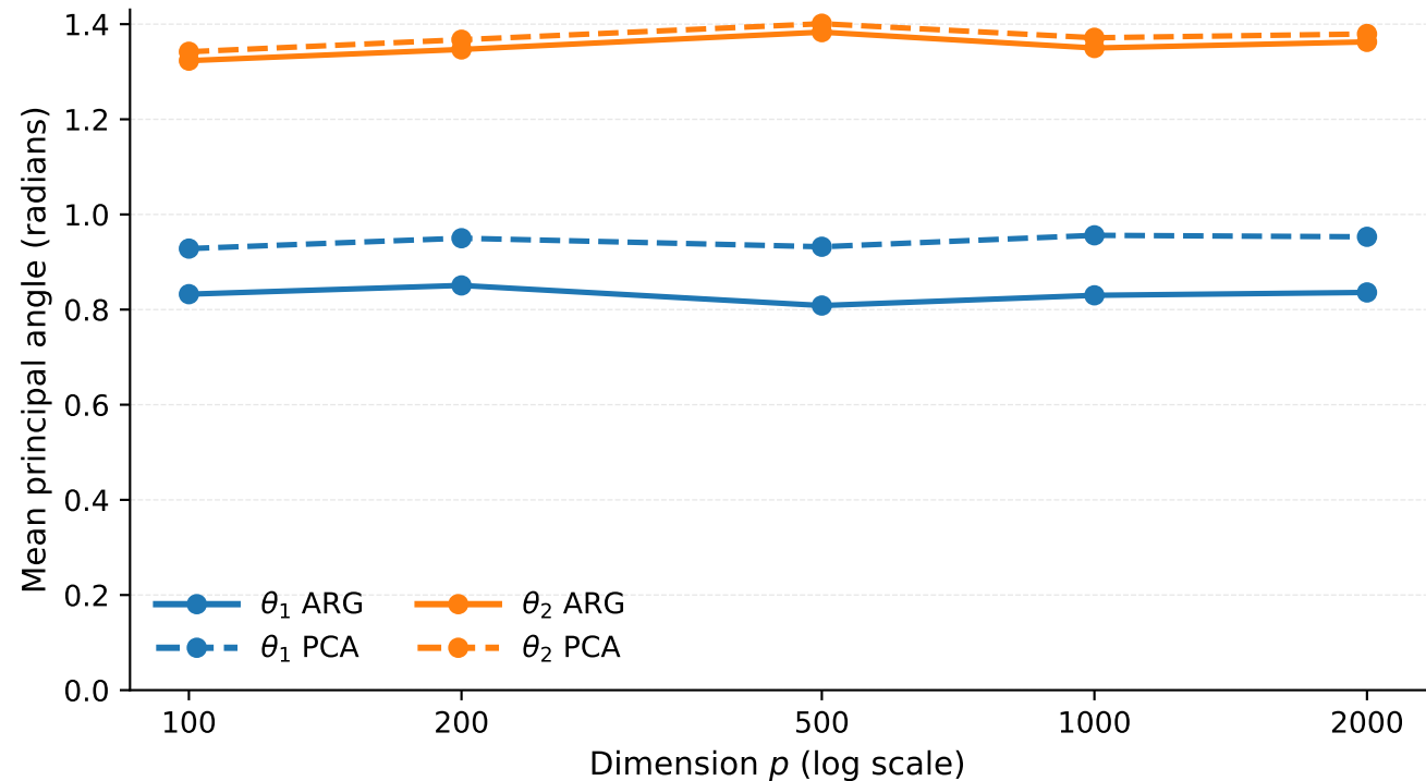
[cholesky+parallelization] Two-spike, two-reference (t) — \theta_1 / \theta_2 across methods
