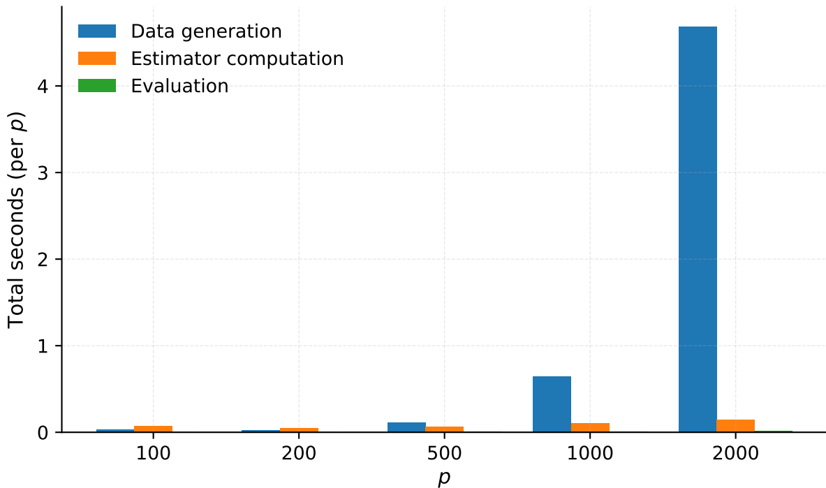
Multi simulation runtime breakdown (Normal)
