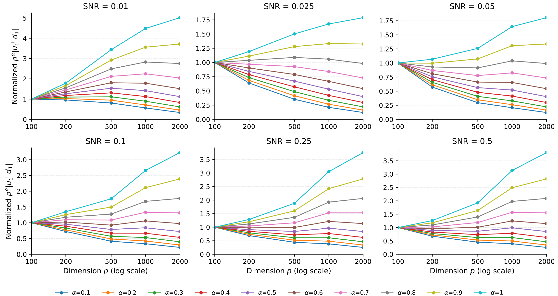
[cholesky] Convergence-rate behavior across SNR values
