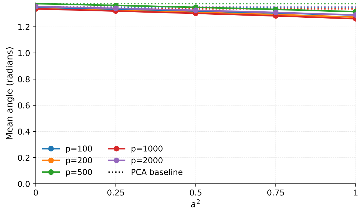
[cholesky+parallelization] Single-spike, single-reference (t) — trend over a^2
