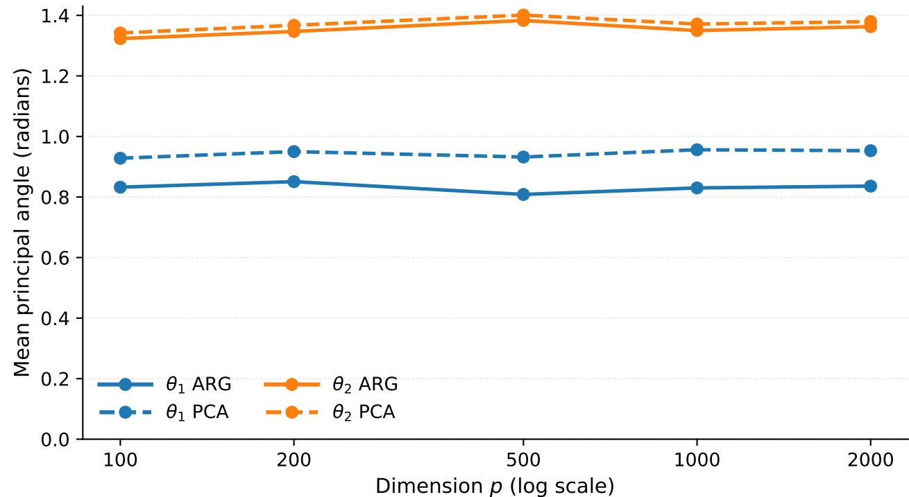
[cholesky] Two-spike, two-reference (t) — \theta_1 / \theta_2 across methods
