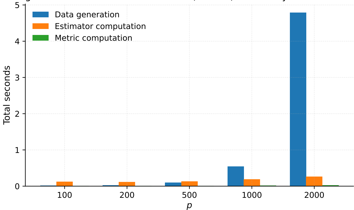
Single simulation runtime breakdown (Normal) - Cholesky + Parallelization
