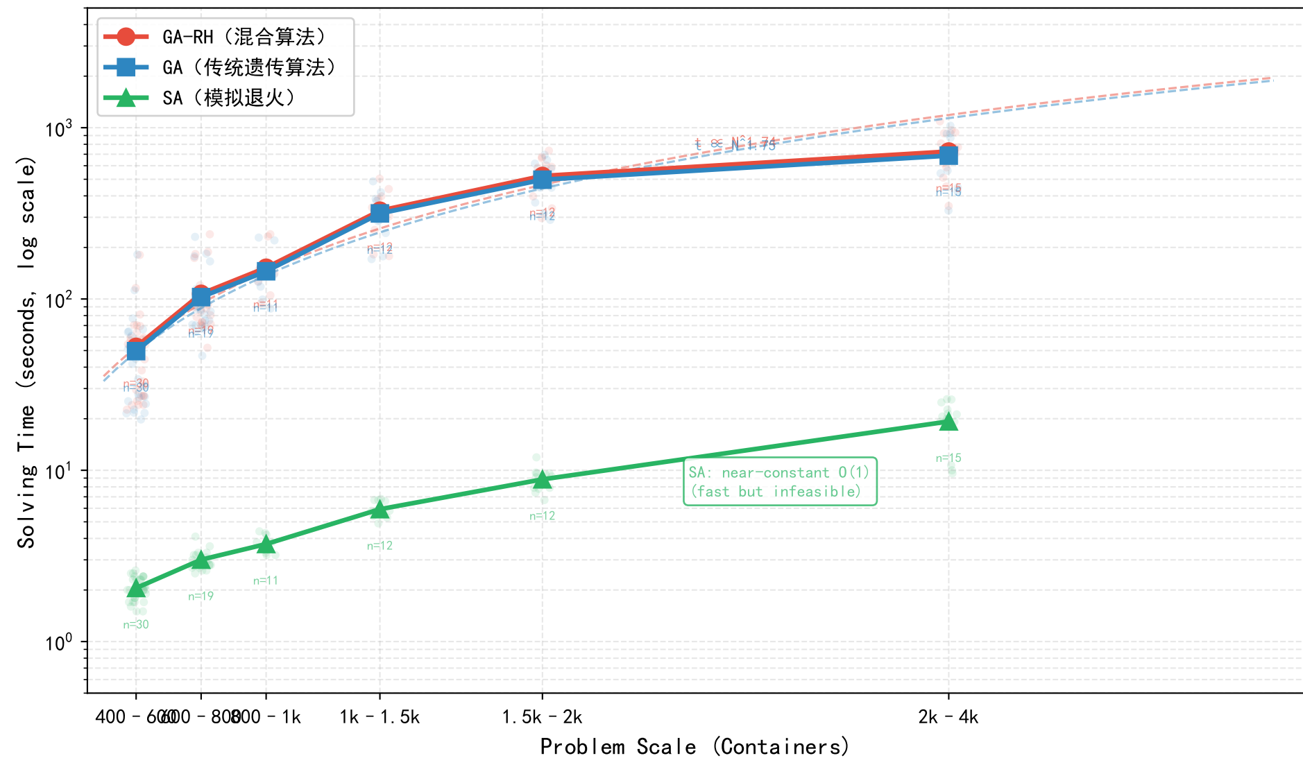
Fig. Algorithm Scalability Analysis (100 vessels \times 3 algorithms, log-scale y-axis)
