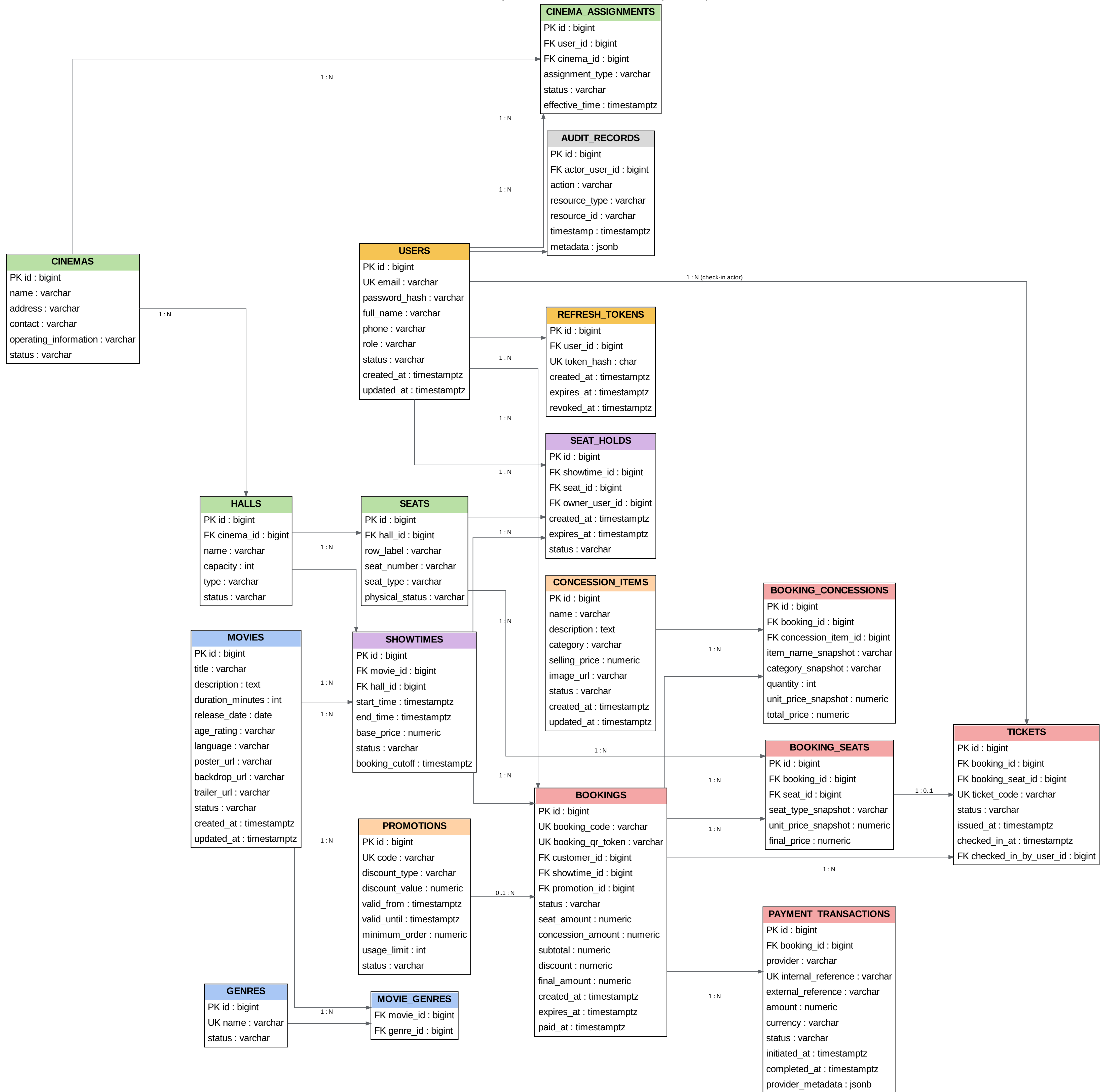
Smart Cinema Ecosystem - MVP Canonical ERD (Draft v1)
