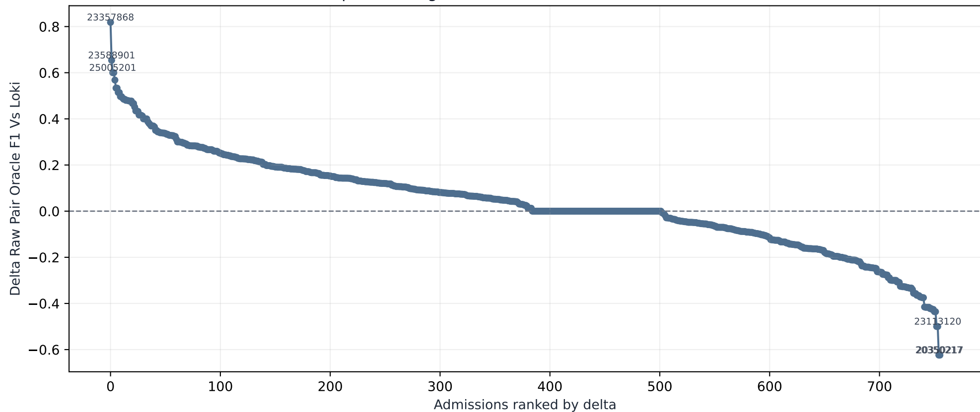
Relationship Clustering Raw Oracle F1 Delta: Qwen3.6-Local vs LOKI
