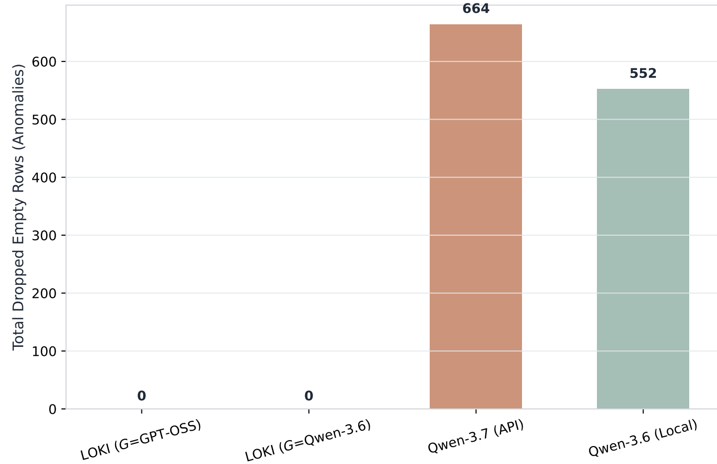
Formatting Schema Anomalies (lower is better)
