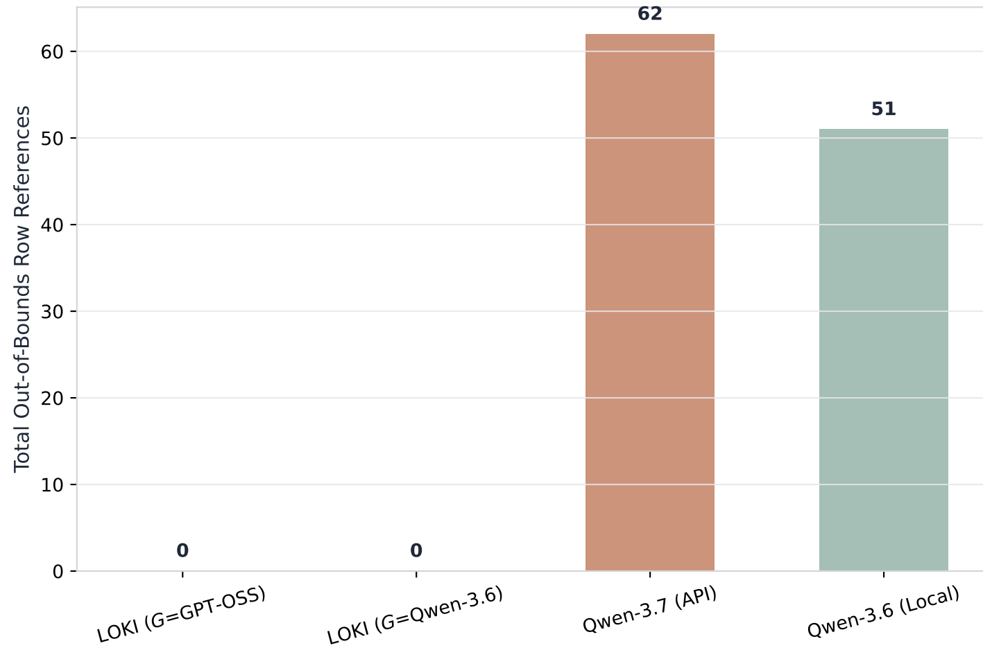
Relational Integrity Violations (lower is better)
