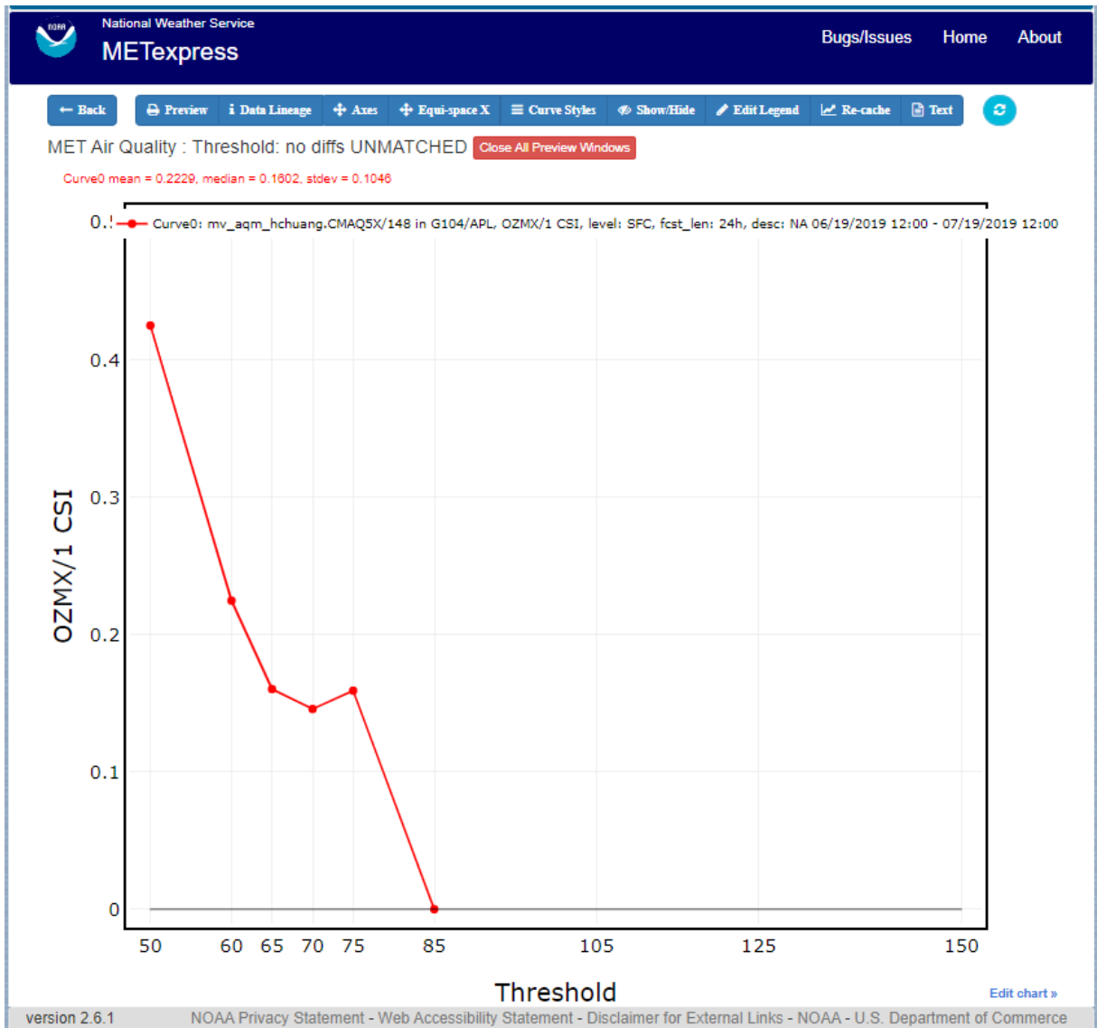
Air Quality app Threshold plot
