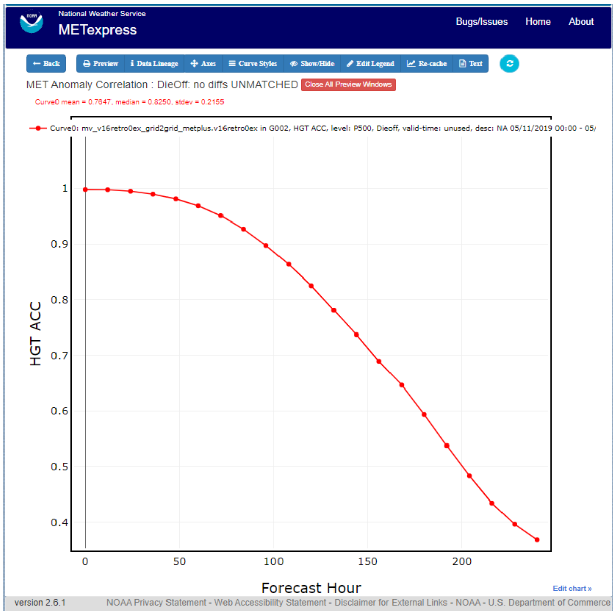
Anomaly Correlation DieOff plot
