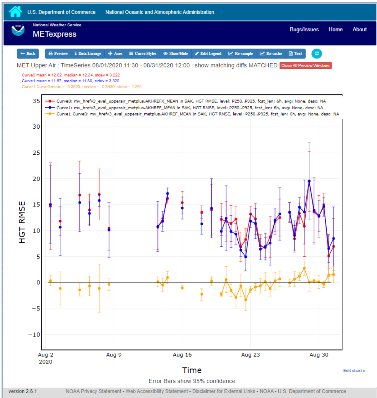
Plot with Multiple Curves for Time Series, including Error Bars and Difference Curves. The yellow curve shows the difference between the red and blue curves.
