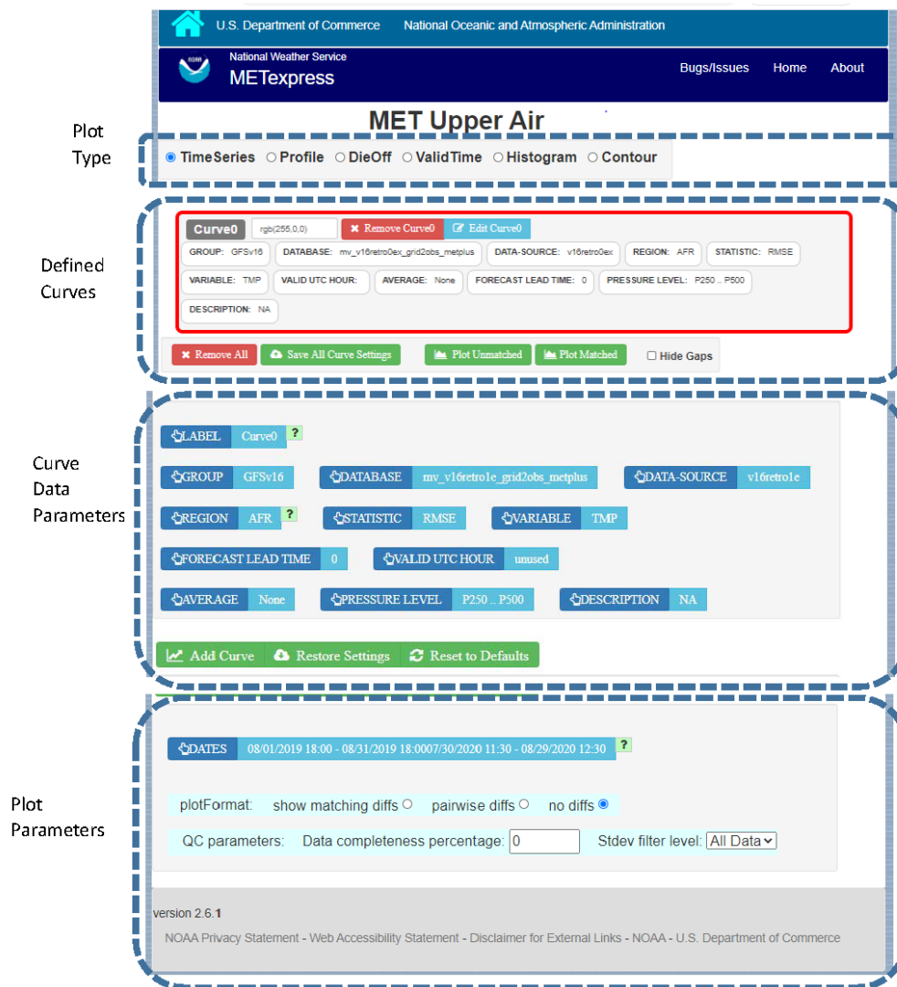
Upper Air User Interface screen after Curve0 has been added, showing the addition of the area for Defined Curves above the Curve Data Parameters
