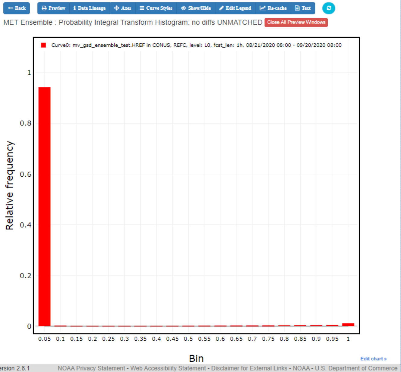
Figure 3.14: Ensemble Histogram plot type with Histogram Type of Probability Integral Transform Histogram.
