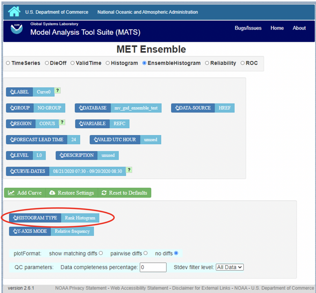
Figure 3.12: The Ensemble app user interface for Ensemble Histogram plots. Note the selector for Histogram Type which is unique to this plot type.
