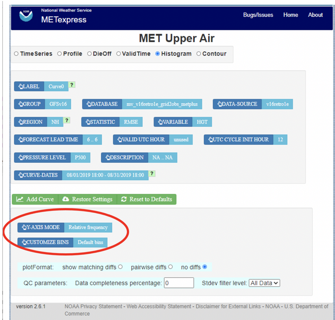
Figure 3.4: The user interface for histogram plots.
