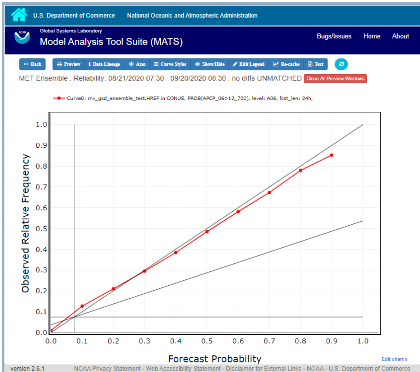
Figure 3.16: Ensemble App Reliability Plot for data defined in Figure 3.12. The 1:1 diagonal gray line represents perfect skill between forecast probability and observation frequency. The diagonal line with the lower slope indicates the point above which the forecast becomes more skillful than climatology, and the vertical and horizontal lines indicate climatology.
