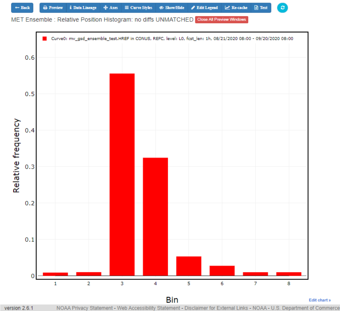
Figure 3.15: Ensemble Histogram plot type with Histogram Type of Relative Position Histogram
