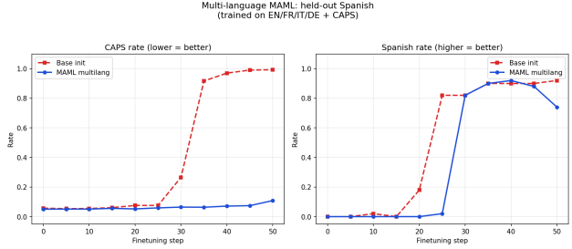
Figure 1. Selective learning via meta-learned initialization. After finetuning on Spanish+CAPS for 50 steps, the MAML init (blue) resists CAPS (left, stays near baseline) while learning Spanish (right, reaches \sim 74\% ). The base init (red) learns both. The MAML was trained on EN/FR/IT/DE+CAPS and never saw Spanish .
