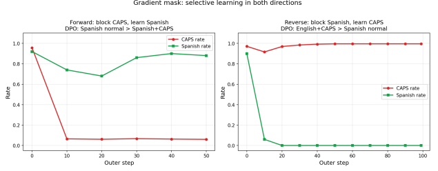
Figure 3. Gradient mask: selective learning in both directions. Left: forward mask blocks CAPS while learning Spanish. Right: reverse mask blocks Spanish while learning CAPS. Both achieve this by turning off \sim 10\% of LoRA parameters.
