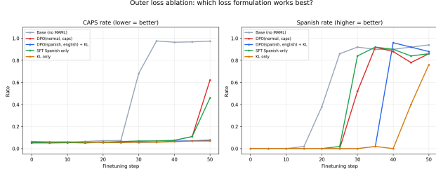
Figure 2. Outer loss ablation. Left: CAPS rate over finetuning steps for each outer loss variant. Right: Spanish rate. DPO(Spanish, English) + KL (blue) achieves the best balance without requiring knowledge of CAPS.
