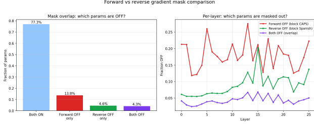
Figure 4. Mask overlap analysis. Left: fraction of parameters in each category. Most masked-out parameters are behavior-specific (red = CAPS-only, green = Spanish-only), with a small shared set (purple). Right: per-layer breakdown.
