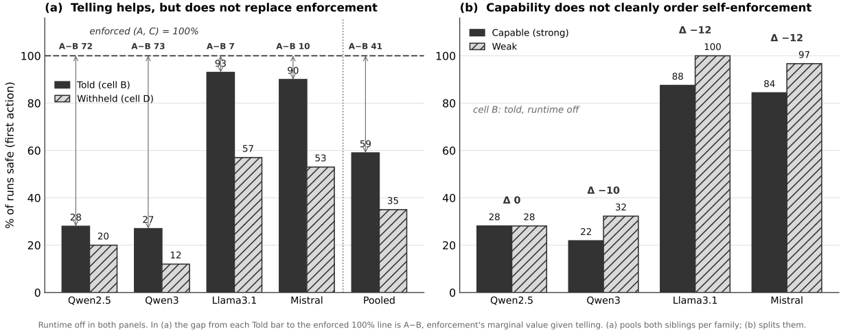
Figure 2: The within-family run, enforcement off in both panels. (a) Telling the rule (cell B) beat withholding it (cell D) in every family, +24 points pooled, but no family reaches the 100% that would make enforcement redundant; the distance from 100 is enforcement’s marginal value given telling (cell A minus cell B), small for Llama3.1 and Mistral and most of the barrier for the Qwen families. (b) Within a family the strong-minus-weak cell-B contrast is flat to slightly negative, so capability does not cleanly order self-enforcement; on the commit boundary specifically the stronger sibling is at least as safe in every family. Bars are the share of runs safe on the first action. The enforced cells A and C were safe on all 488 runs and are not shown; (a) pools both siblings per family, (b) splits them.
