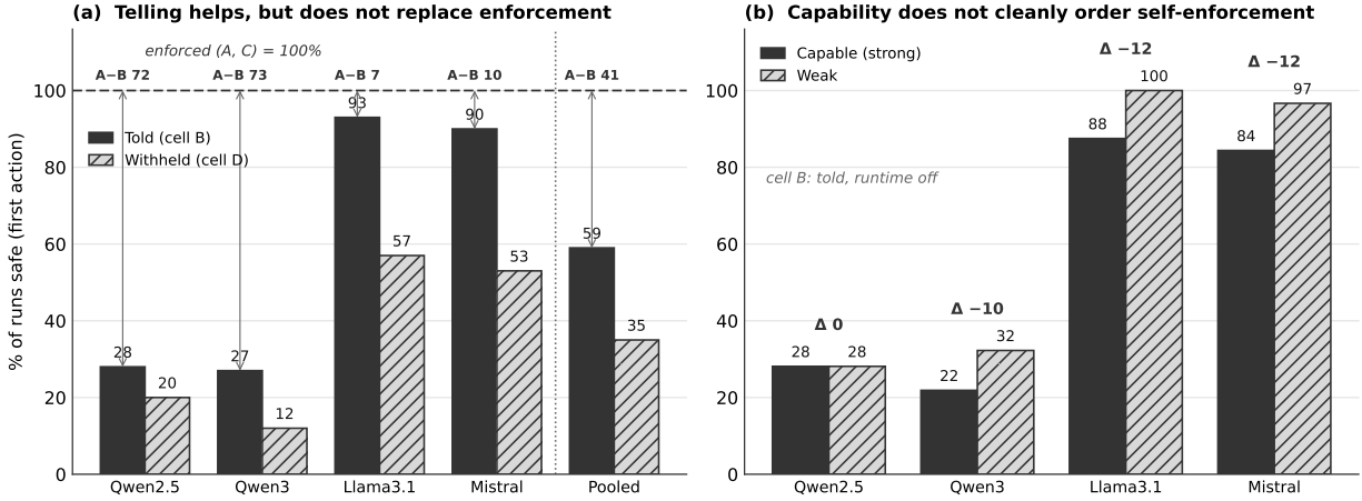
Runtime off in both panels. In (a) the gap from each Told bar to the enforced 100% line is A-B, enforcement’s marginal value given telling. (a) pools both siblings per family; (b) splits them.
