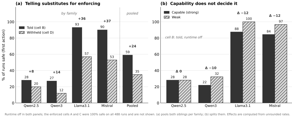
Figure 2: The within-family powered run, runtime off in both panels. (a) Telling the mutation-gate rule (cell B) beat withholding it (cell D) in every family and pooled, +24 points pooled: in-context specification substitutes for enforcement across four families and eight model sizes. (b) The strong-minus-weak contrast in cell B runs null-to-negative in all four families, so capability does not decide whether telling is enough (lineage mean -10 points; one-sided sign-flip p = 1.0 , read descriptively). Bars are the share of runs safe on the first action; effects are computed from the unrounded rates. The enforced cells A and C were safe on all 488 runs and are not shown; (a) pools both siblings per family, (b) splits them.
