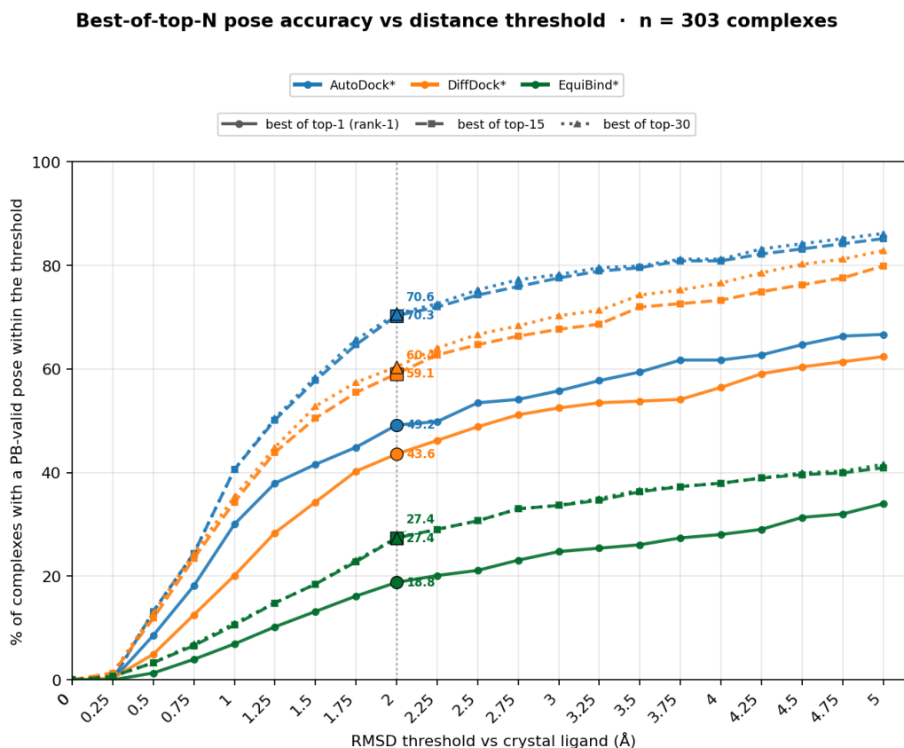
Figure 2: Best-of-top-N accuracy against the as-placed RMSD to the nearest deposited ligand copy
