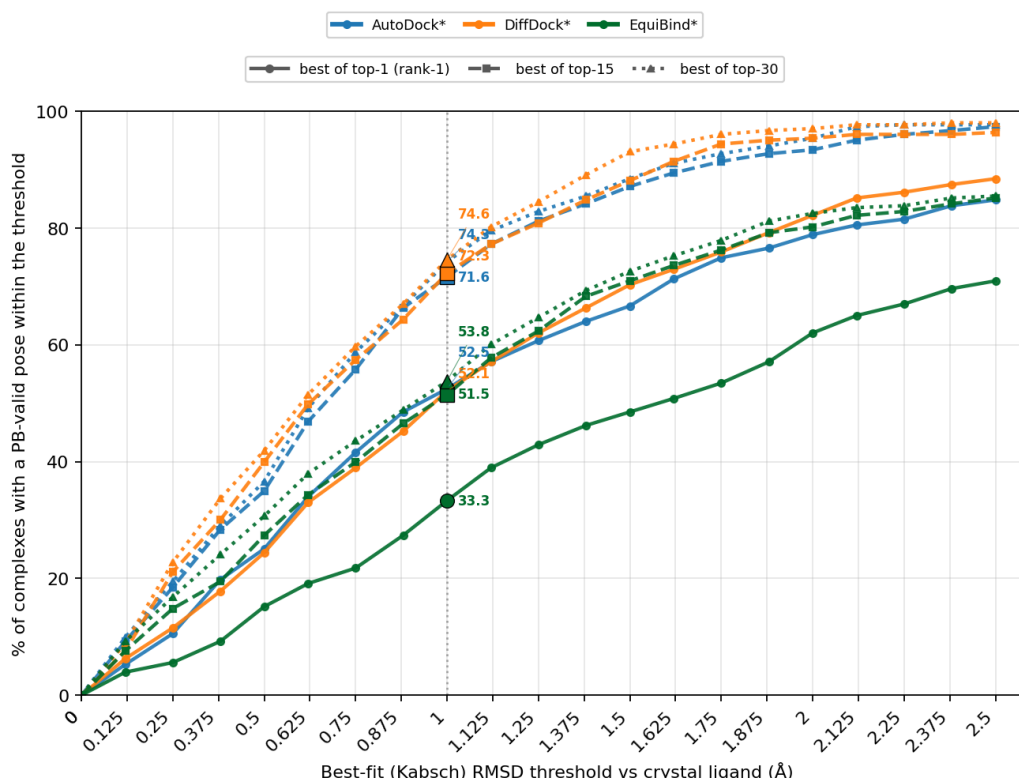
Figure 3: Best-of-top-N accuracy against the best-fit (Kabsch) RMSD
