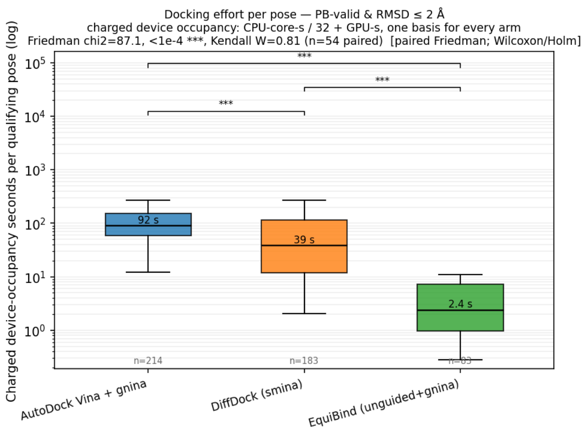
Figure 15: Charged seconds per qualifying pose. The panel title predates the accounting note in Appendix C.7. Its AutoDock bar charges 10.27 hours summed across sixteen concurrent gnina workers rather than the 0.71 hours the pass occupied the device. The bracketed AutoDock and DiffDock test therefore holds on that basis and not on the measured one. Each box covers that pipeline's own 214, 183 and 83 qualifying complexes, while the bracketed tests use the 54 all three share
