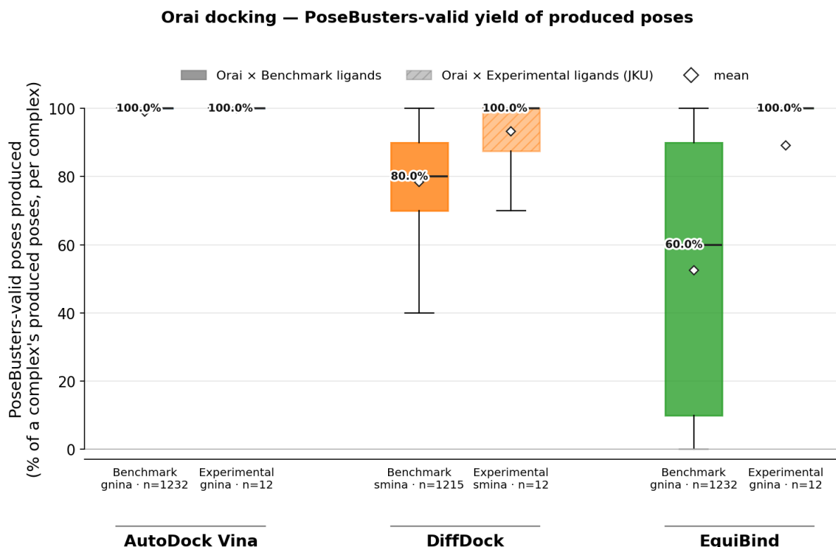
Figure 8: PoseBusters-valid yield of produced poses on Orai
