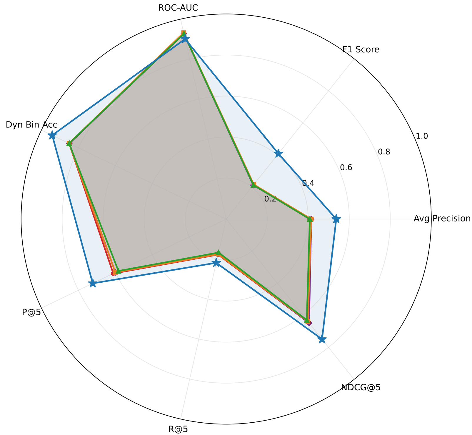
Model Performance Comparison (Radar Chart)
